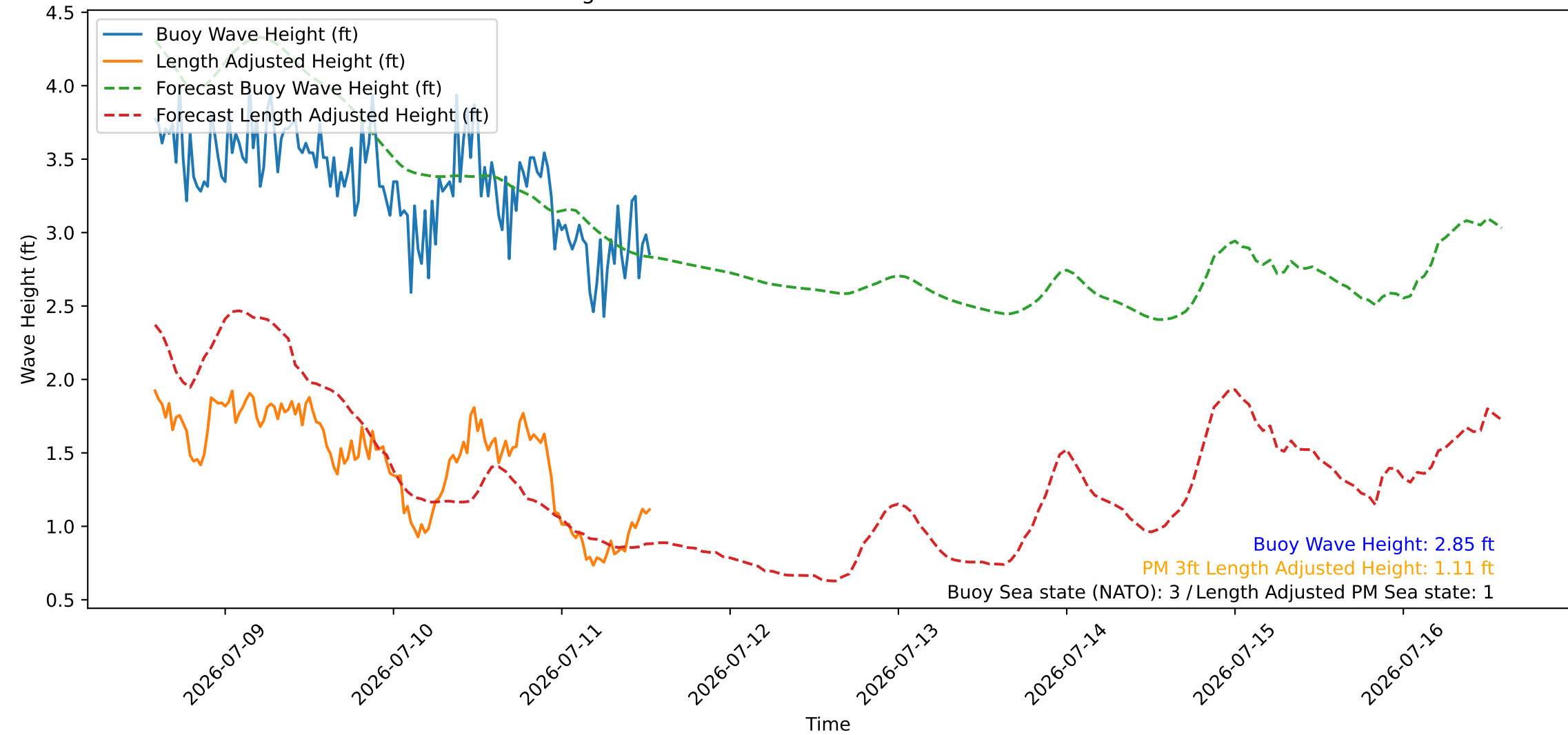
Wave Heights over Time for Red Beach at 2026-07-11 13:30:46
