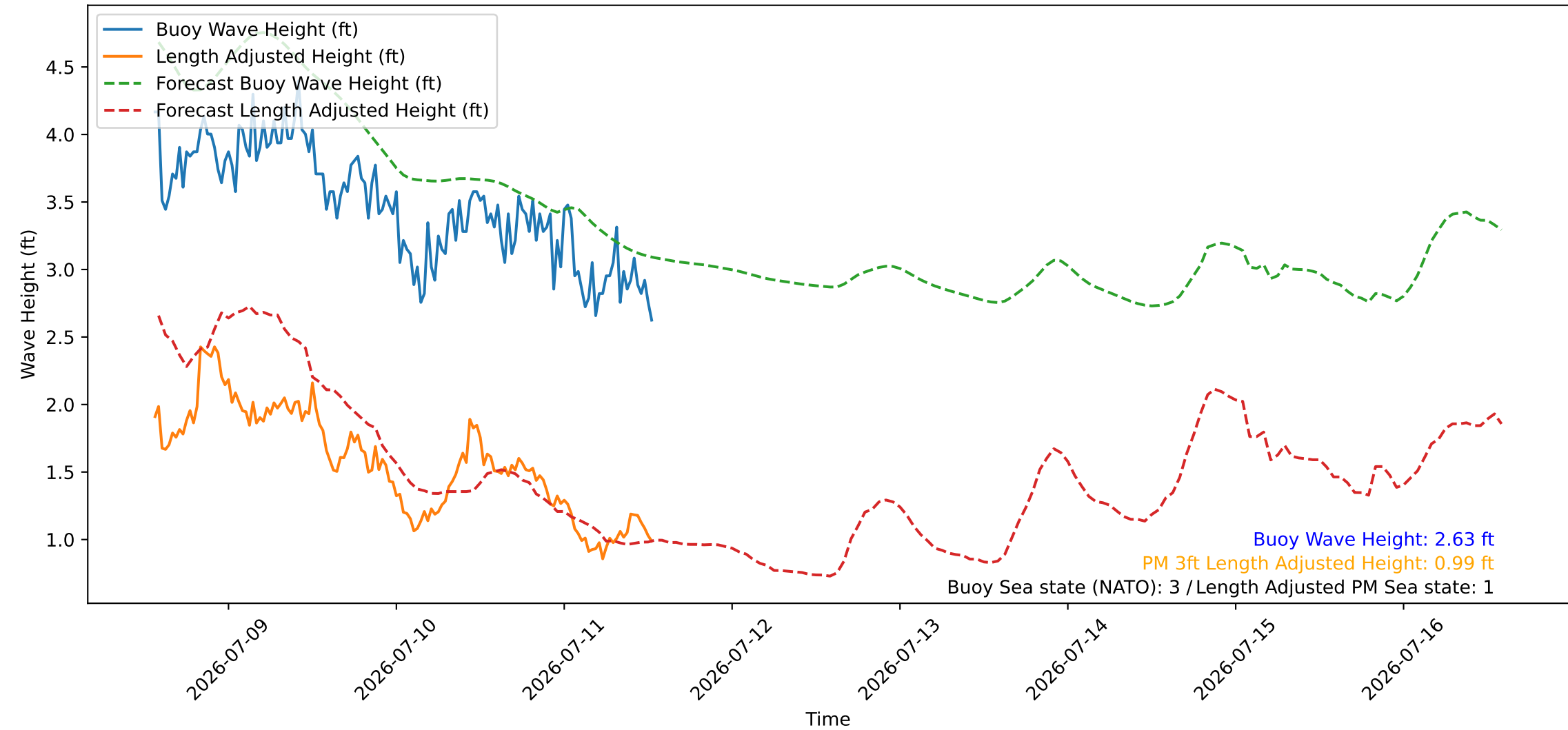
Wave Heights over Time for Green Beach at 2026-07-11 13:31:08
