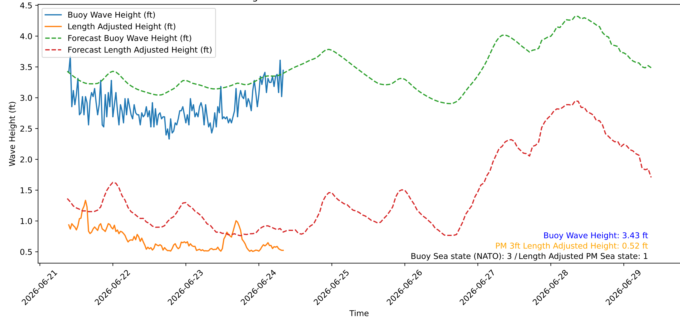
Wave Heights over Time for Red Beach at 2026-06-24 09:00:45
