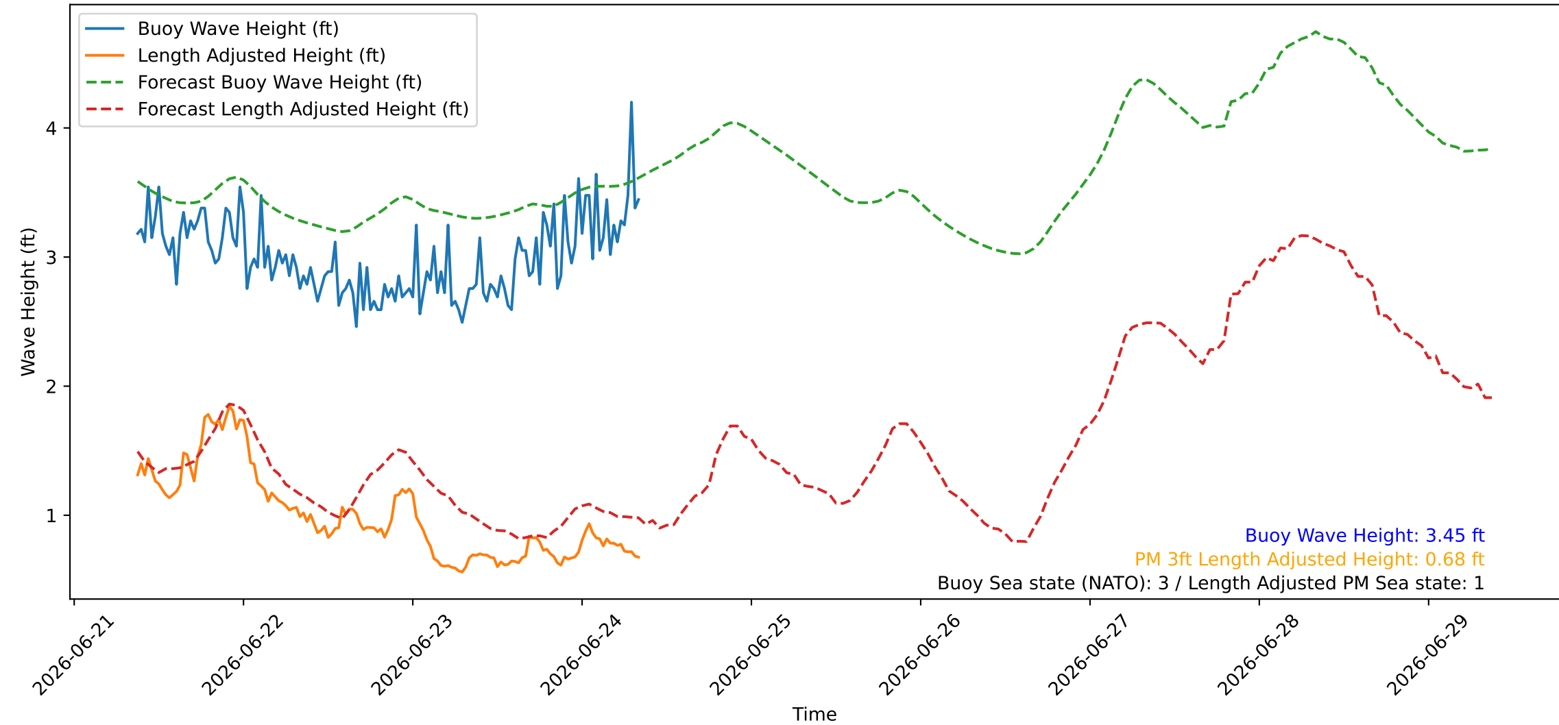
Wave Heights over Time for Green Beach at 2026-06-24 09:01:08
