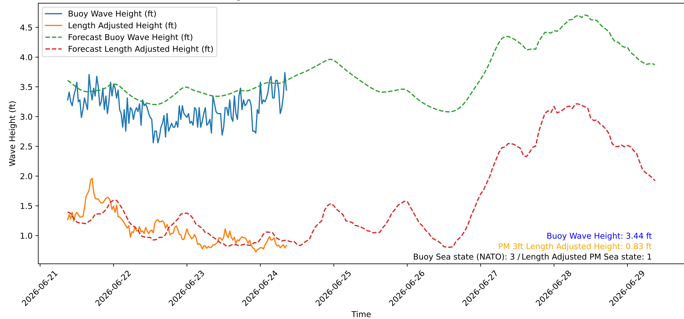
Wave Heights over Time for Oceanside Harbor at 2026-06-24 09:00:26
