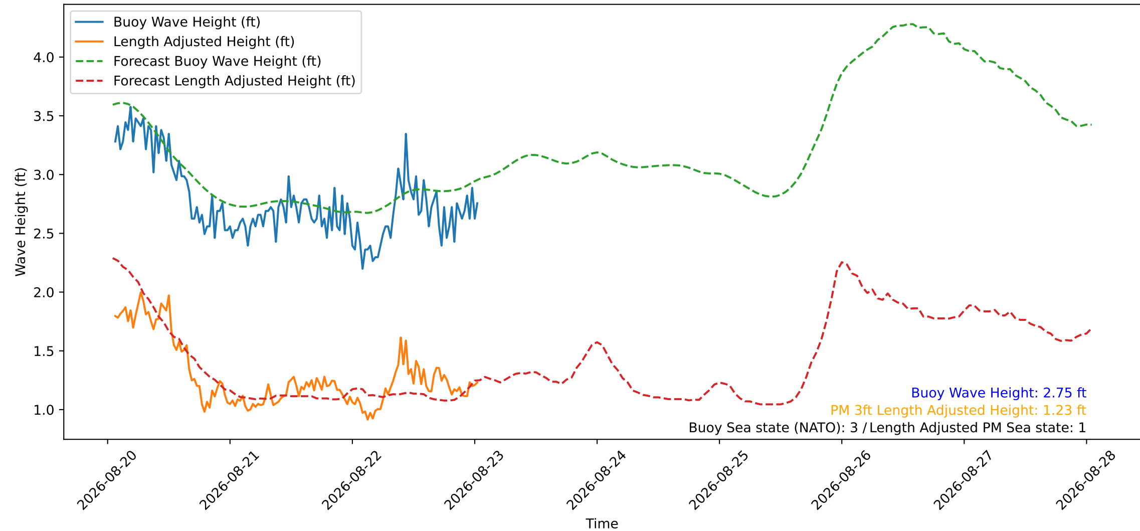
Wave Heights over Time for Oceanside Harbor at 2026-08-23 01:20:30
