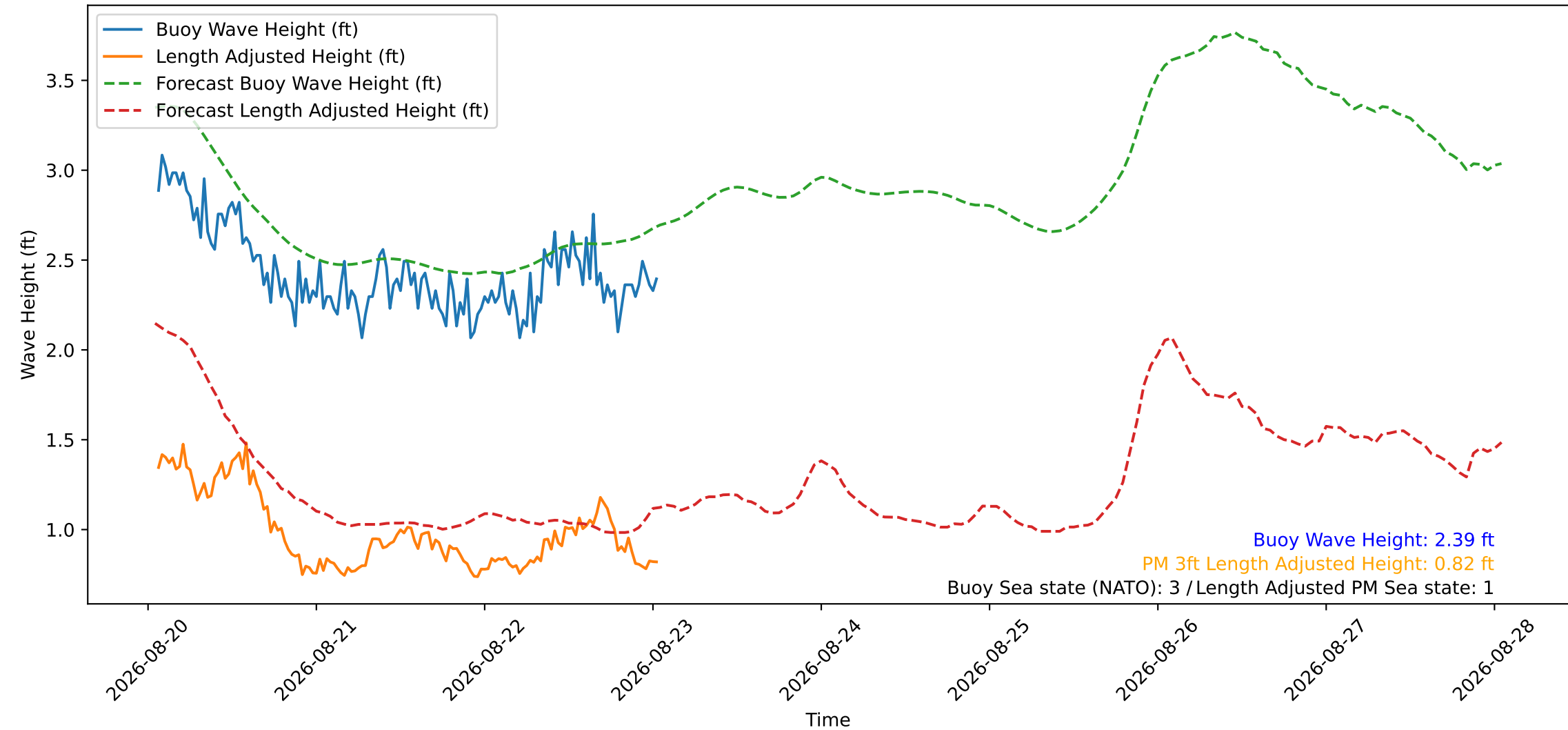
Wave Heights over Time for Red Beach at 2026-08-23 01:20:51
