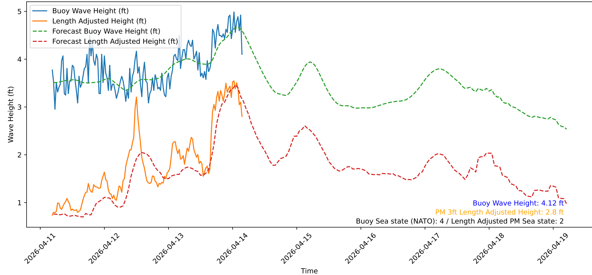
Wave Heights over Time for Green Beach at 2026-04-14 04:31:13
