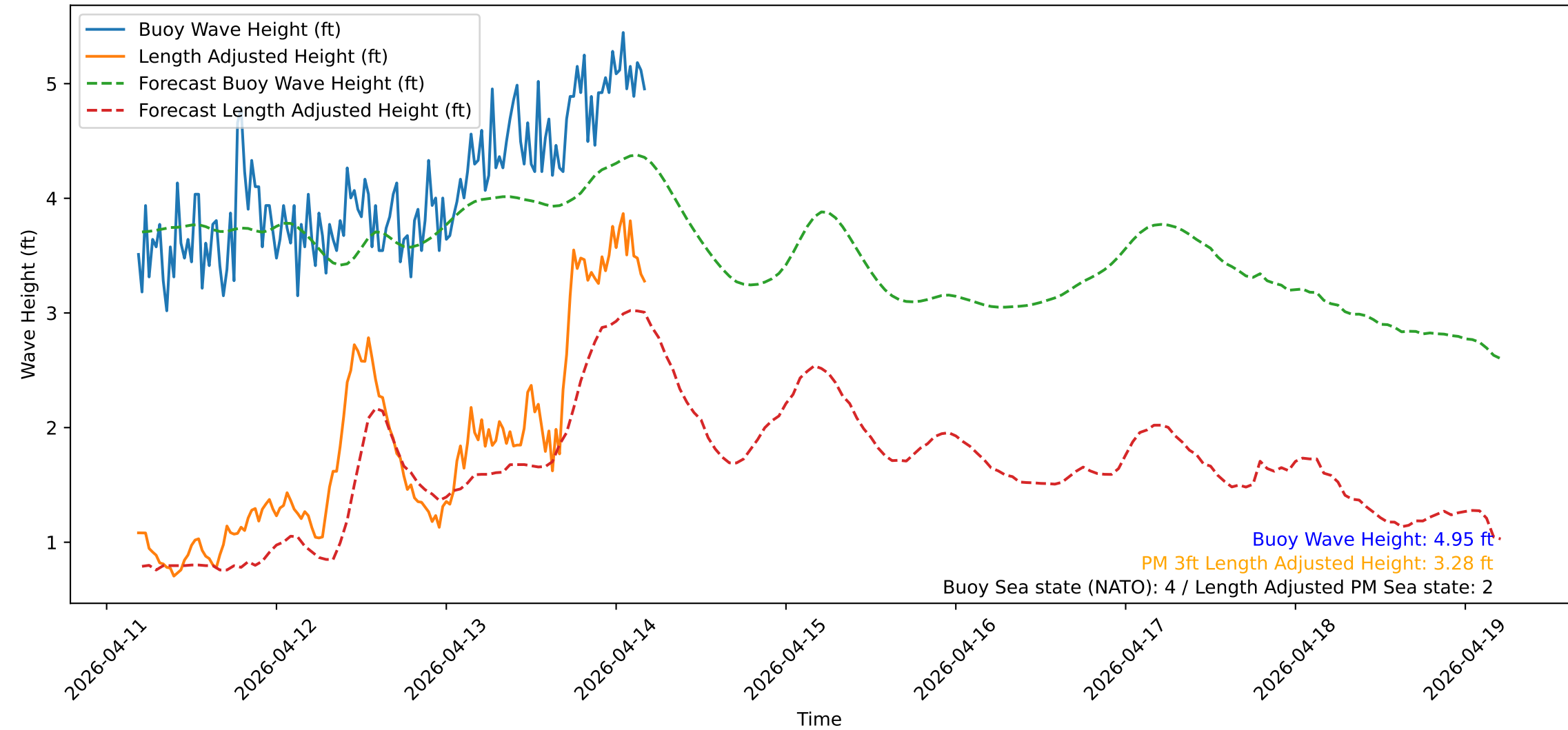
Wave Heights over Time for Oceanside Harbor at 2026-04-14 04:30:31
