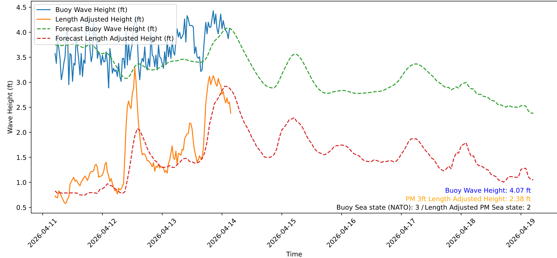
Wave Heights over Time for Red Beach at 2026-04-14 04:30:51
