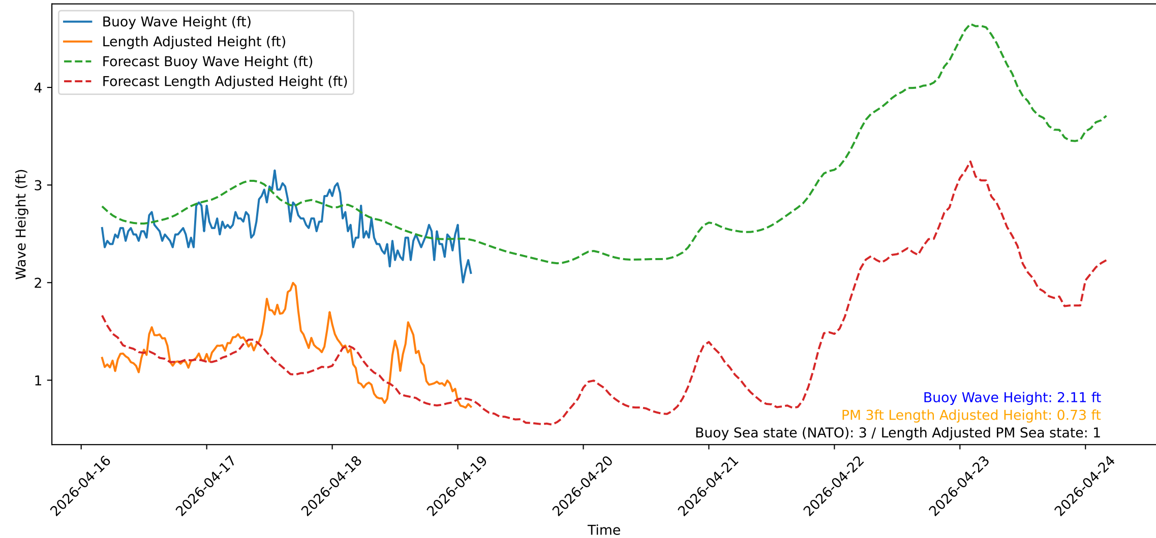
Wave Heights over Time for Red Beach at 2026-04-19 03:30:50
