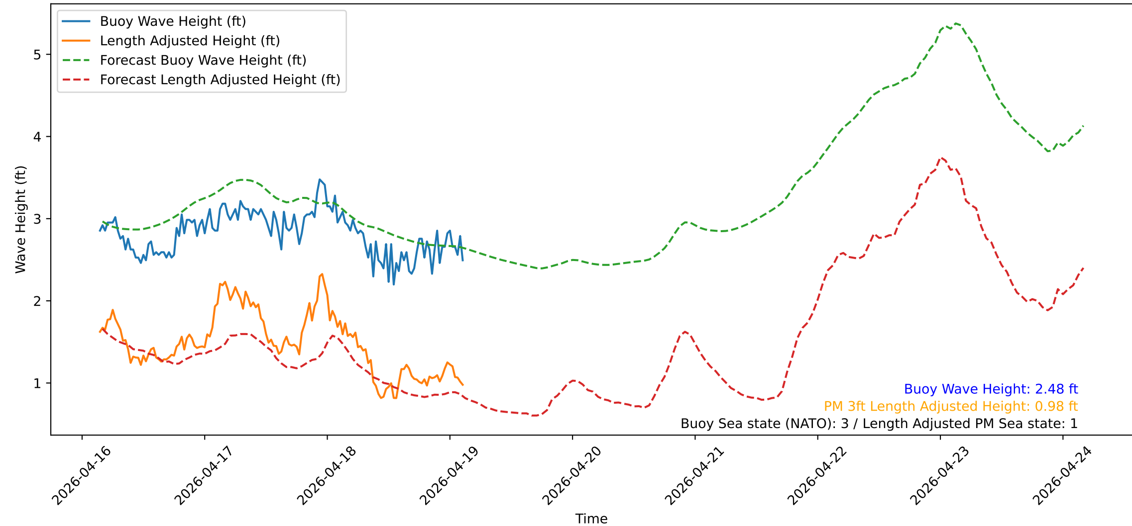
Wave Heights over Time for Green Beach at 2026-04-19 03:31:13
