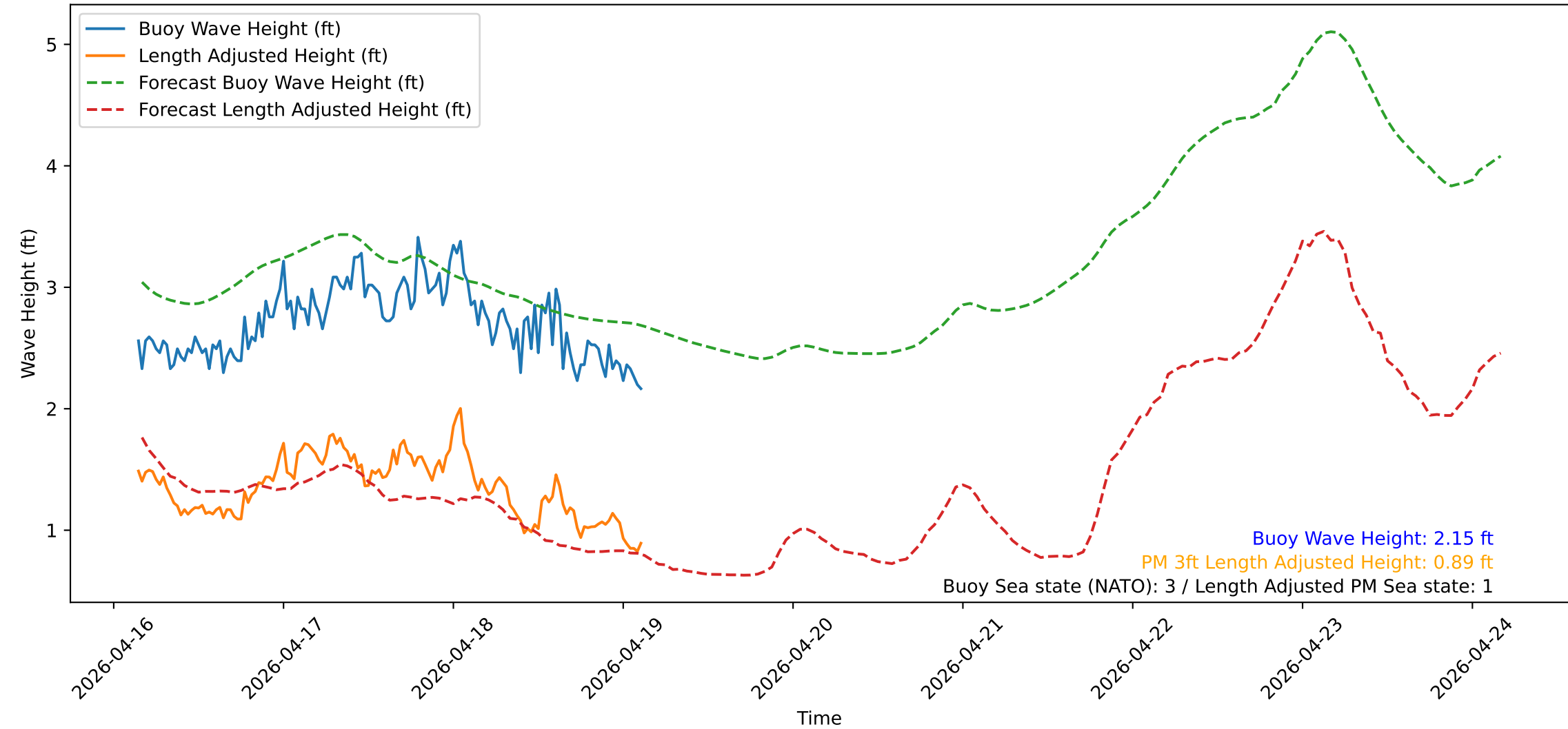
Wave Heights over Time for Oceanside Harbor at 2026-04-19 03:30:31
