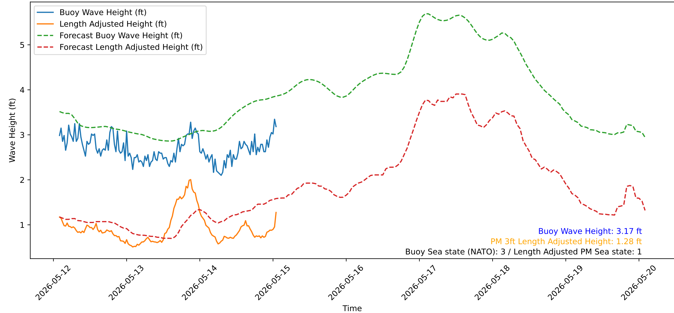
Wave Heights over Time for Green Beach at 2026-05-15 01:51:14
