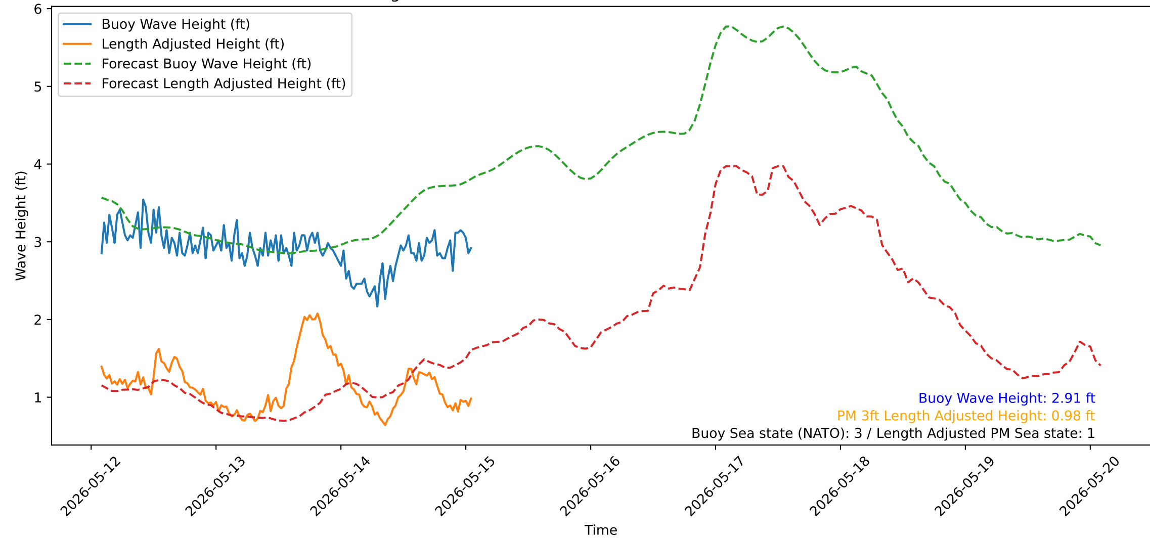
Wave Heights over Time for Oceanside Harbor at 2026-05-15 01:50:31
