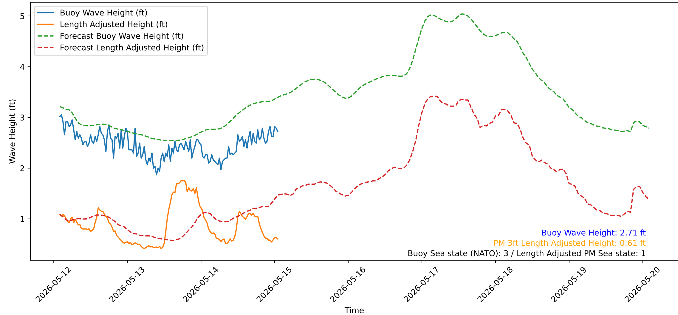
Wave Heights over Time for Red Beach at 2026-05-15 01:50:51
