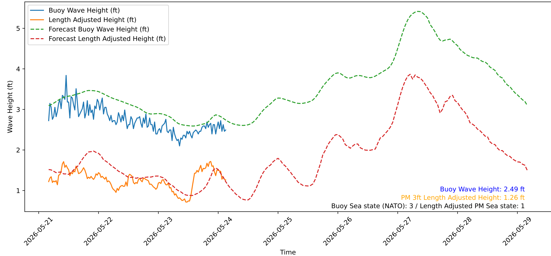
Wave Heights over Time for Oceanside Harbor at 2026-05-24 03:50:31
