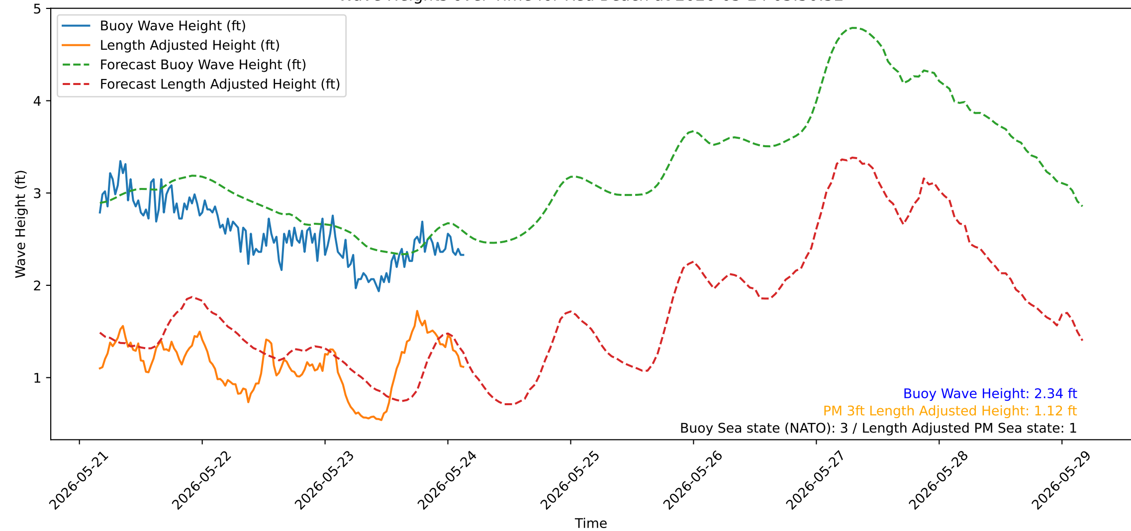
Wave Heights over Time for Red Beach at 2026-05-24 03:50:52
