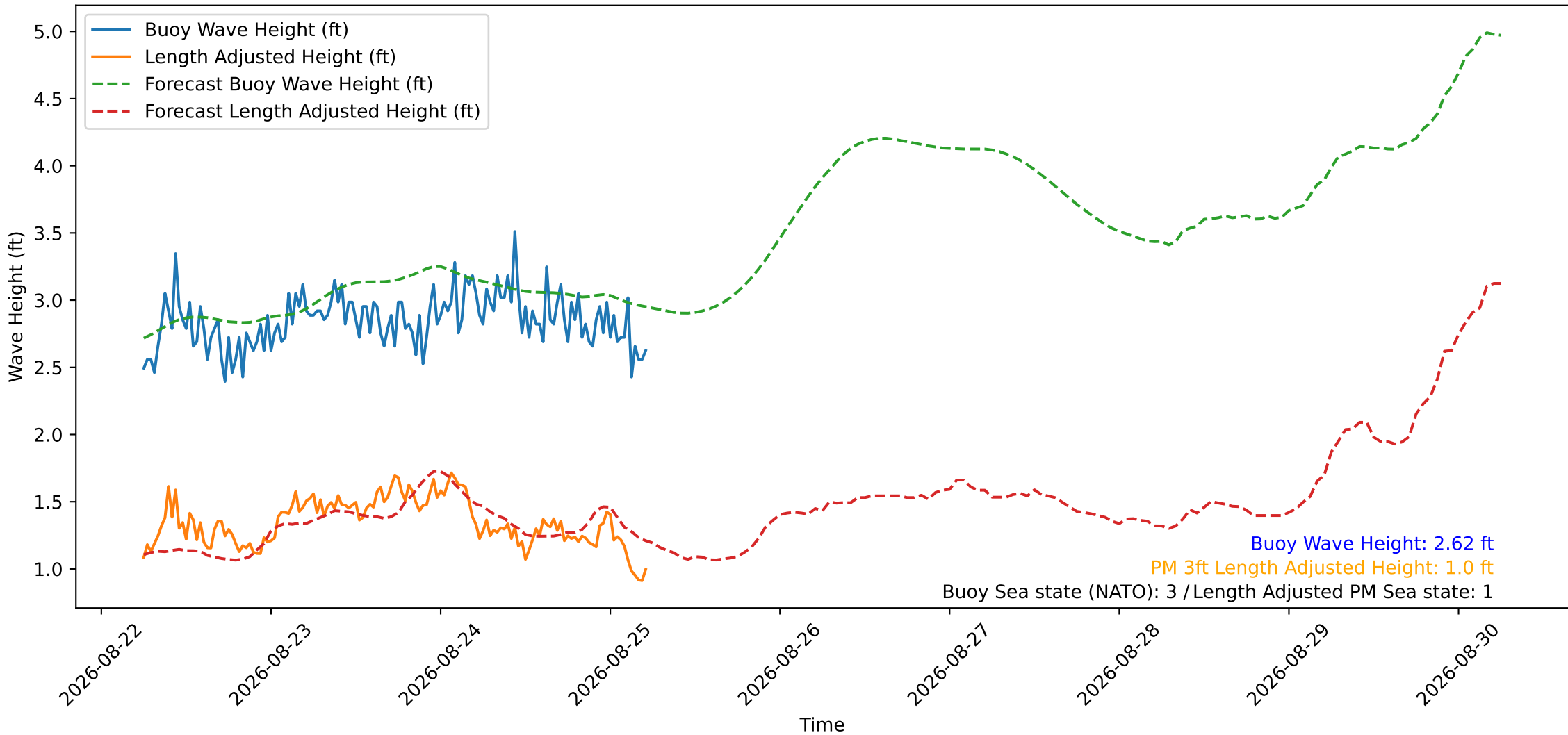
Wave Heights over Time for Oceanside Harbor at 2026-08-25 06:00:29
