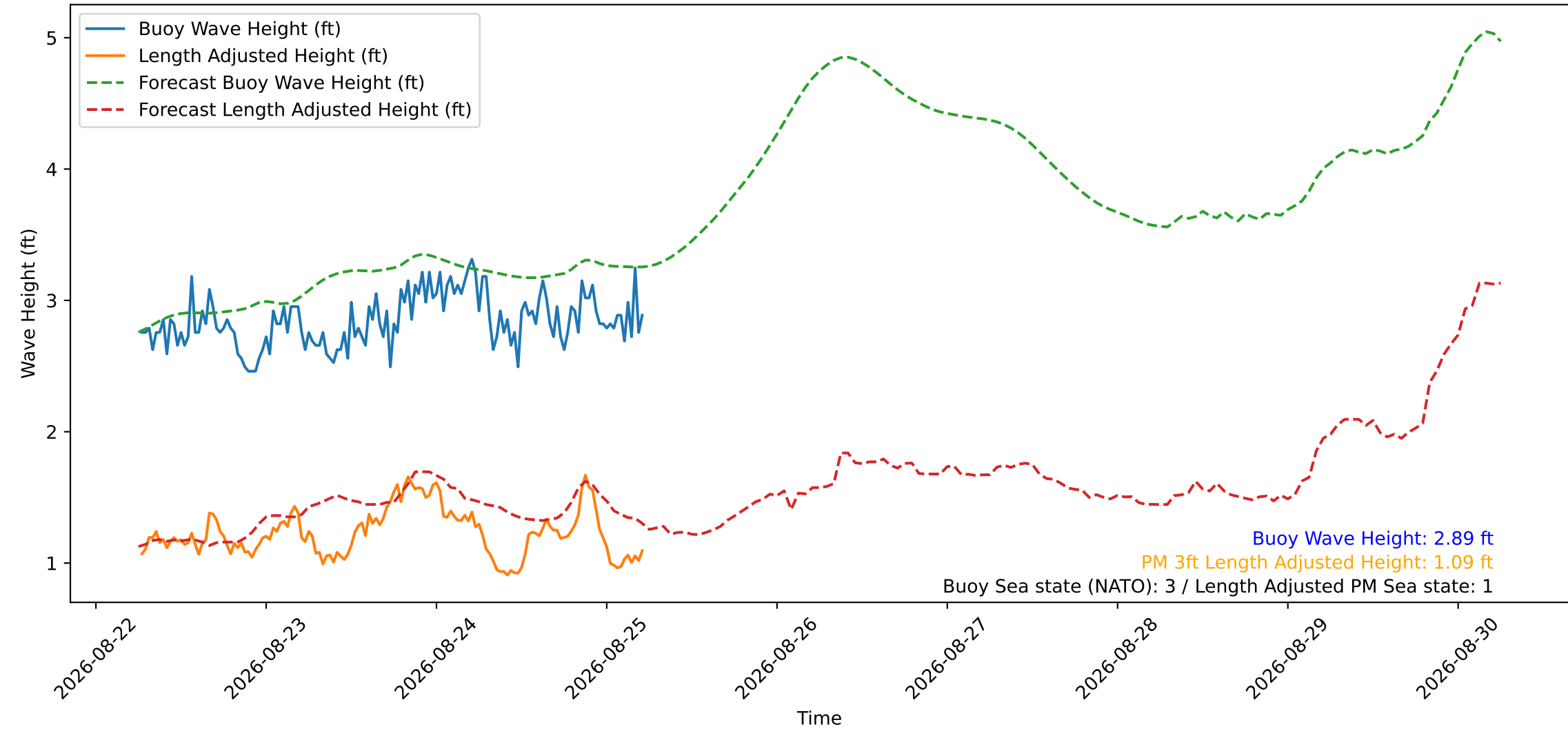
Wave Heights over Time for Green Beach at 2026-08-25 06:01:11
