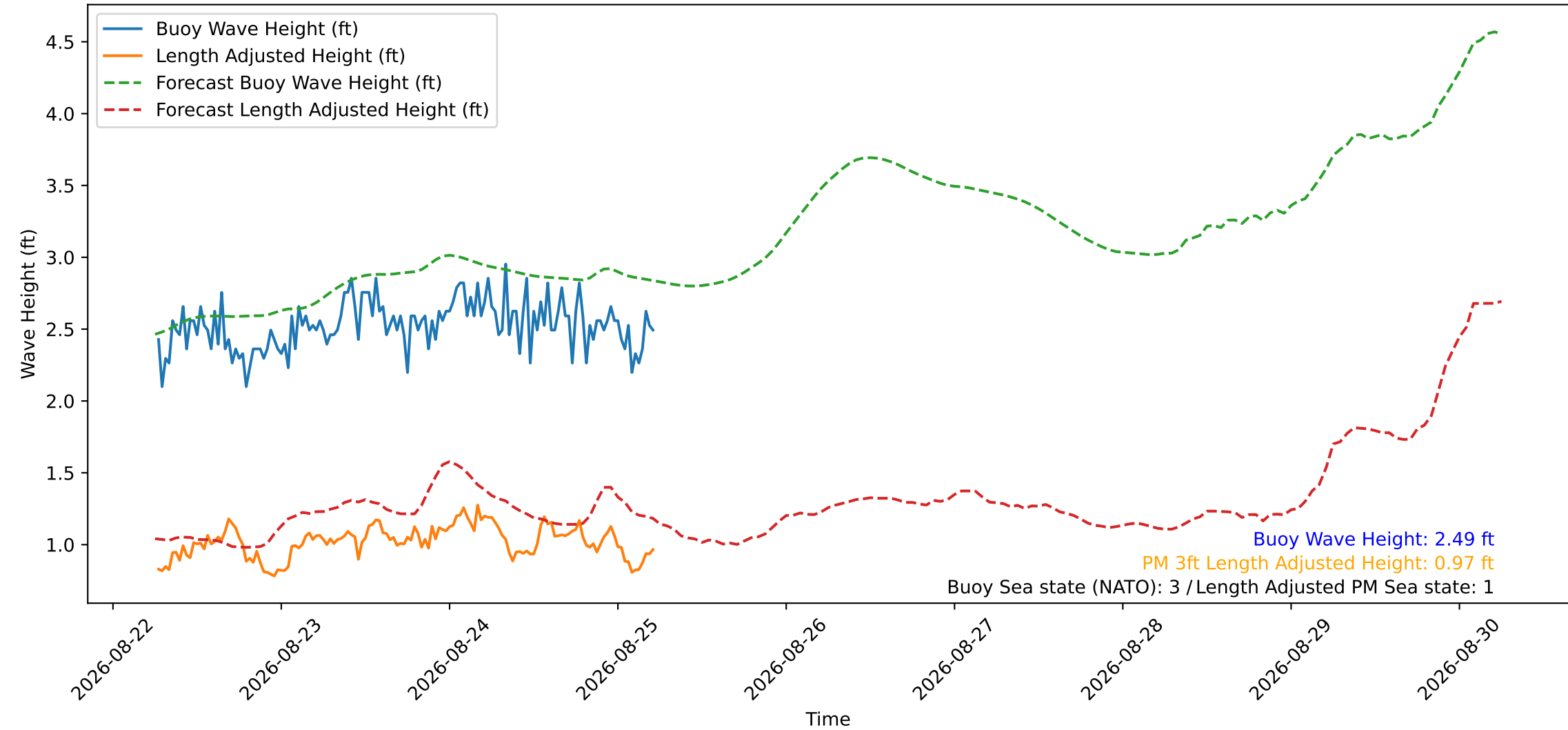
Wave Heights over Time for Red Beach at 2026-08-25 06:00:49
