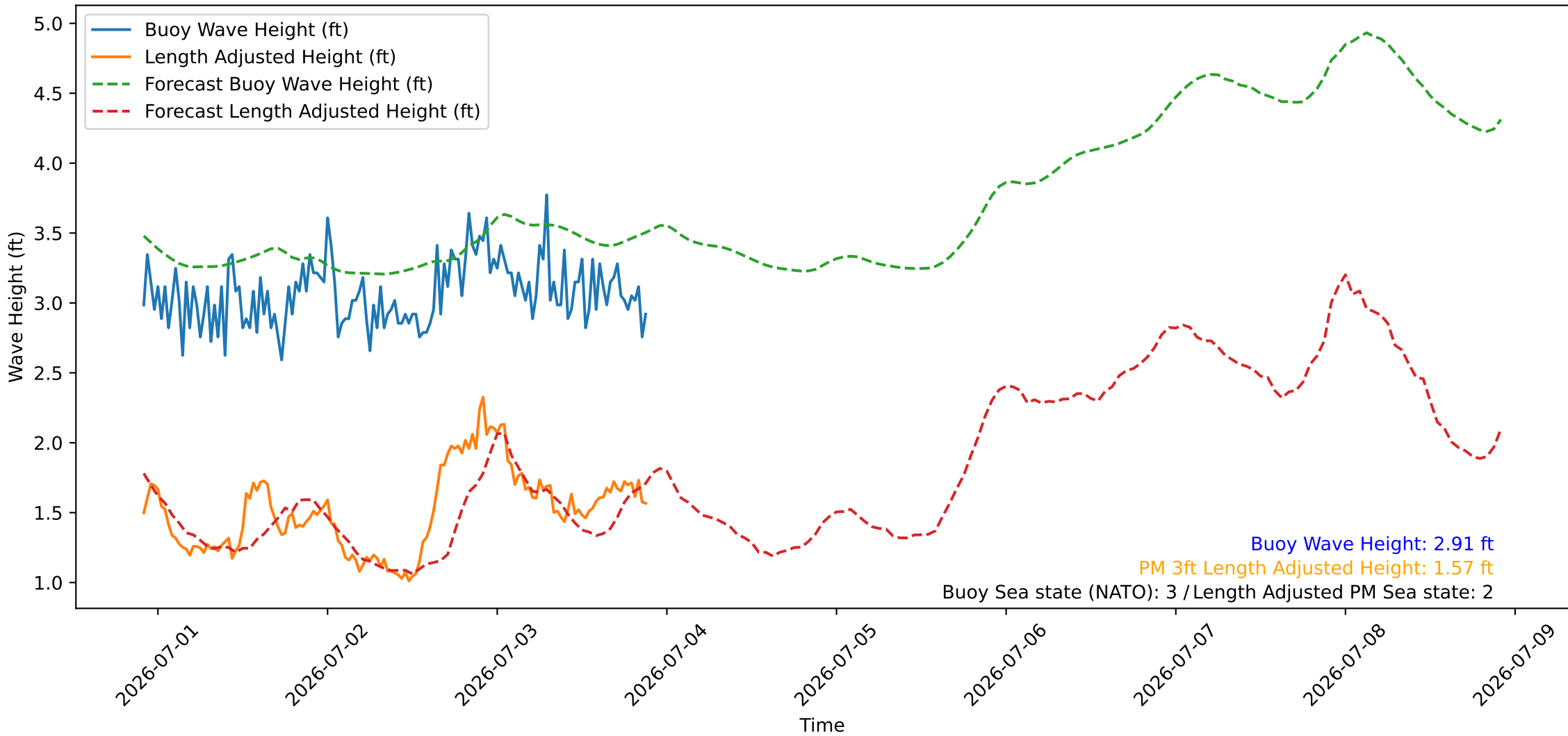
Wave Heights over Time for Oceanside Harbor at 2026-07-03 21:50:26
