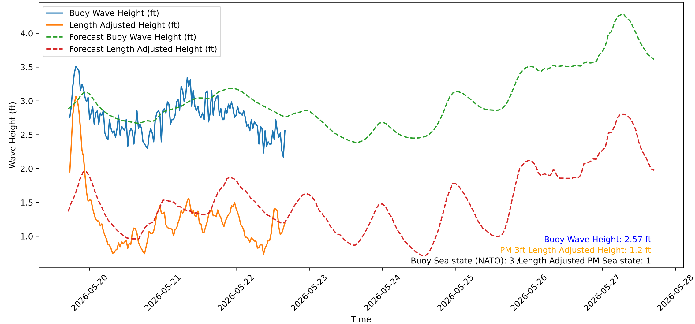
Wave Heights over Time for Red Beach at 2026-05-22 17:00:51
