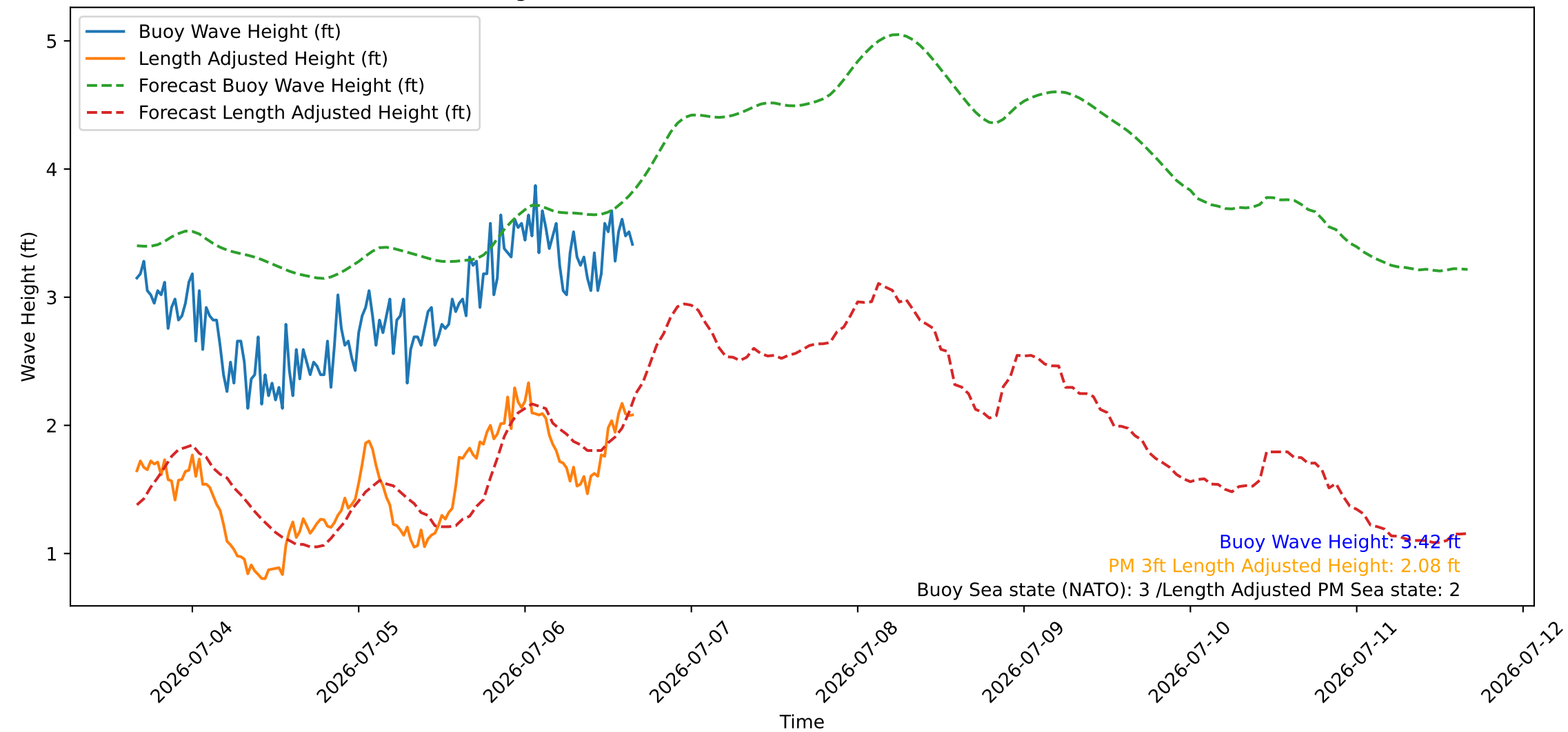
Wave Heights over Time for Oceanside Harbor at 2026-07-06 16:10:26
