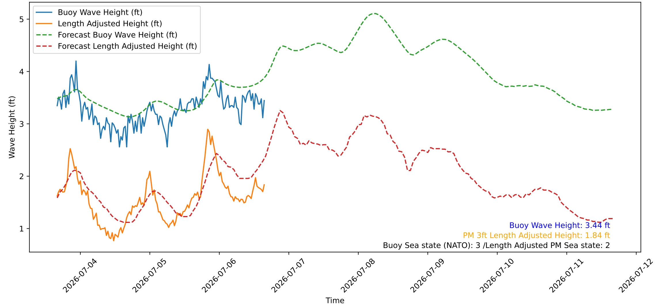
Wave Heights over Time for Green Beach at 2026-07-06 16:11:08
