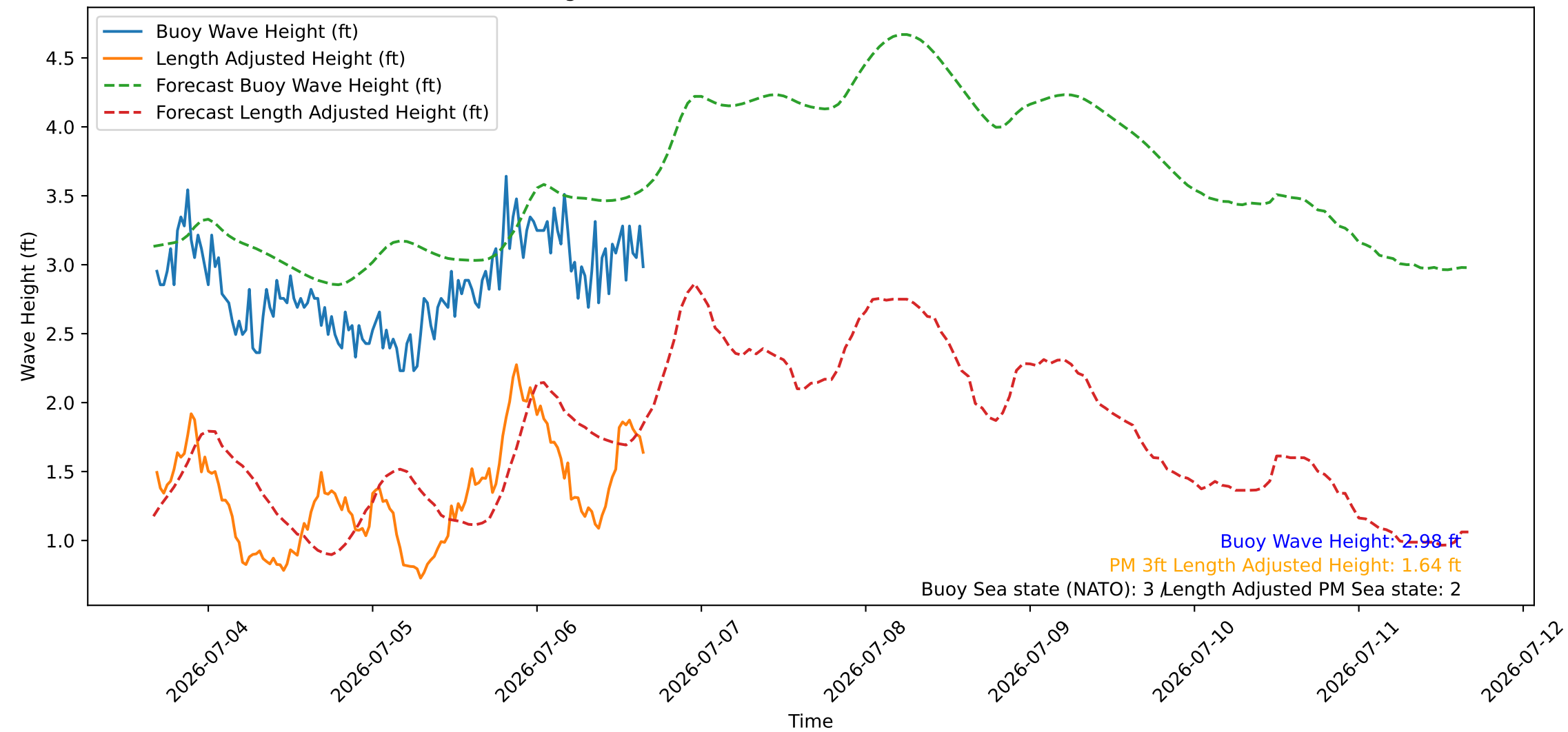
Wave Heights over Time for Red Beach at 2026-07-06 16:10:45
