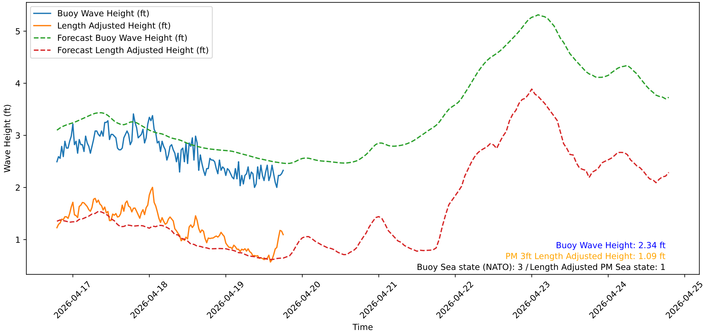
Wave Heights over Time for Oceanside Harbor at 2026-04-19 18:50:31
