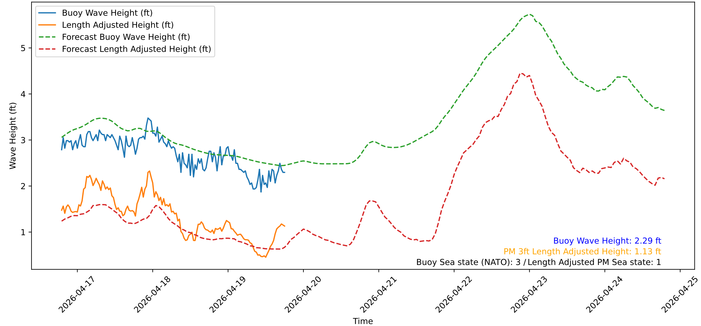
Wave Heights over Time for Green Beach at 2026-04-19 18:51:13
