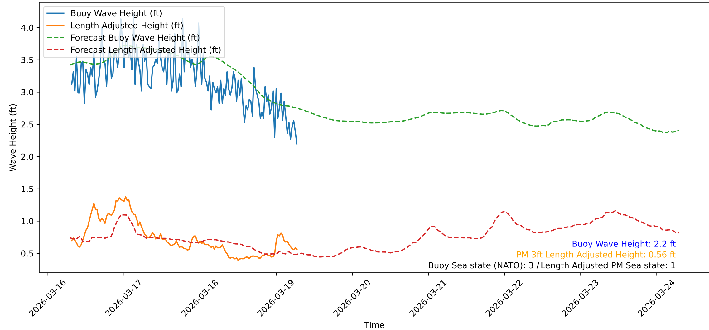
Wave Heights over Time for Green Beach at 2026-03-19 07:21:10
