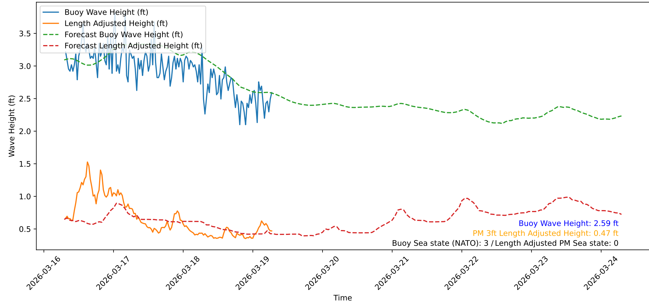
Wave Heights over Time for Red Beach at 2026-03-19 07:20:47
