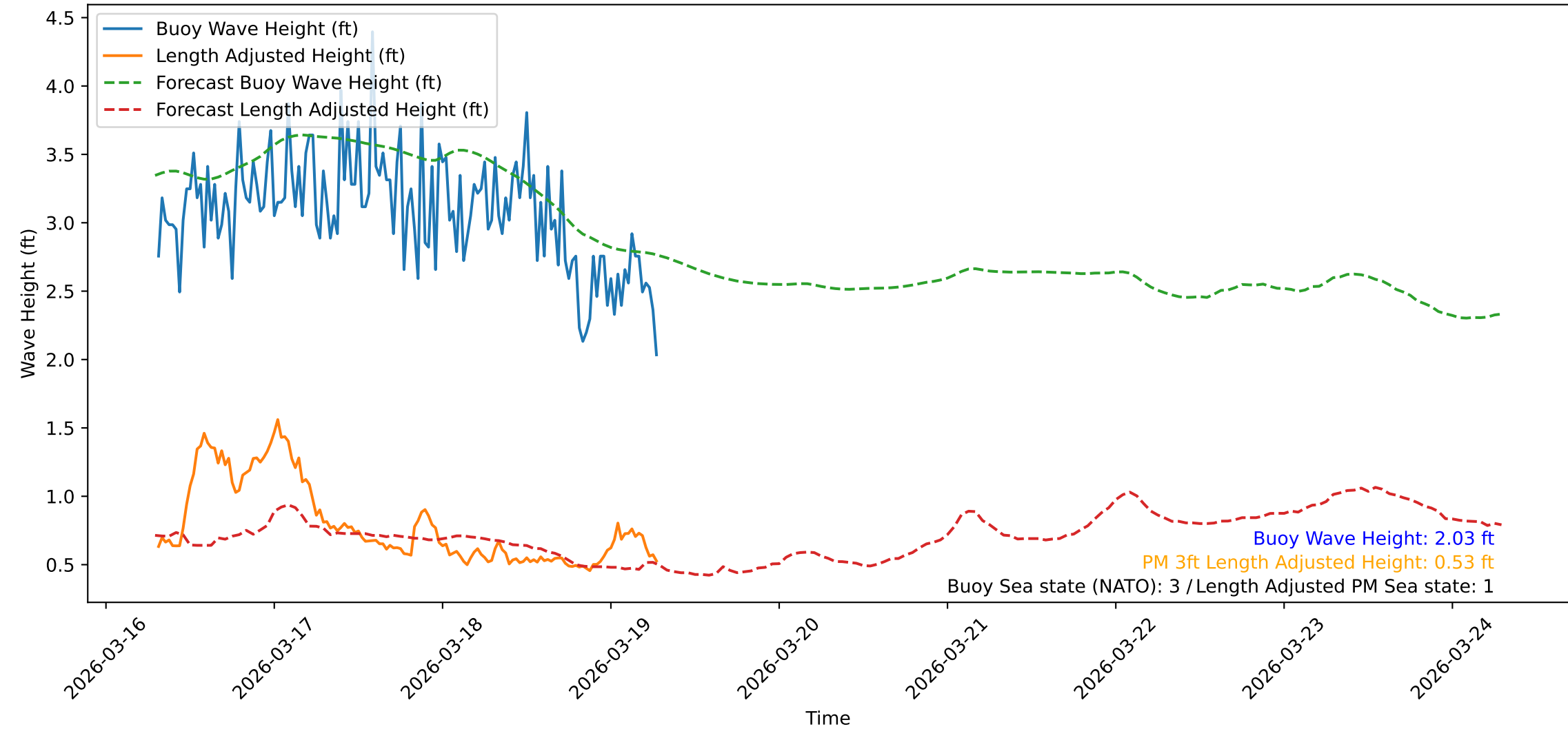
Wave Heights over Time for Oceanside Harbor at 2026-03-19 07:20:31
