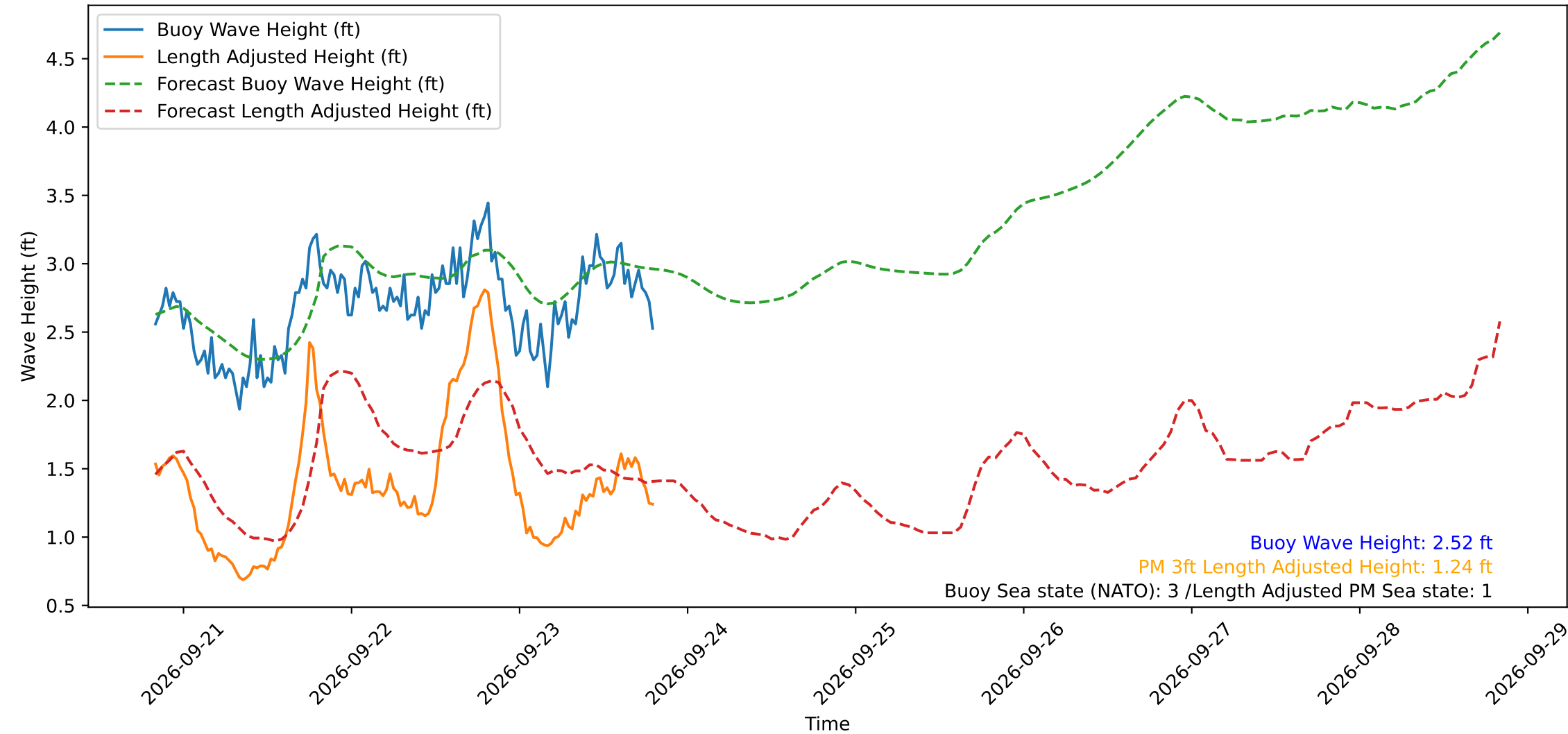
Wave Heights over Time for Green Beach at 2026-09-23 19:51:13
