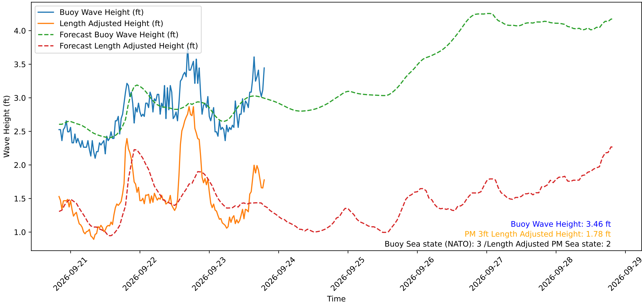
Wave Heights over Time for Oceanside Harbor at 2026-09-23 19:50:29
