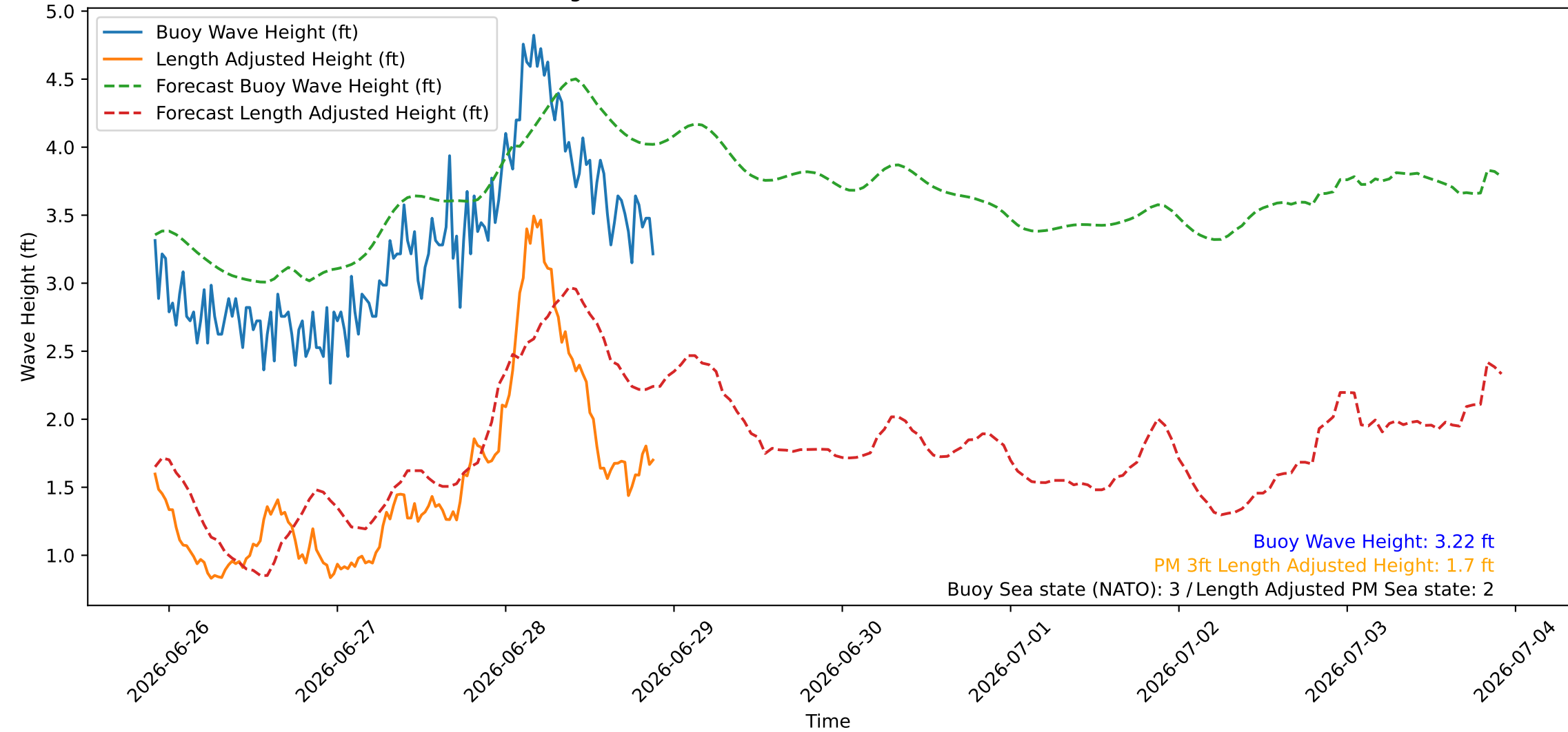
Wave Heights over Time for Green Beach at 2026-06-28 21:51:08
