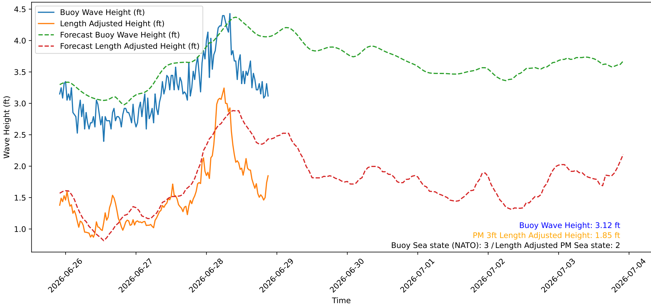
Wave Heights over Time for Oceanside Harbor at 2026-06-28 21:50:25
