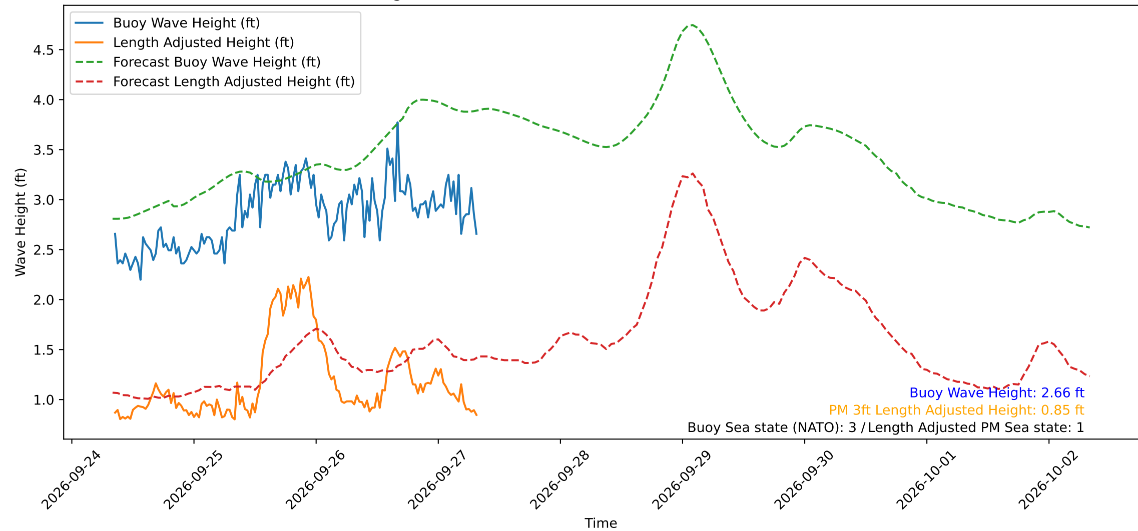
Wave Heights over Time for Oceanside Harbor at 2026-09-27 08:20:30
