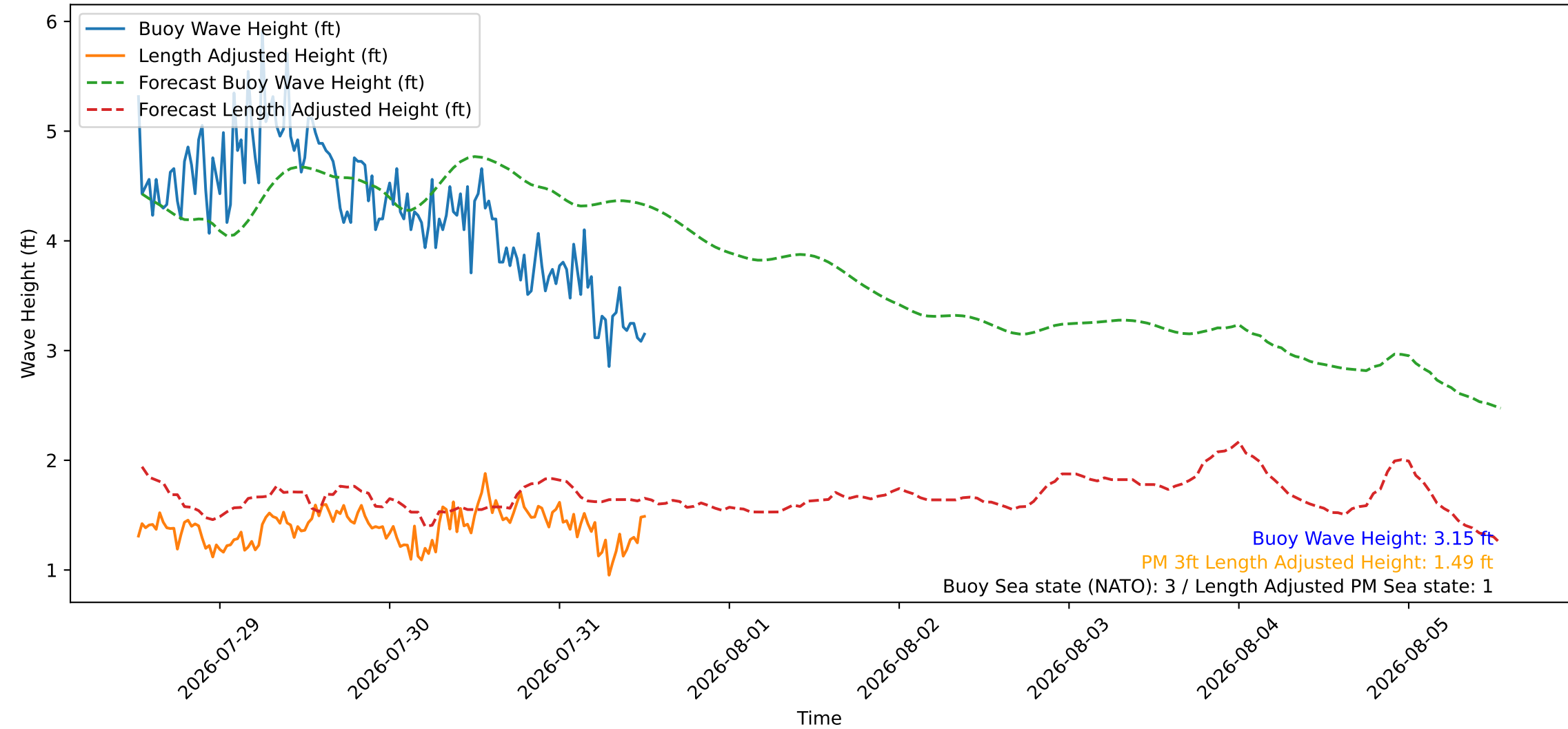
Wave Heights over Time for Oceanside Harbor at 2026-07-31 12:30:27
