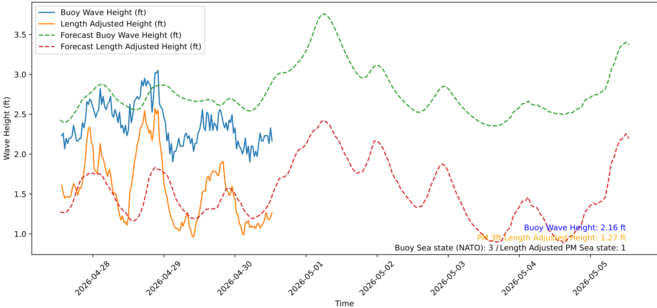
Wave Heights over Time for Oceanside Harbor at 2026-04-30 13:20:31
