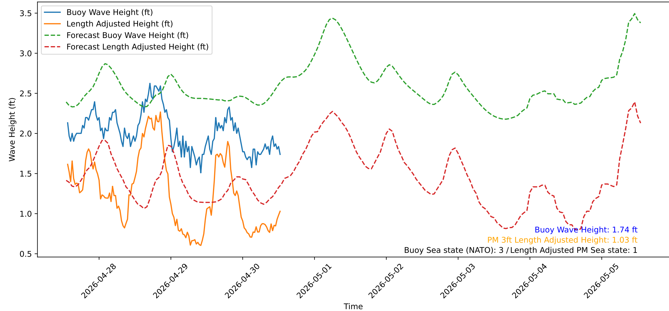
Wave Heights over Time for Red Beach at 2026-04-30 13:20:51
