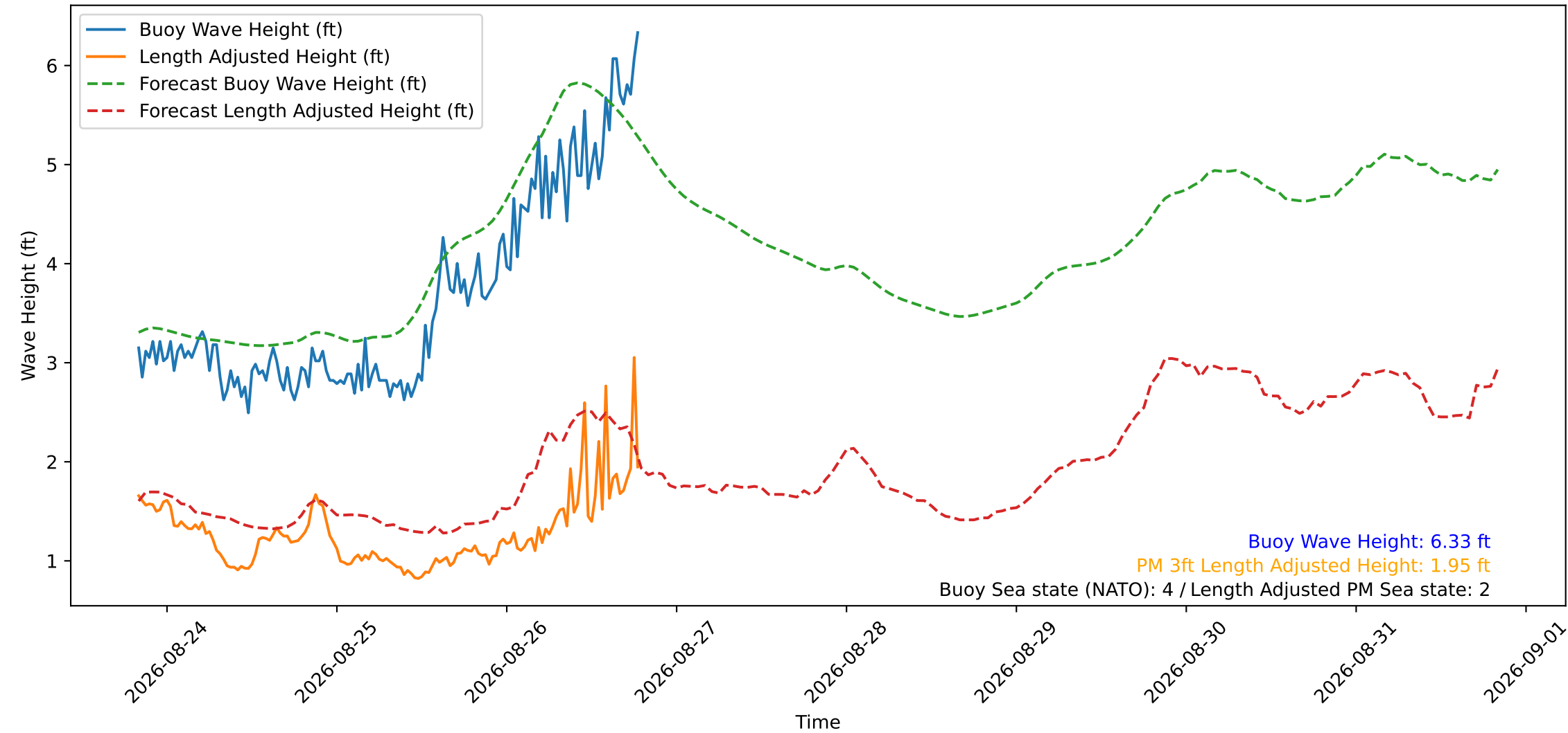
Wave Heights over Time for Green Beach at 2026-08-26 19:31:11
