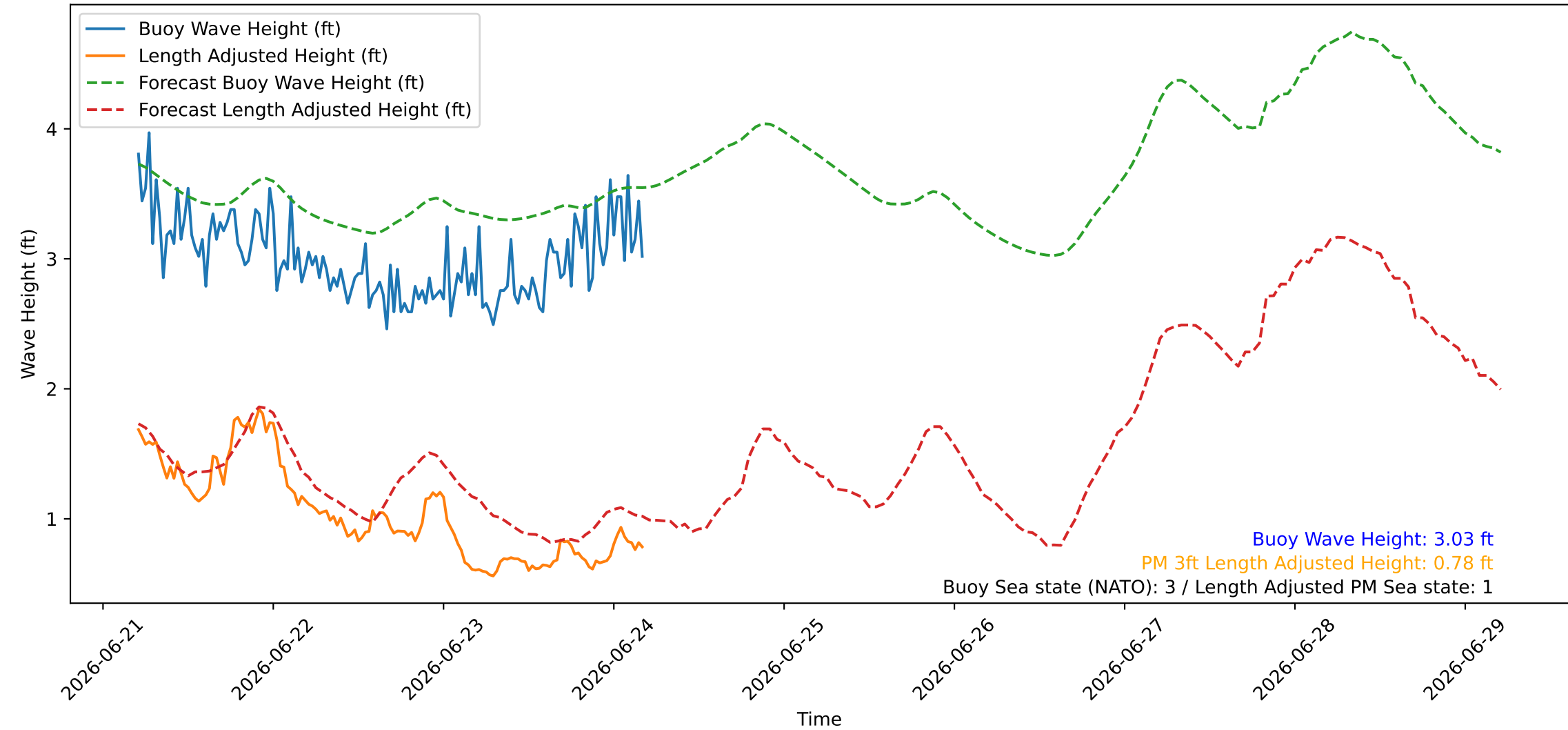
Wave Heights over Time for Green Beach at 2026-06-24 04:51:09
