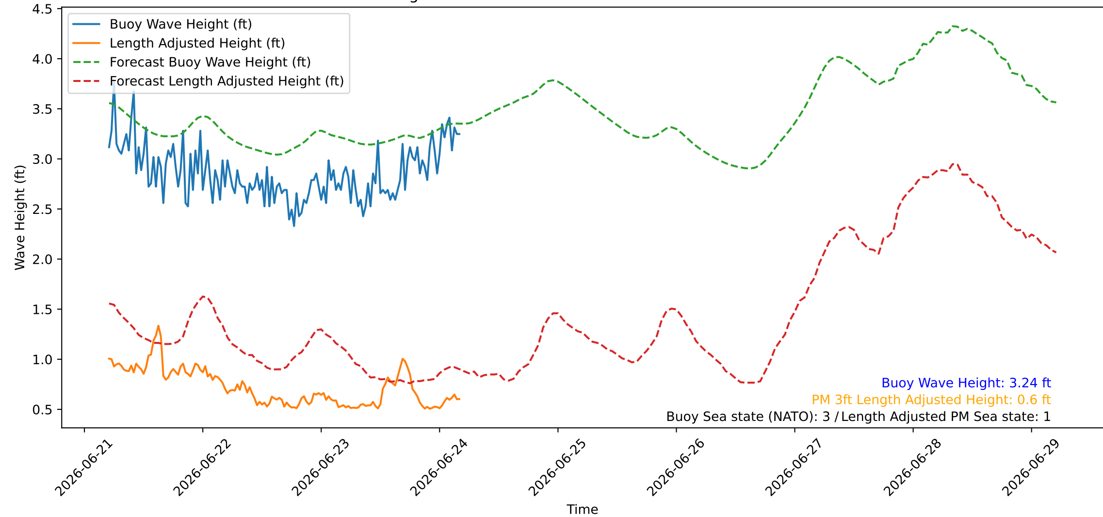
Wave Heights over Time for Red Beach at 2026-06-24 04:50:47
