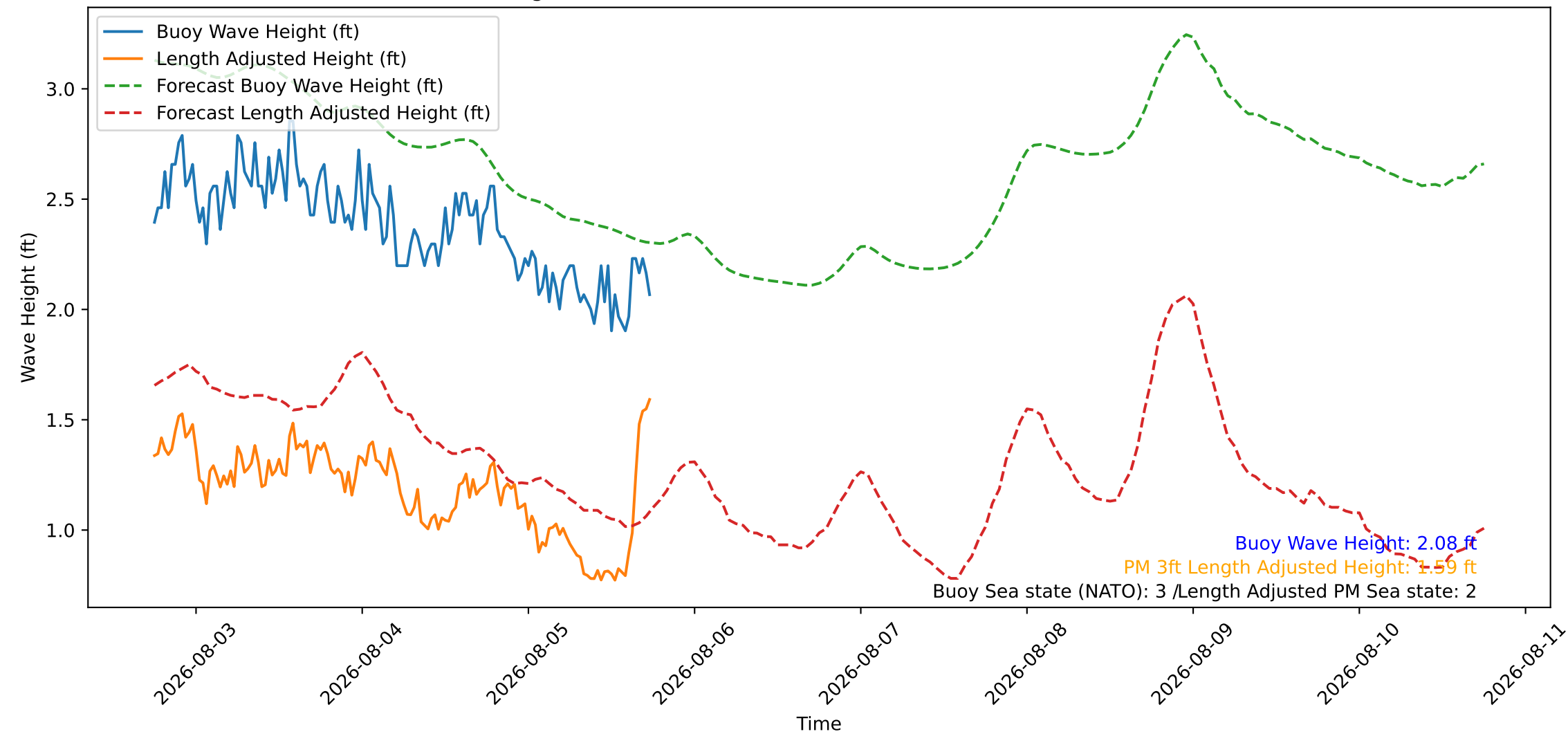
Wave Heights over Time for Oceanside Harbor at 2026-08-05 18:10:27
