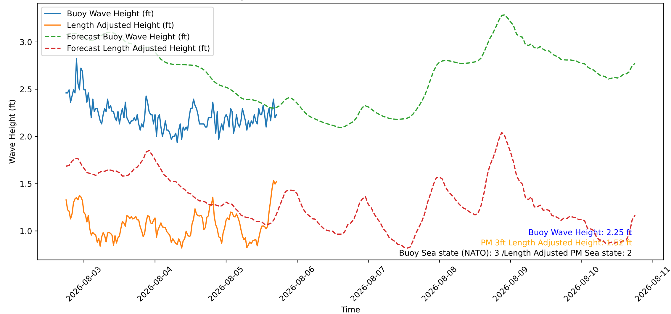
Wave Heights over Time for Green Beach at 2026-08-05 18:11:08
