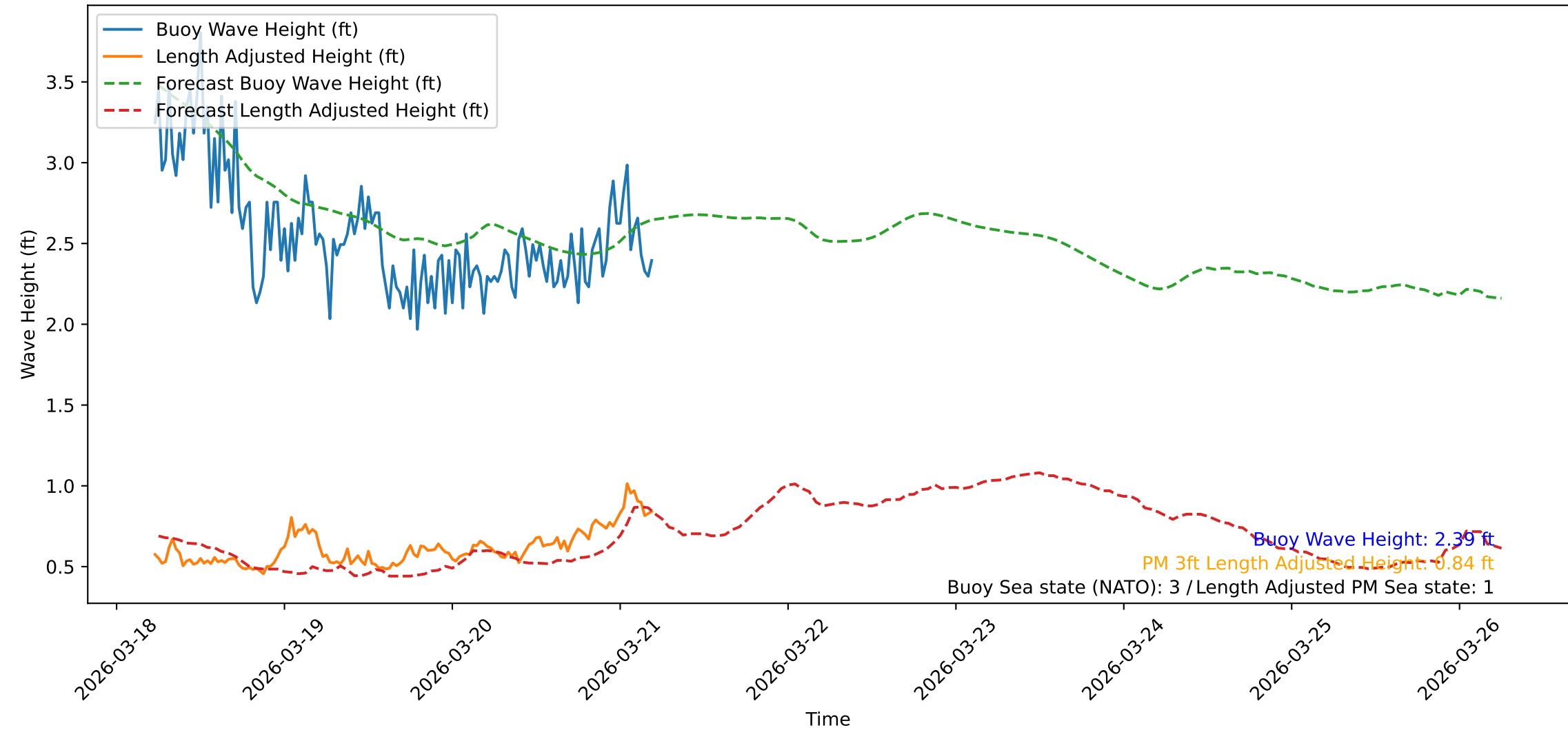
Wave Heights over Time for Oceanside Harbor at 2026-03-21 05:40:31
