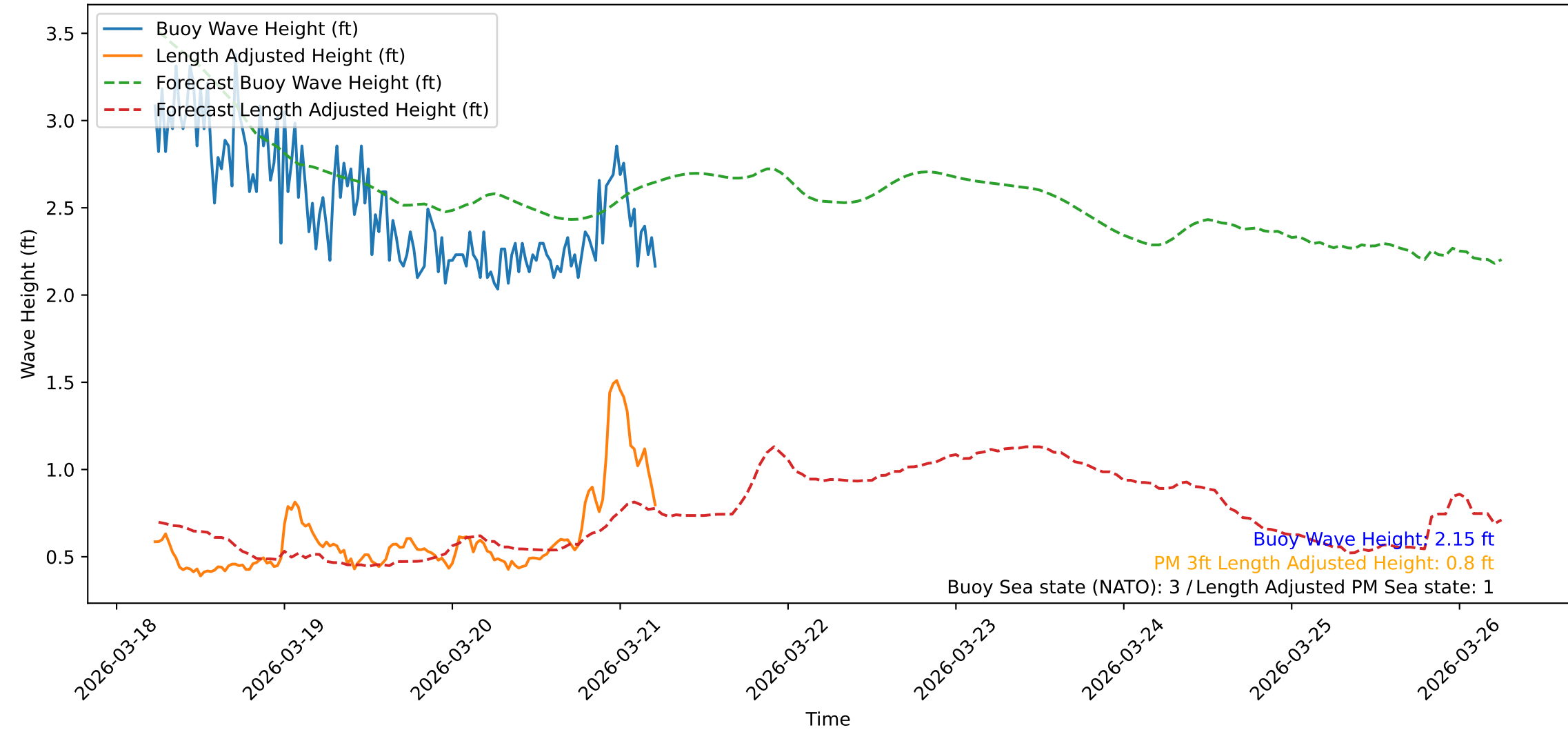
Wave Heights over Time for Green Beach at 2026-03-21 05:41:10
