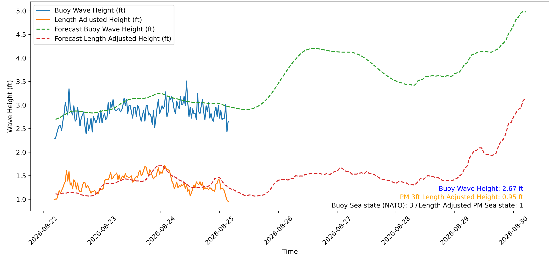
Wave Heights over Time for Oceanside Harbor at 2026-08-25 04:30:29
