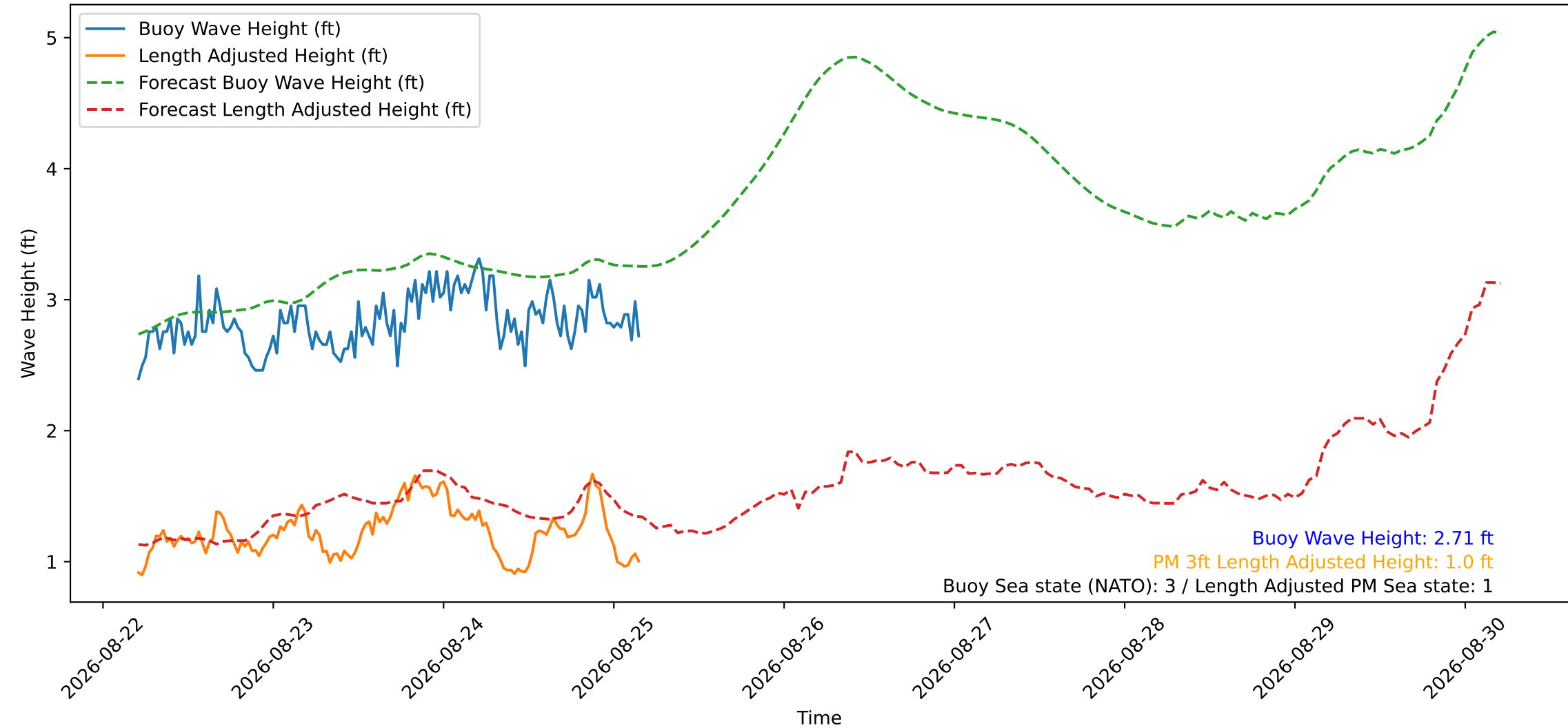
Wave Heights over Time for Green Beach at 2026-08-25 04:31:10
