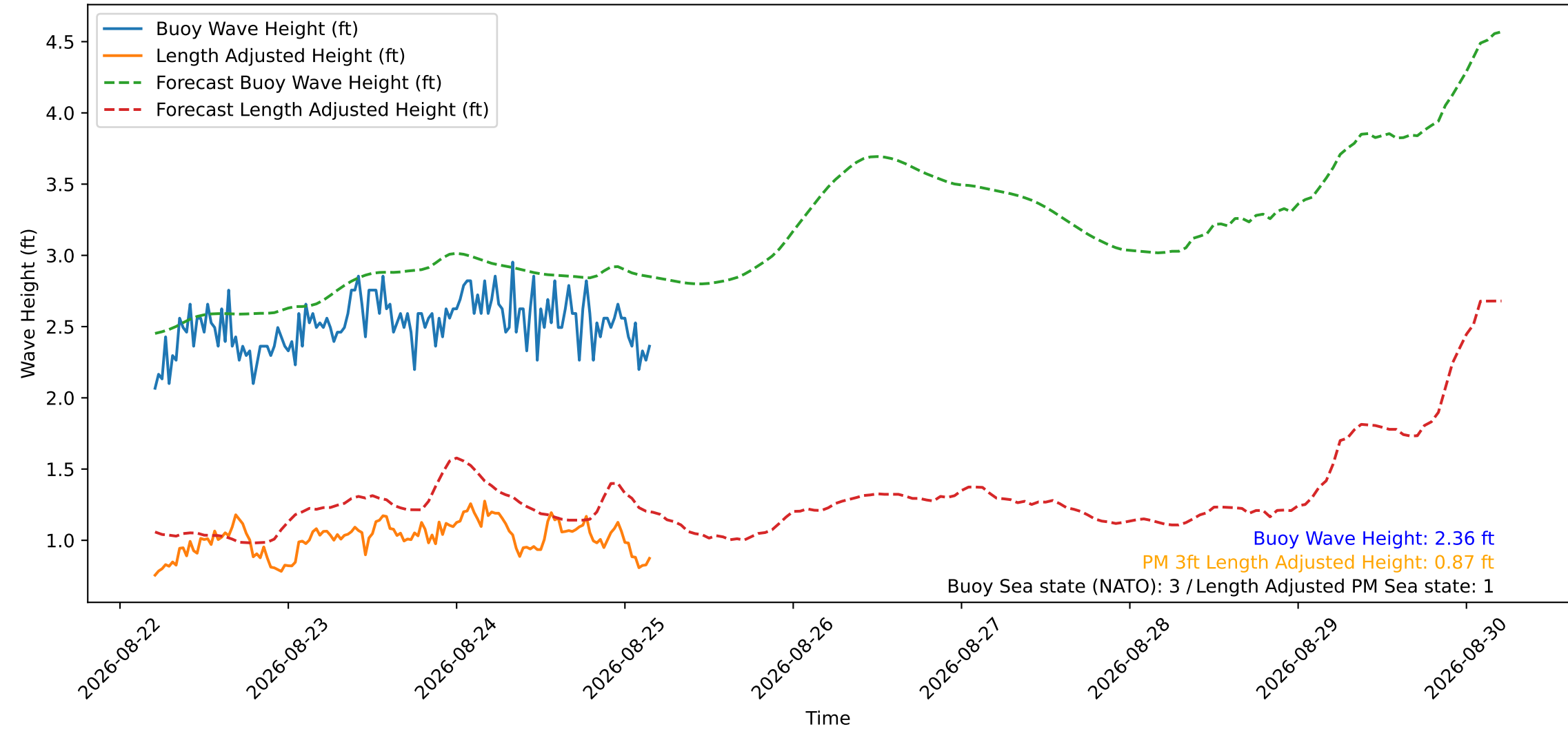
Wave Heights over Time for Red Beach at 2026-08-25 04:30:48
