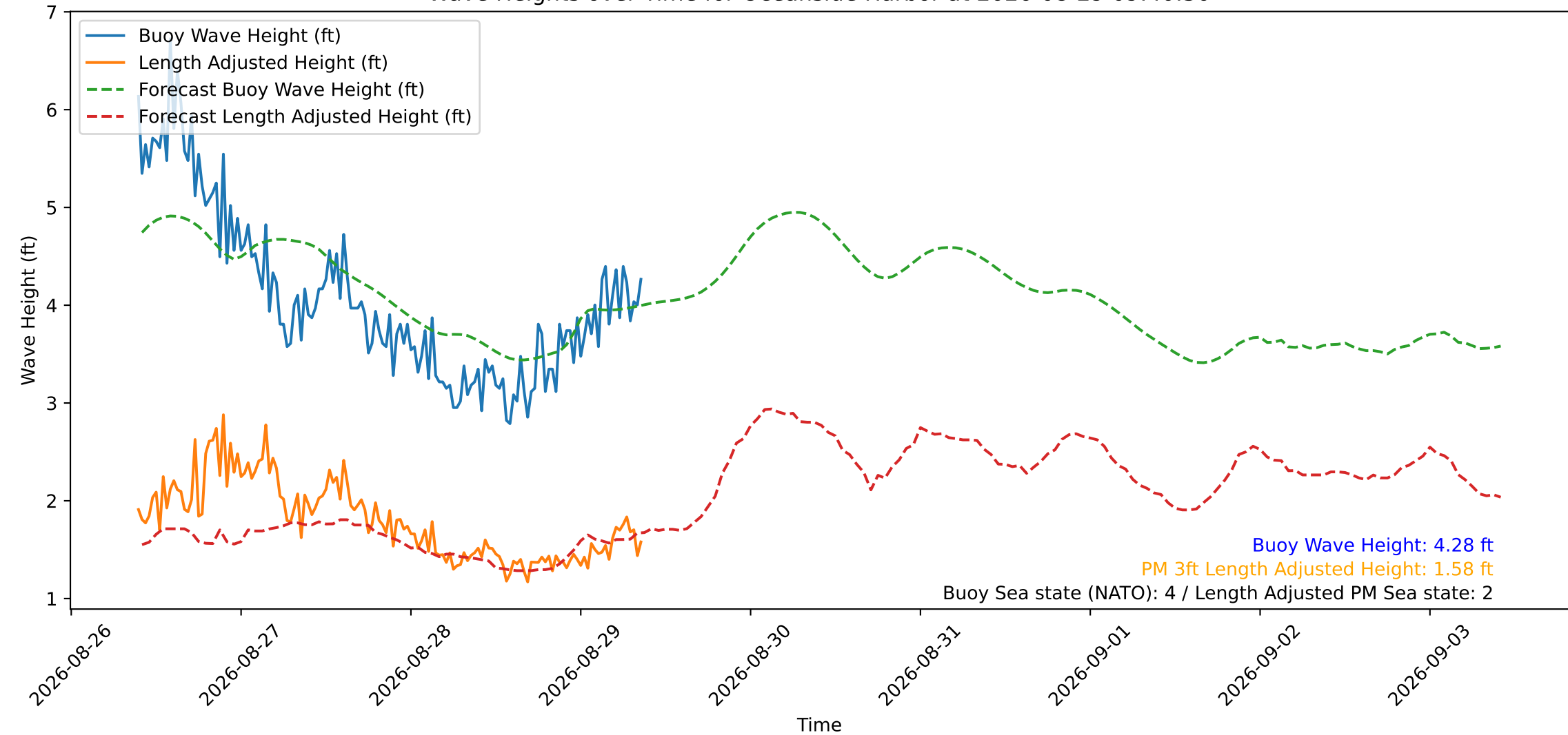
Wave Heights over Time for Oceanside Harbor at 2026-08-29 09:40:30
