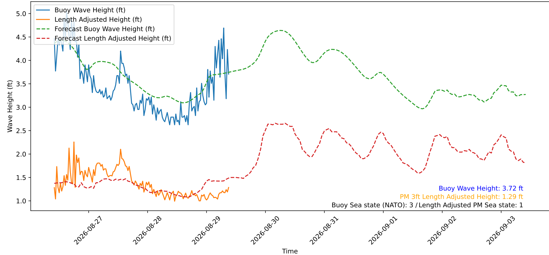
Wave Heights over Time for Red Beach at 2026-08-29 09:40:50
