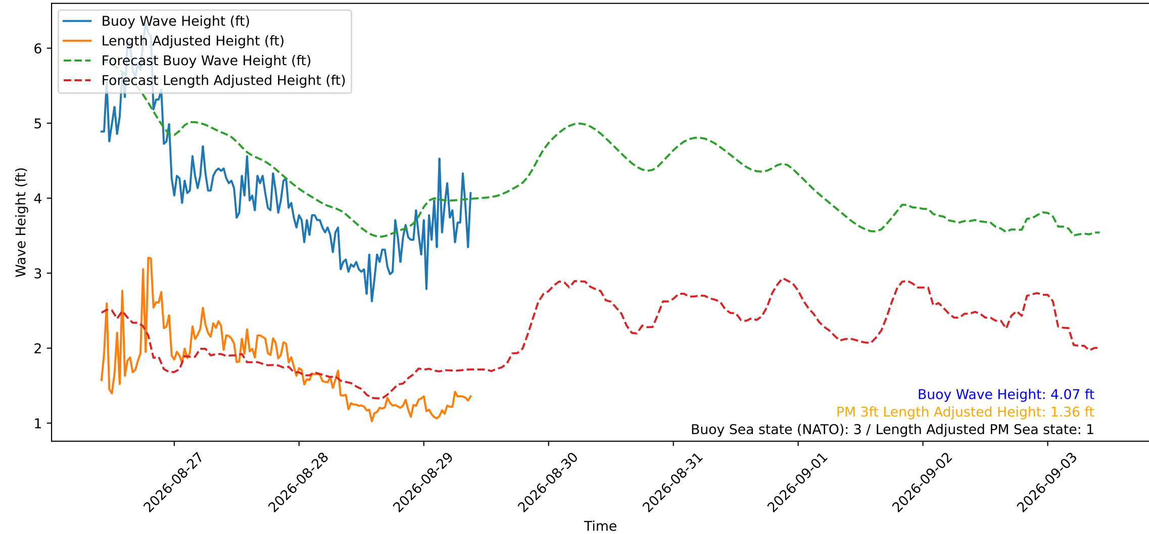
Wave Heights over Time for Green Beach at 2026-08-29 09:41:12
