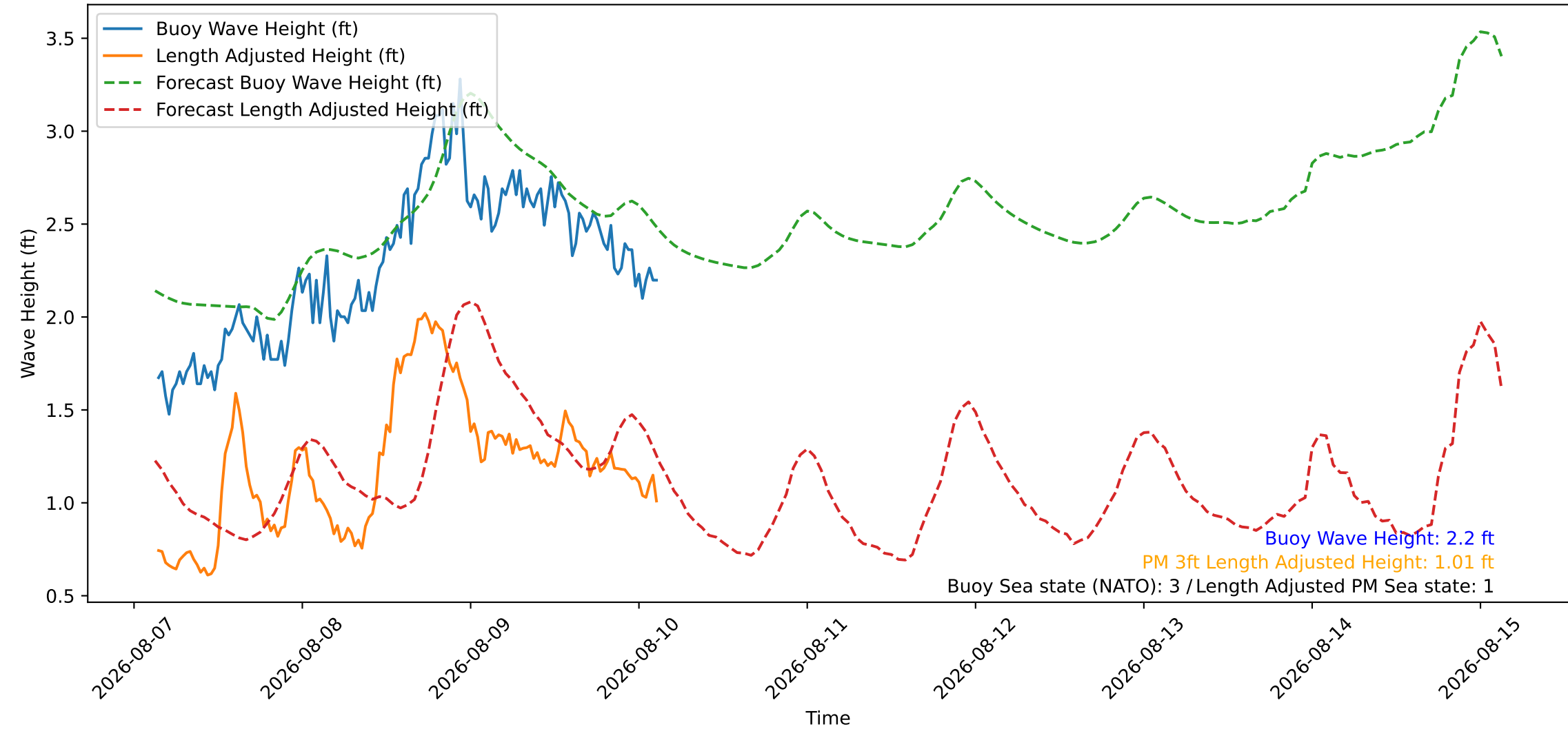
Wave Heights over Time for Red Beach at 2026-08-10 03:10:46
