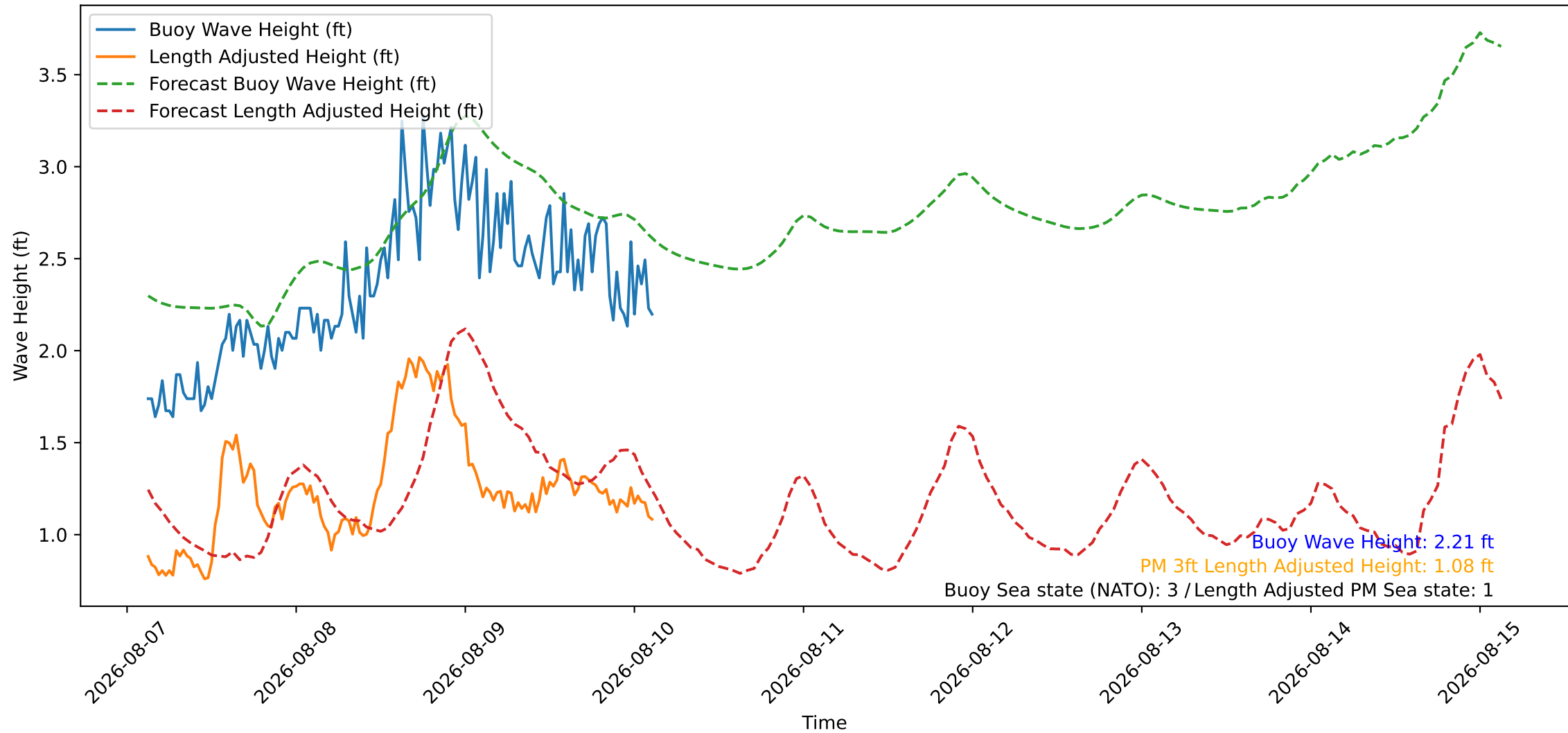
Wave Heights over Time for Oceanside Harbor at 2026-08-10 03:10:26
