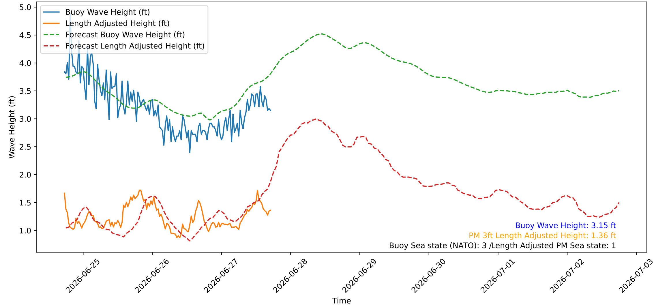
Wave Heights over Time for Oceanside Harbor at 2026-06-27 17:30:26
