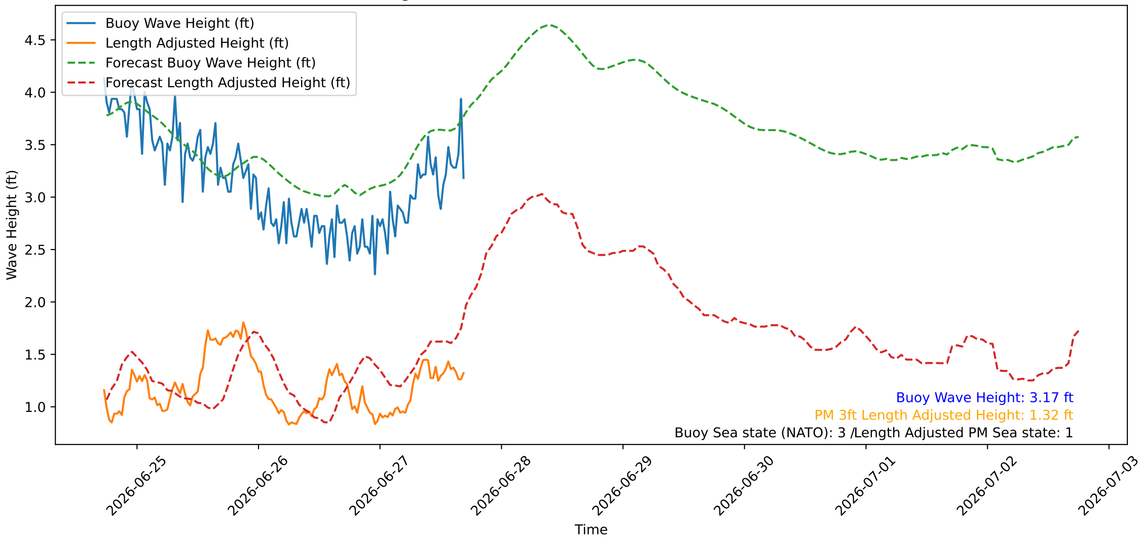
Wave Heights over Time for Green Beach at 2026-06-27 17:31:08
