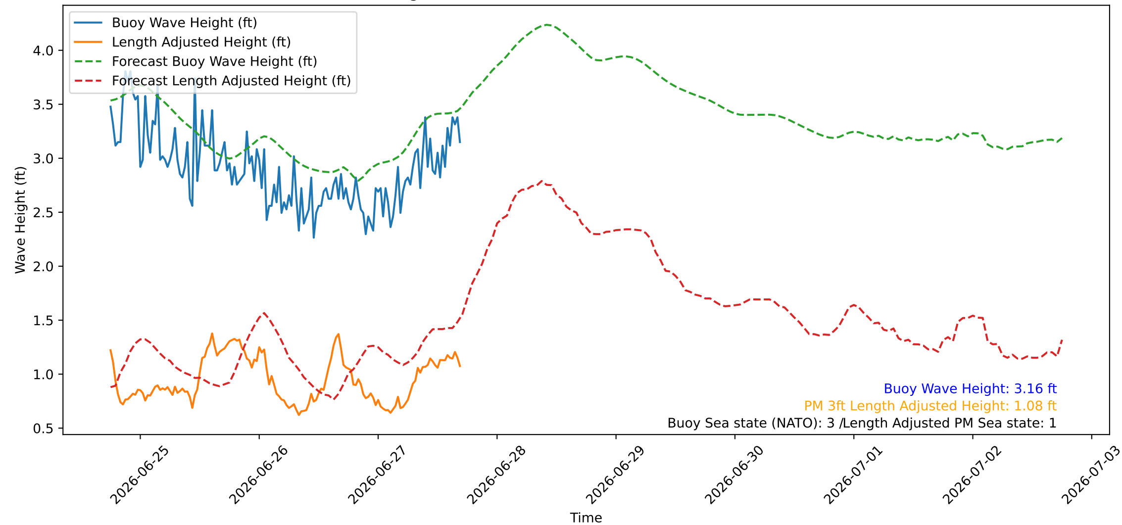
Wave Heights over Time for Red Beach at 2026-06-27 17:30:45
