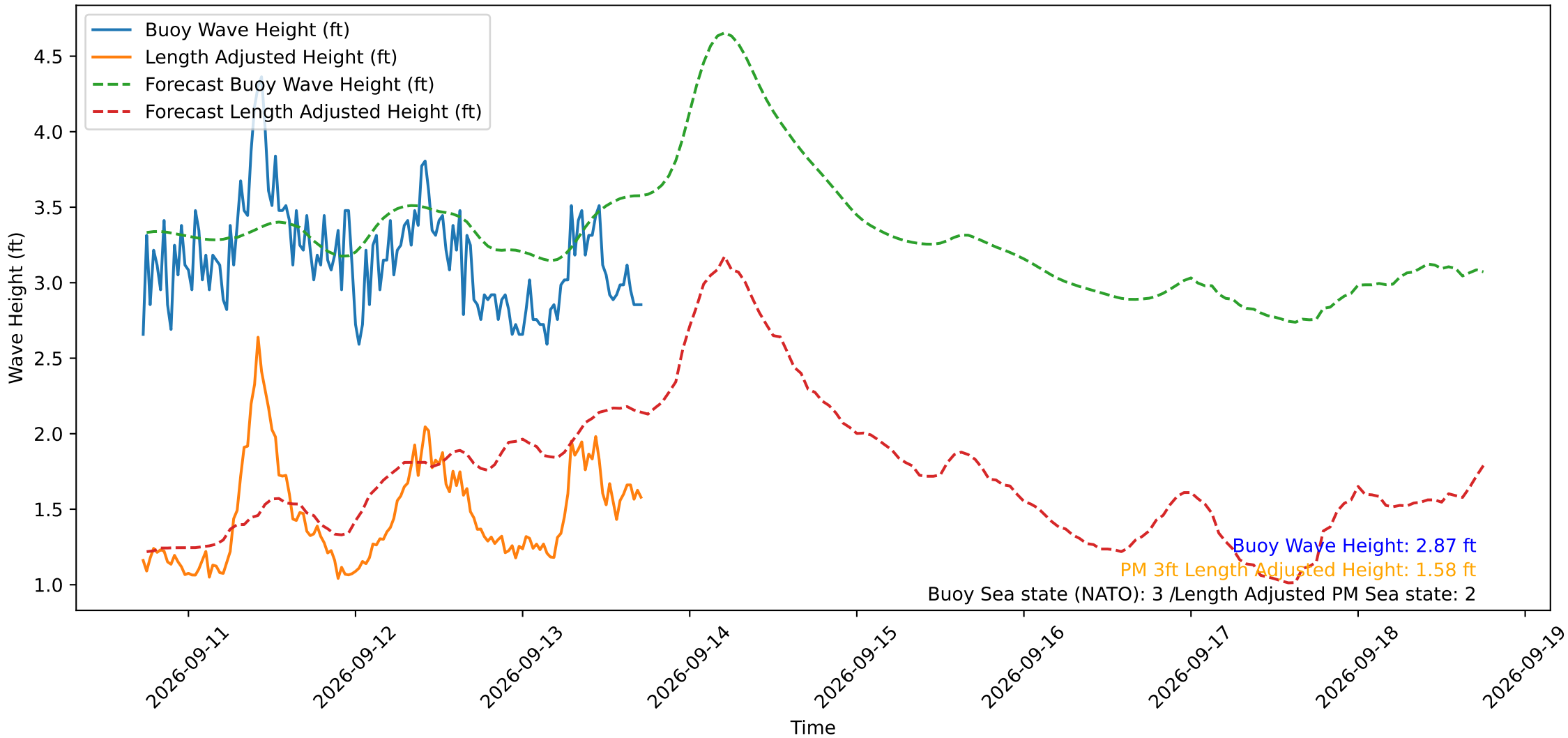
Wave Heights over Time for Oceanside Harbor at 2026-09-13 17:40:29
