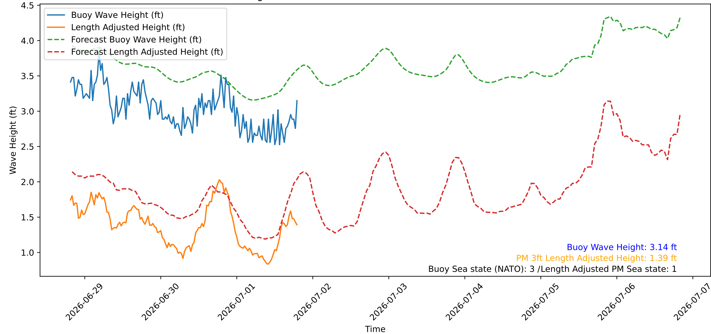
Wave Heights over Time for Green Beach at 2026-07-01 19:41:08
