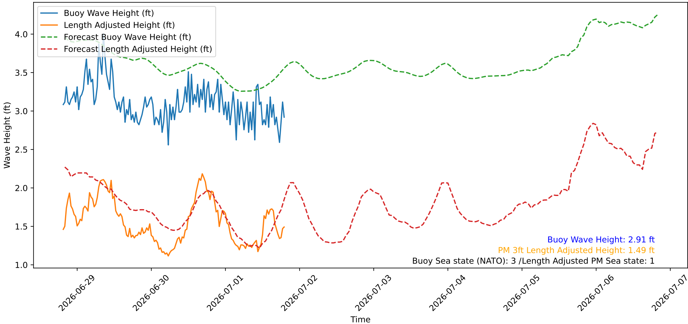
Wave Heights over Time for Oceanside Harbor at 2026-07-01 19:40:26
