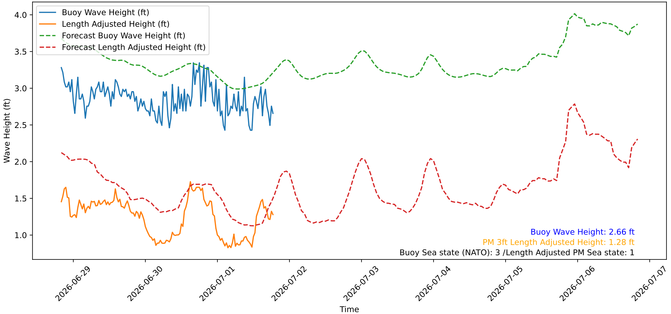
Wave Heights over Time for Red Beach at 2026-07-01 19:40:45
