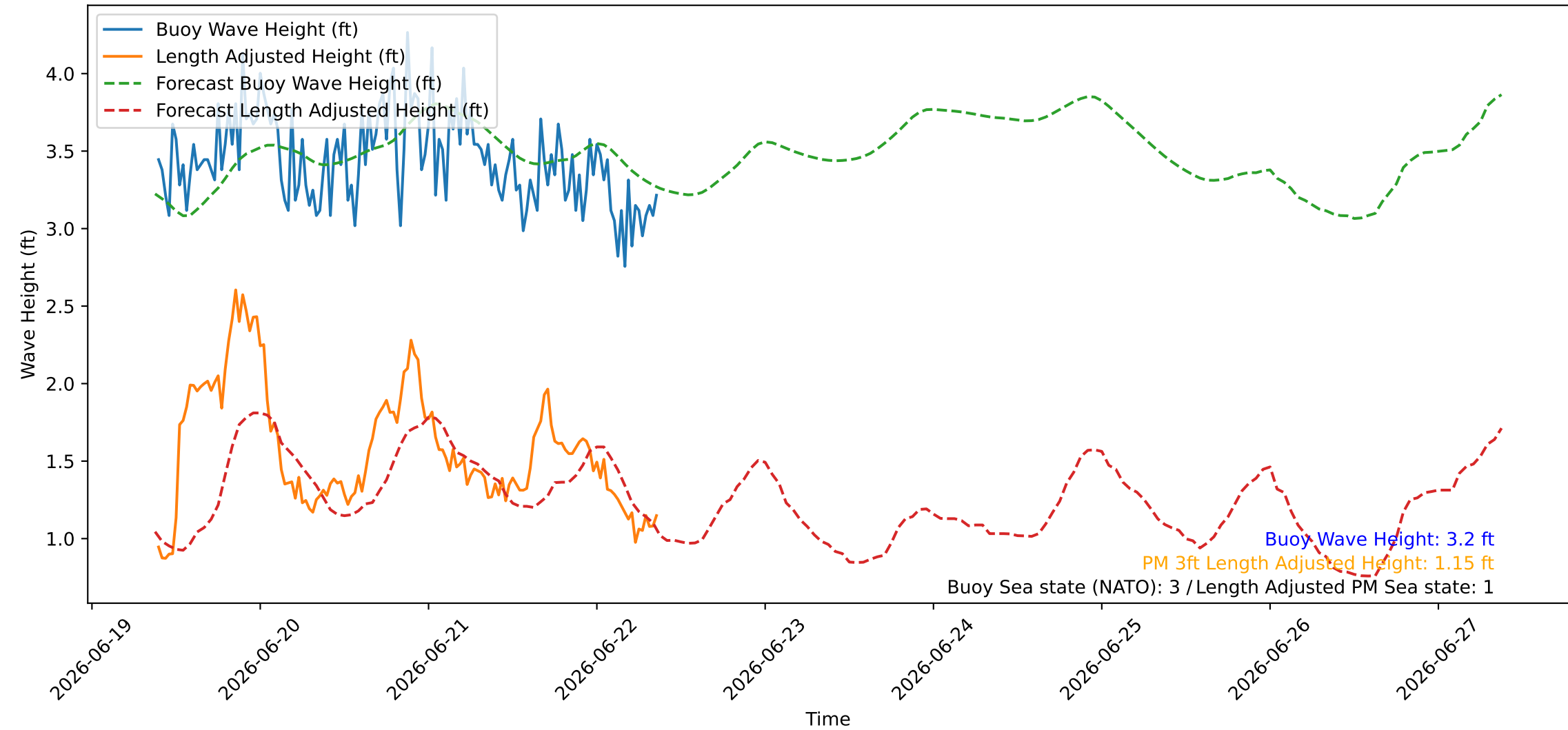
Wave Heights over Time for Oceanside Harbor at 2026-06-22 09:20:26
