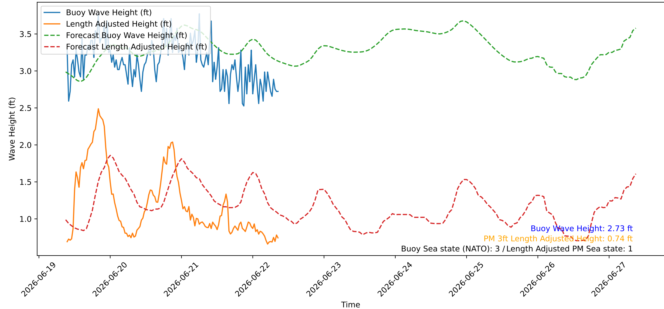
Wave Heights over Time for Red Beach at 2026-06-22 09:20:47
