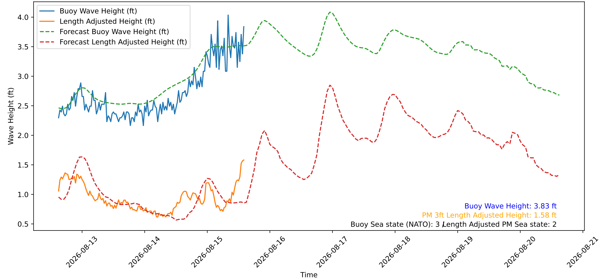
Wave Heights over Time for Red Beach at 2026-08-15 14:50:47
