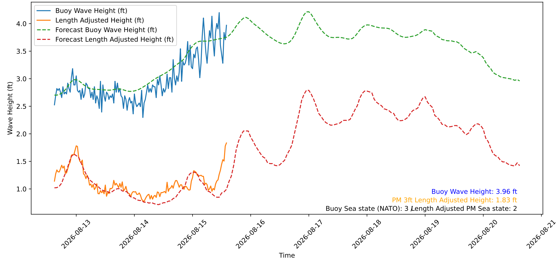
Wave Heights over Time for Oceanside Harbor at 2026-08-15 14:50:26
