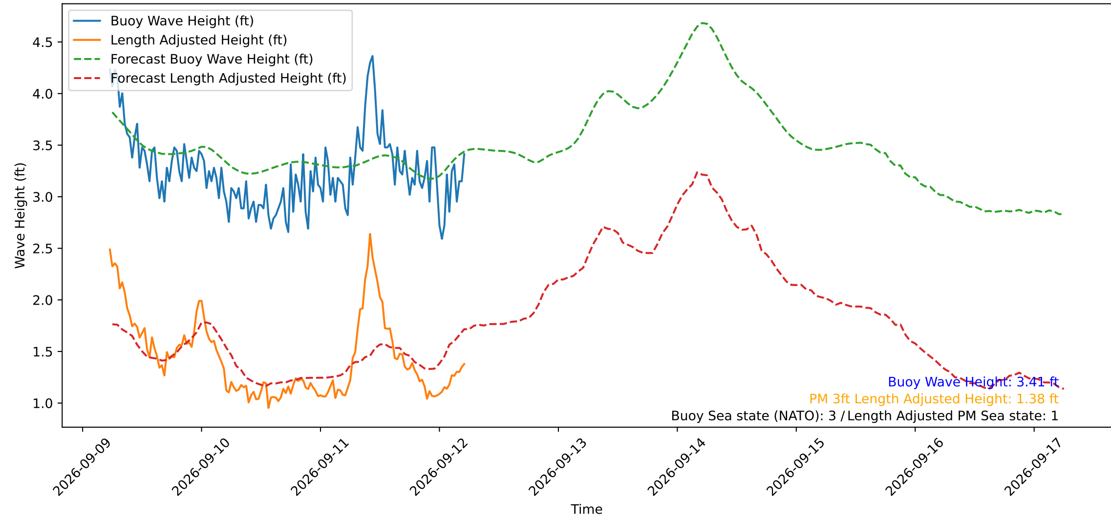
Wave Heights over Time for Oceanside Harbor at 2026-09-12 05:30:30
