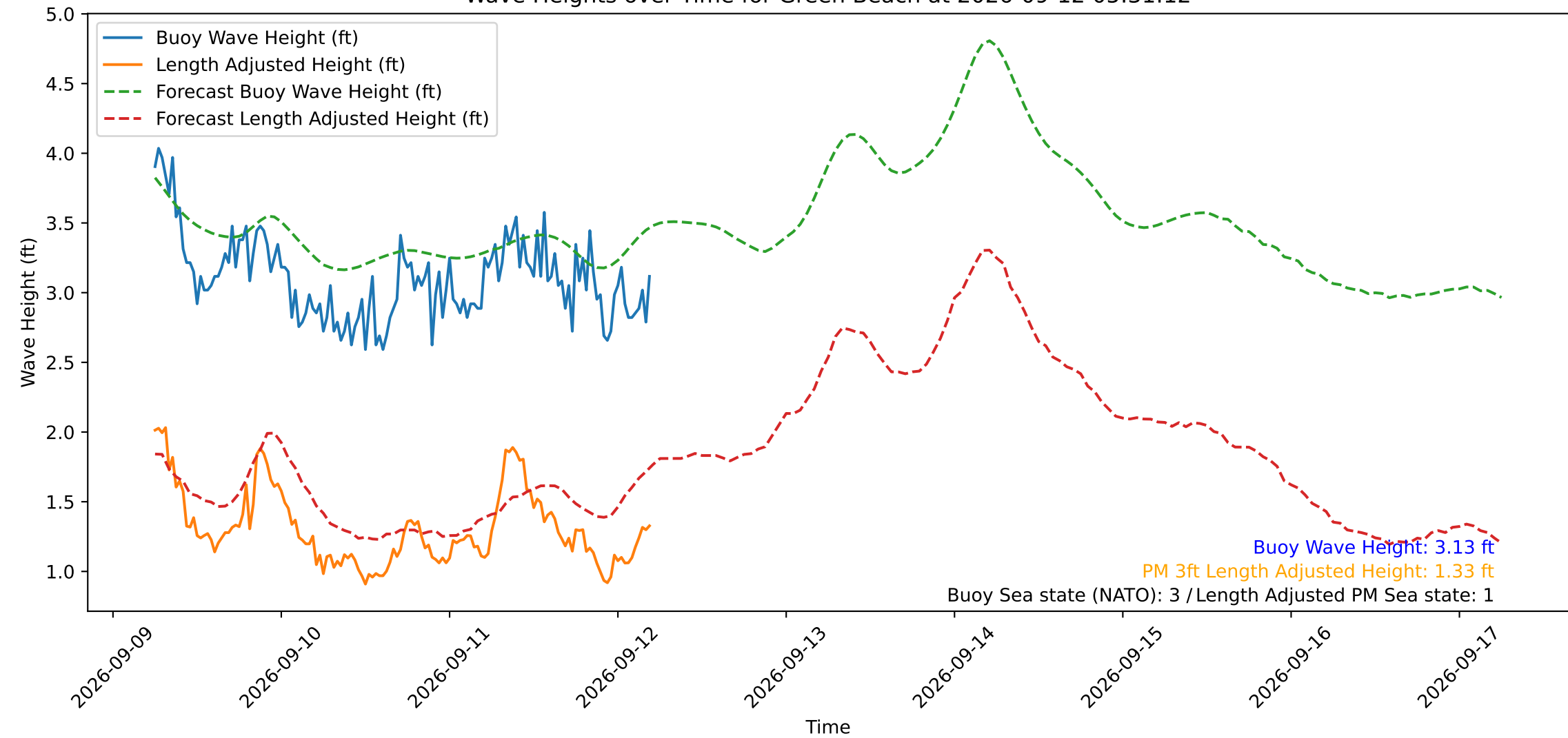
Wave Heights over Time for Green Beach at 2026-09-12 05:31:12
