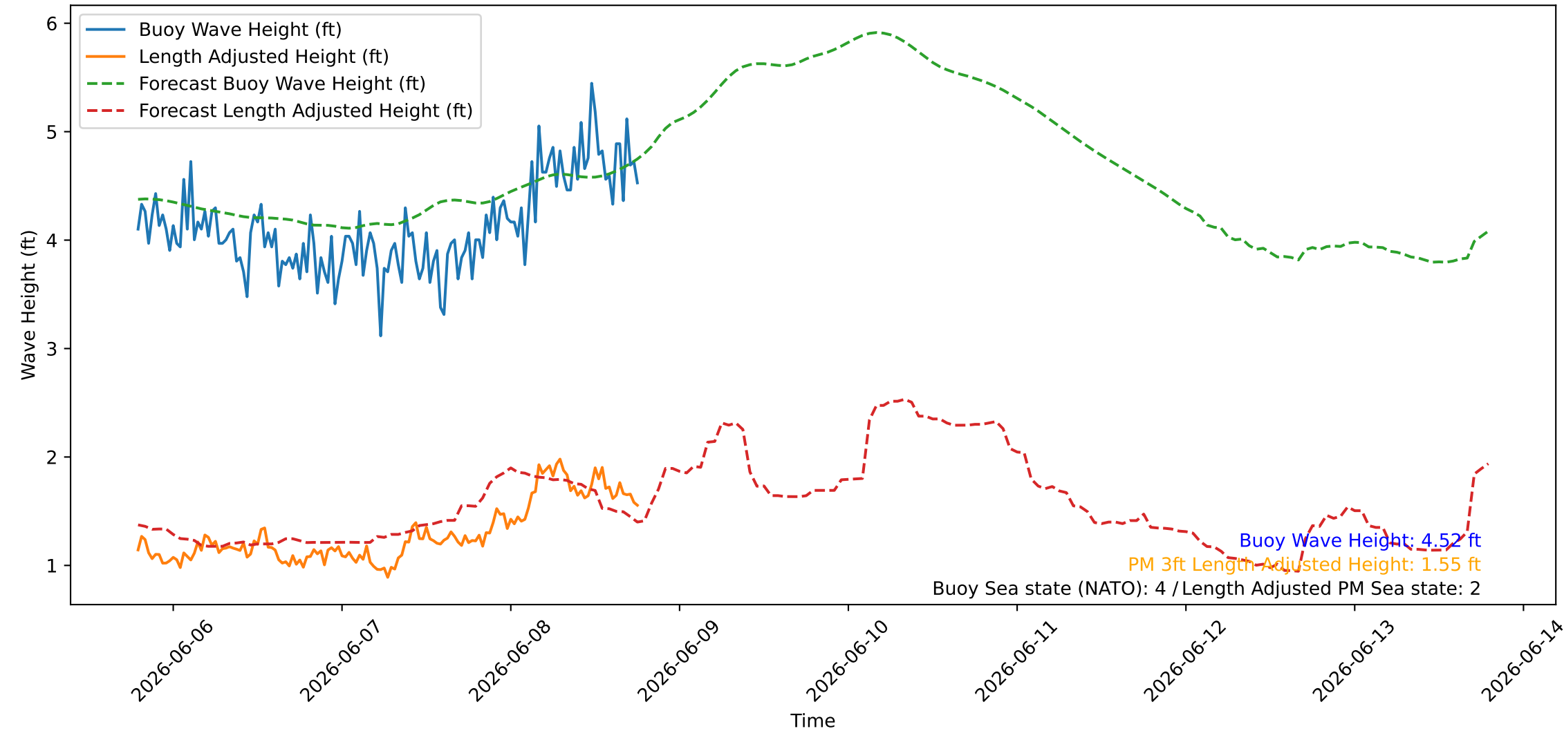
Wave Heights over Time for Green Beach at 2026-06-08 18:51:13
