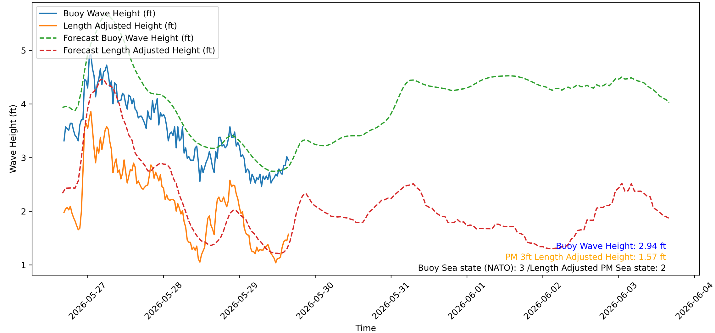
Wave Heights over Time for Green Beach at 2026-05-29 16:21:05
