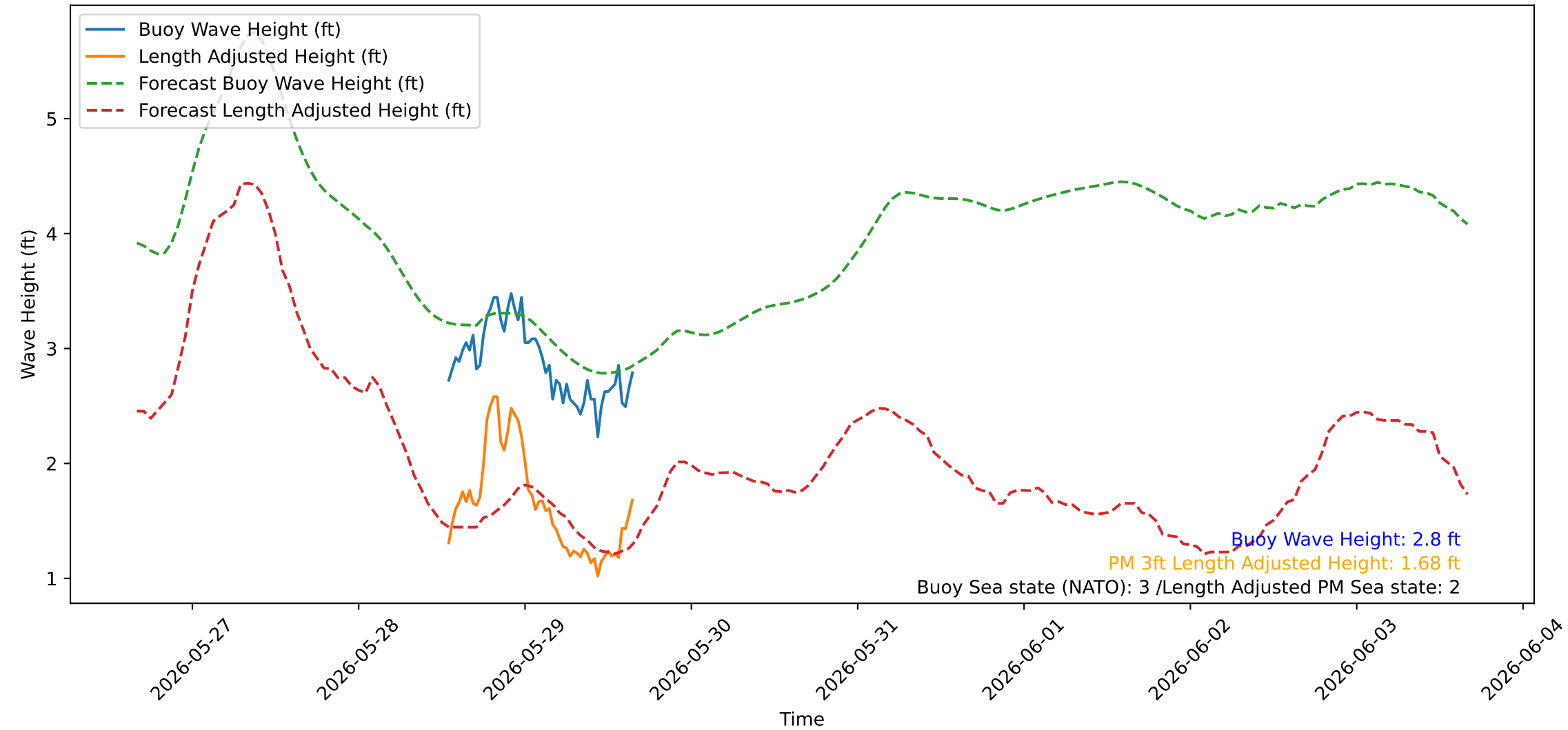
Wave Heights over Time for Oceanside Harbor at 2026-05-29 16:20:22
