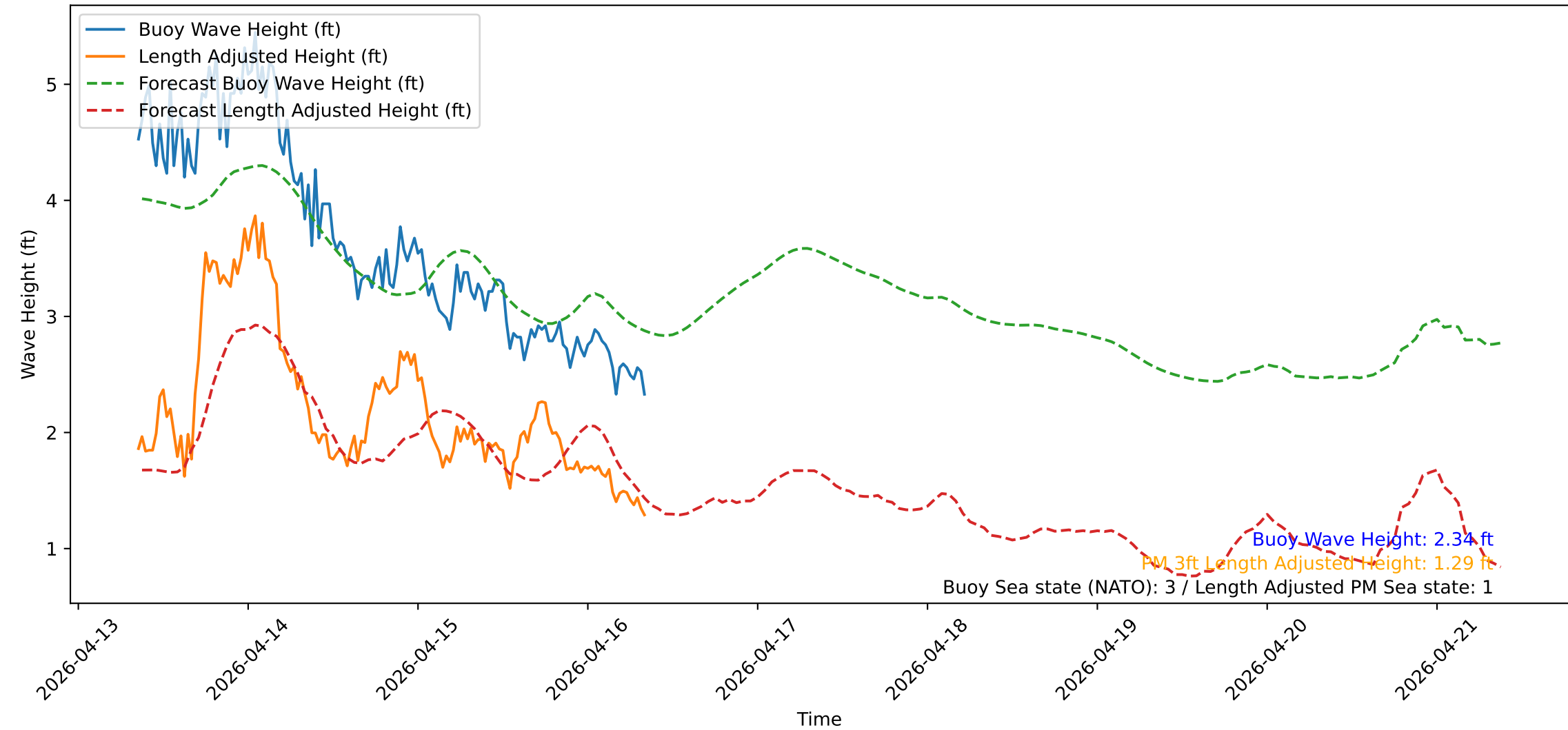
Wave Heights over Time for Oceanside Harbor at 2026-04-16 08:30:31
