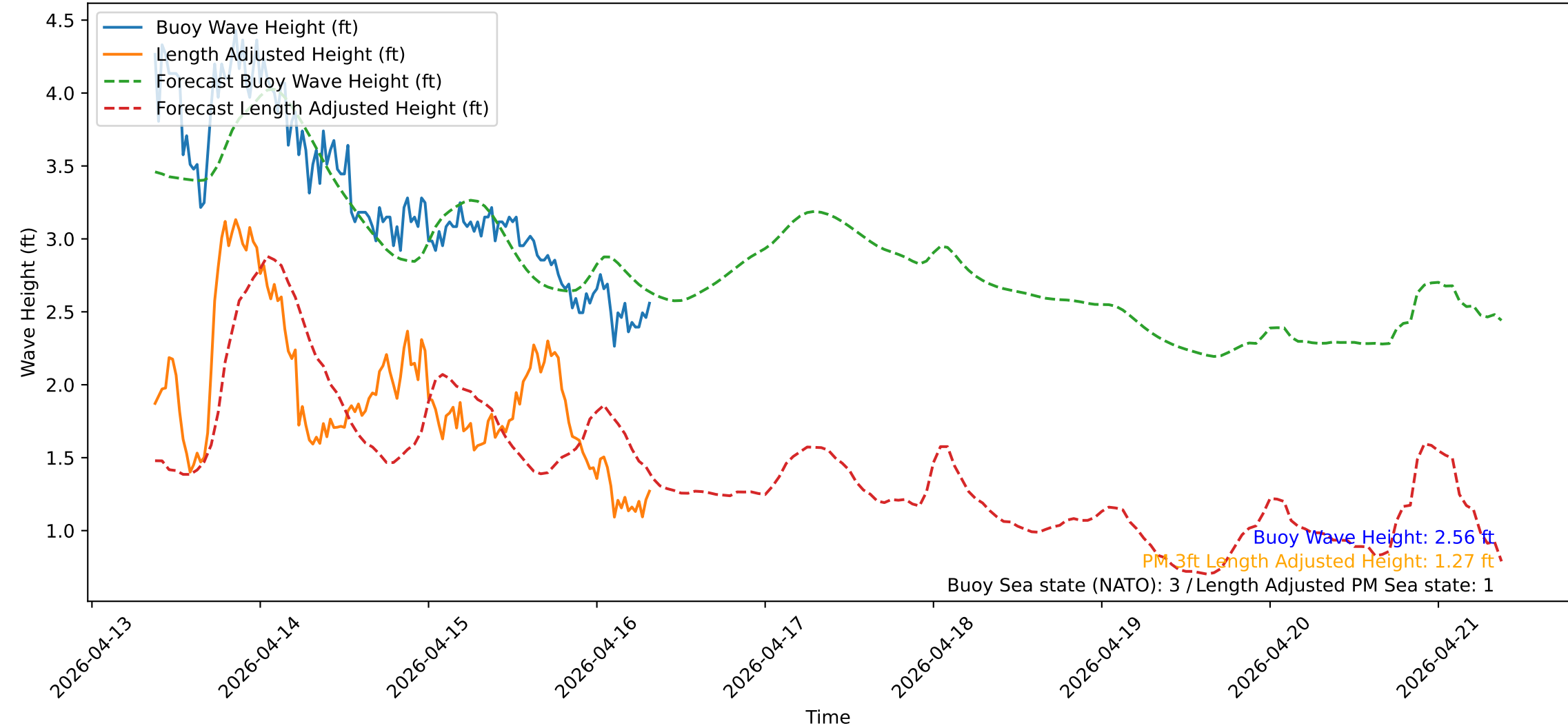
Wave Heights over Time for Red Beach at 2026-04-16 08:30:50
