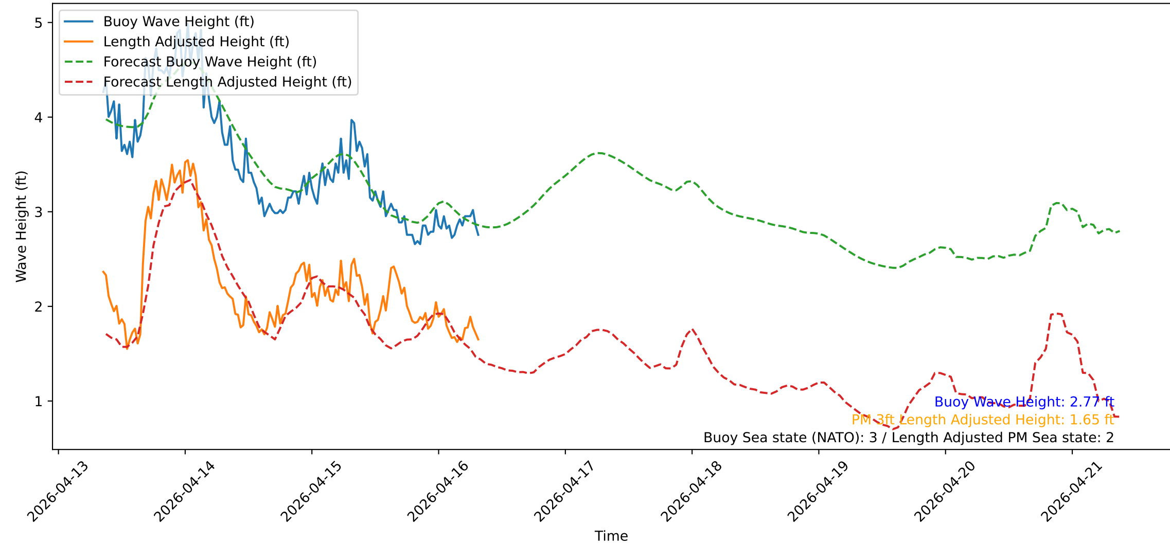
Wave Heights over Time for Green Beach at 2026-04-16 08:31:13
