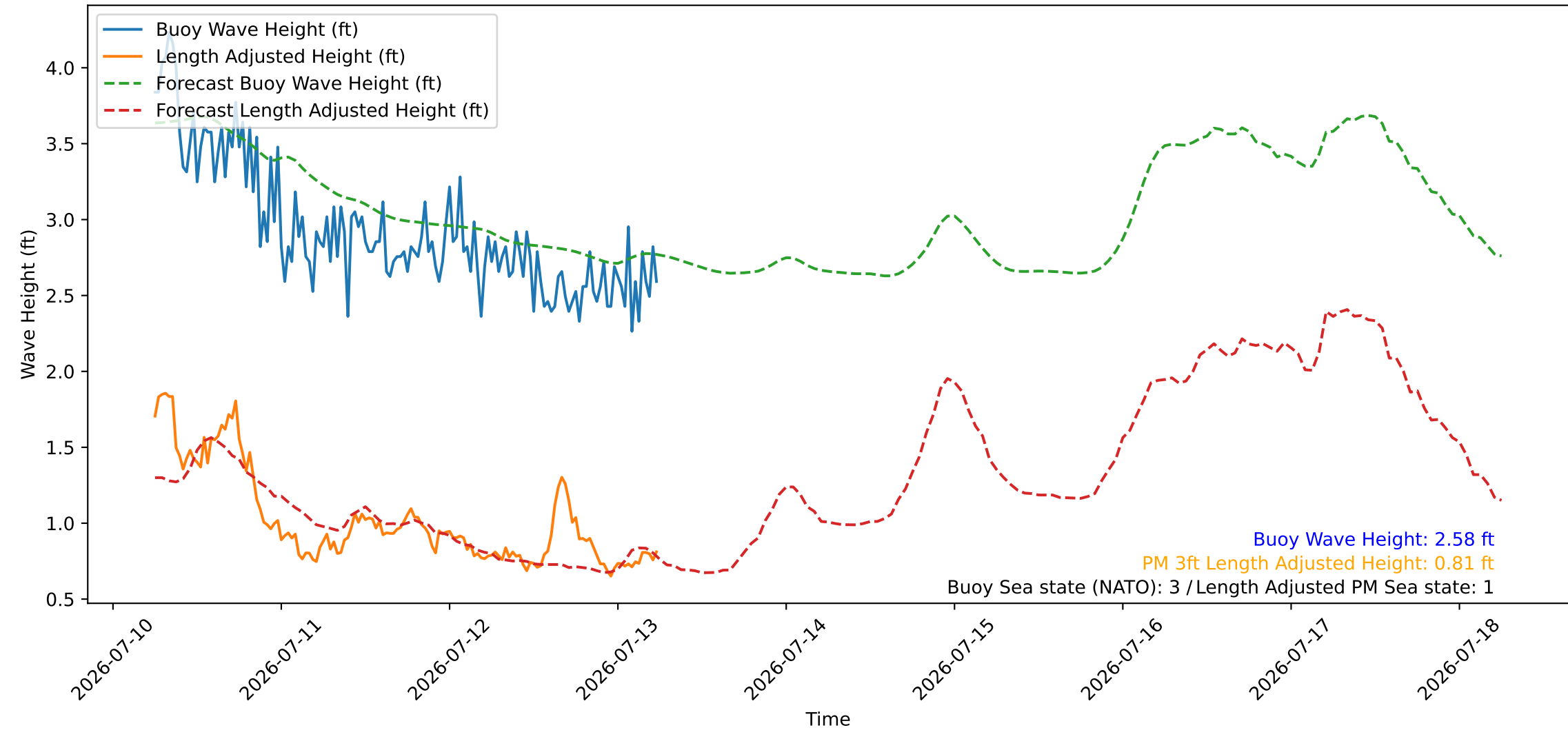
Wave Heights over Time for Oceanside Harbor at 2026-07-13 06:10:25
