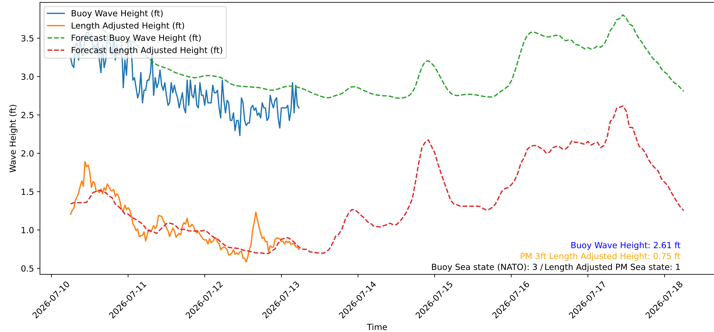
Wave Heights over Time for Green Beach at 2026-07-13 06:11:06
