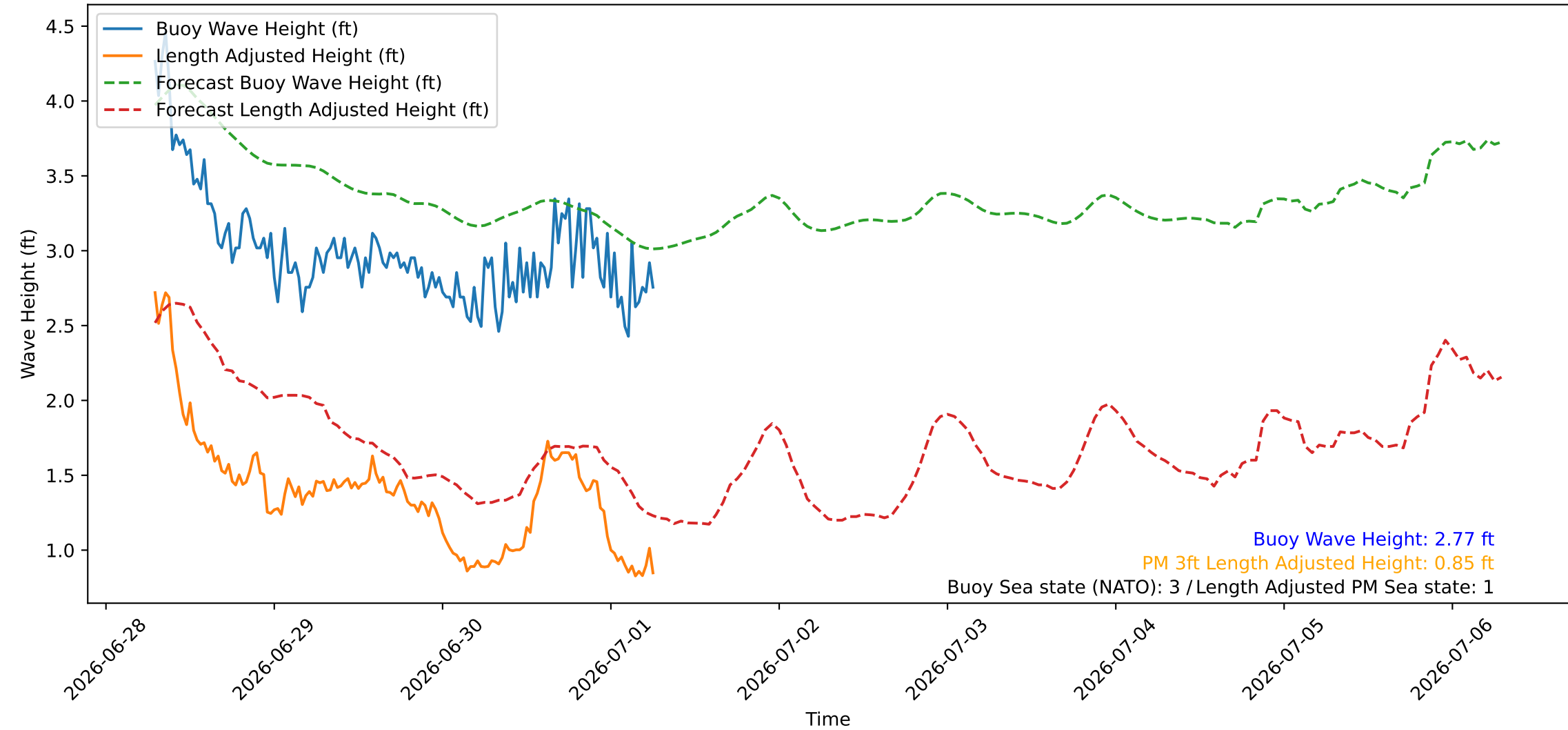
Wave Heights over Time for Red Beach at 2026-07-01 06:40:46
