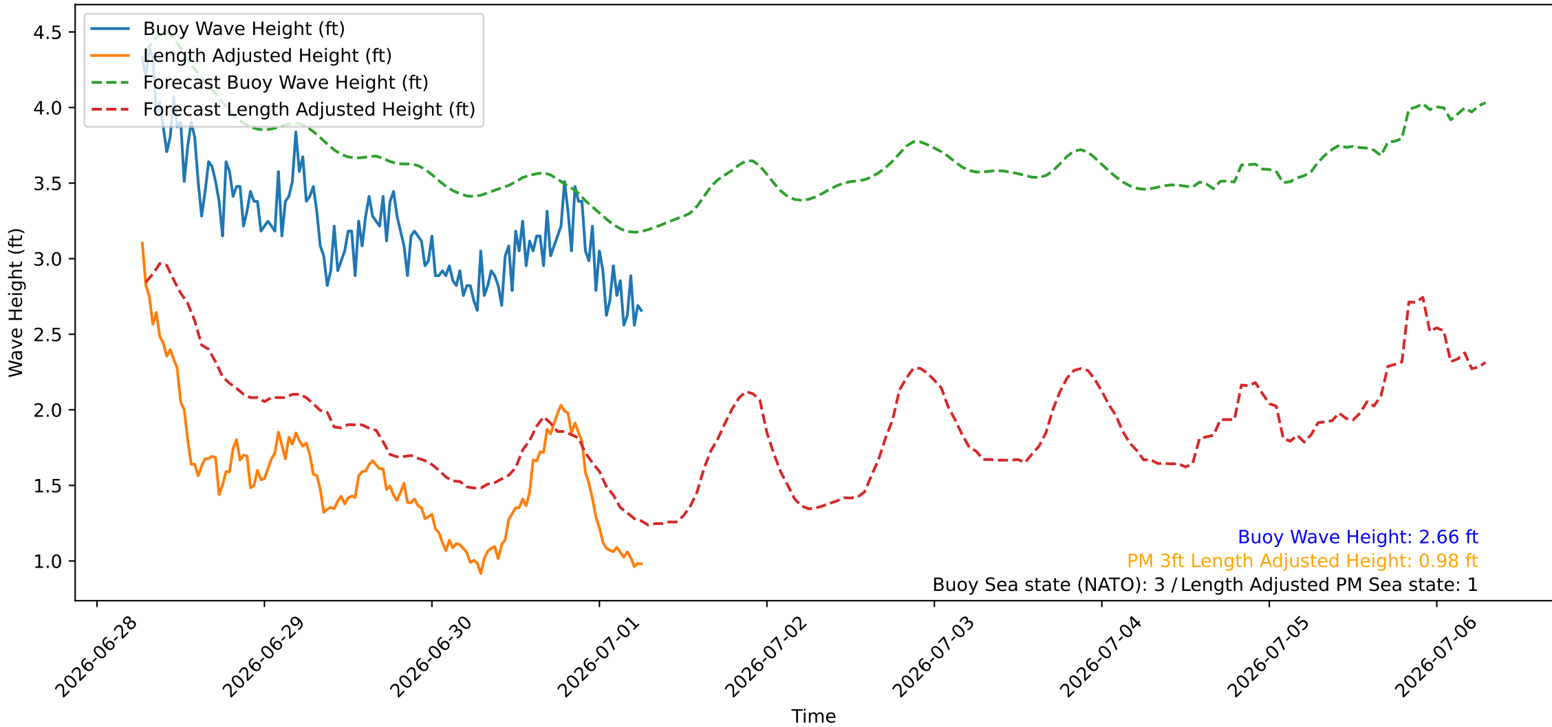
Wave Heights over Time for Green Beach at 2026-07-01 06:41:08
