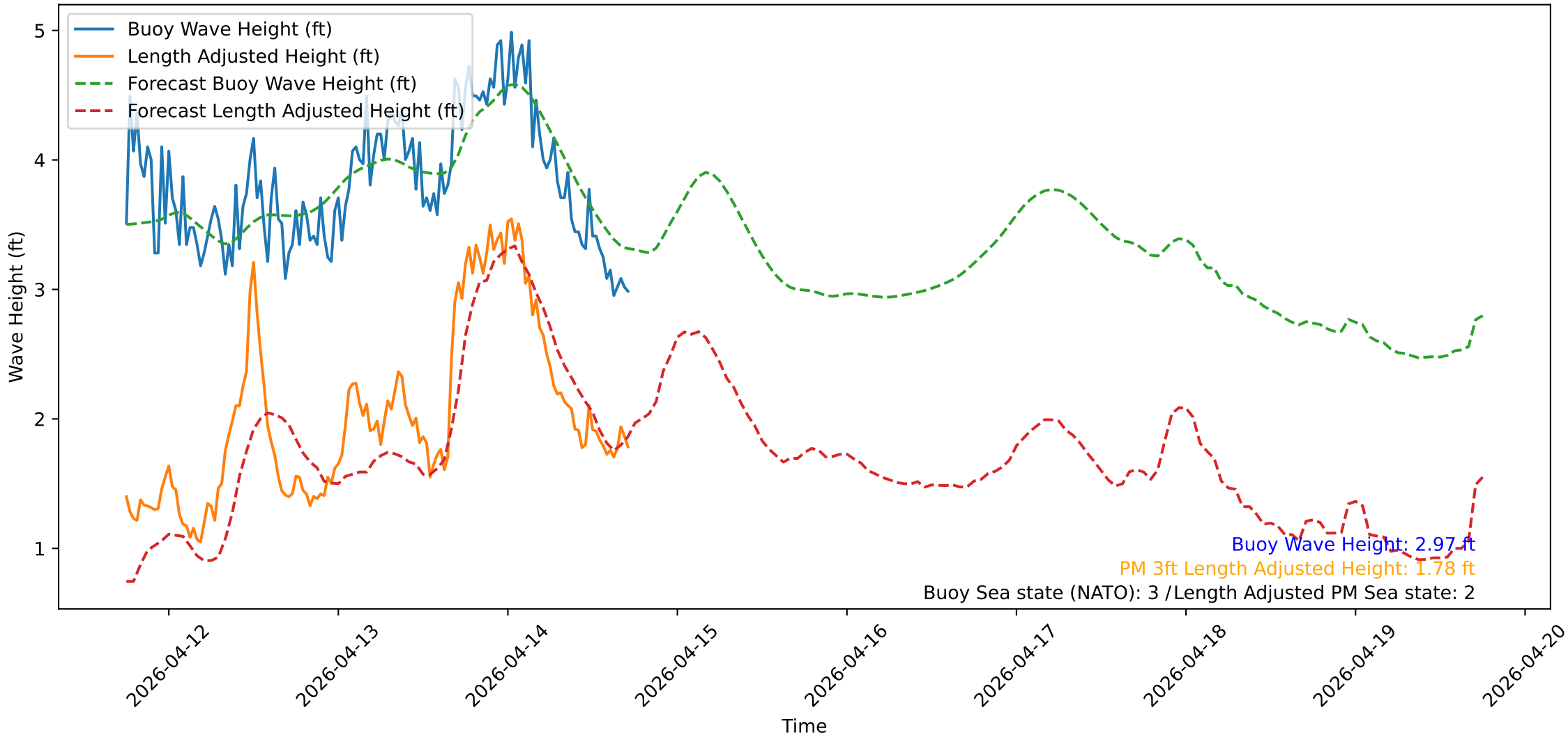
Wave Heights over Time for Green Beach at 2026-04-14 17:51:14
