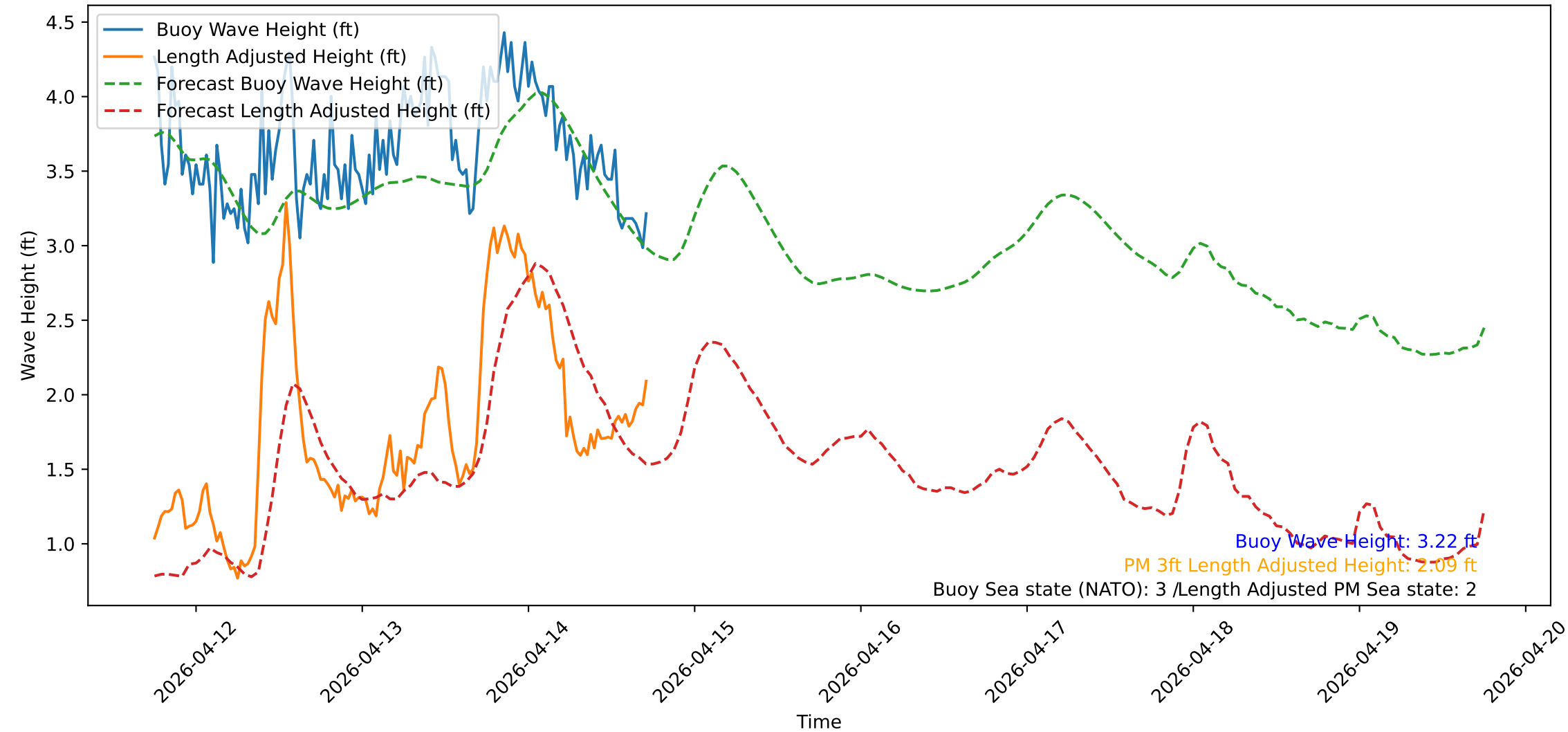
Wave Heights over Time for Red Beach at 2026-04-14 17:50:52
