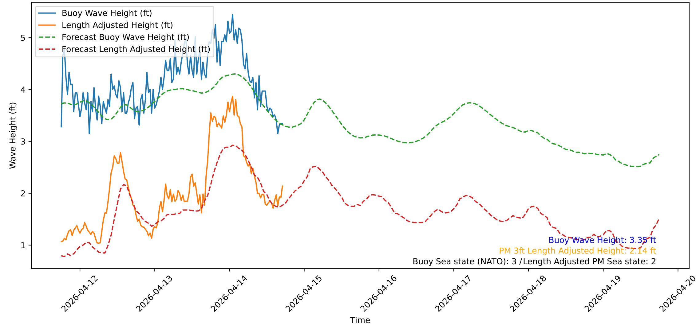
Wave Heights over Time for Oceanside Harbor at 2026-04-14 17:50:32
