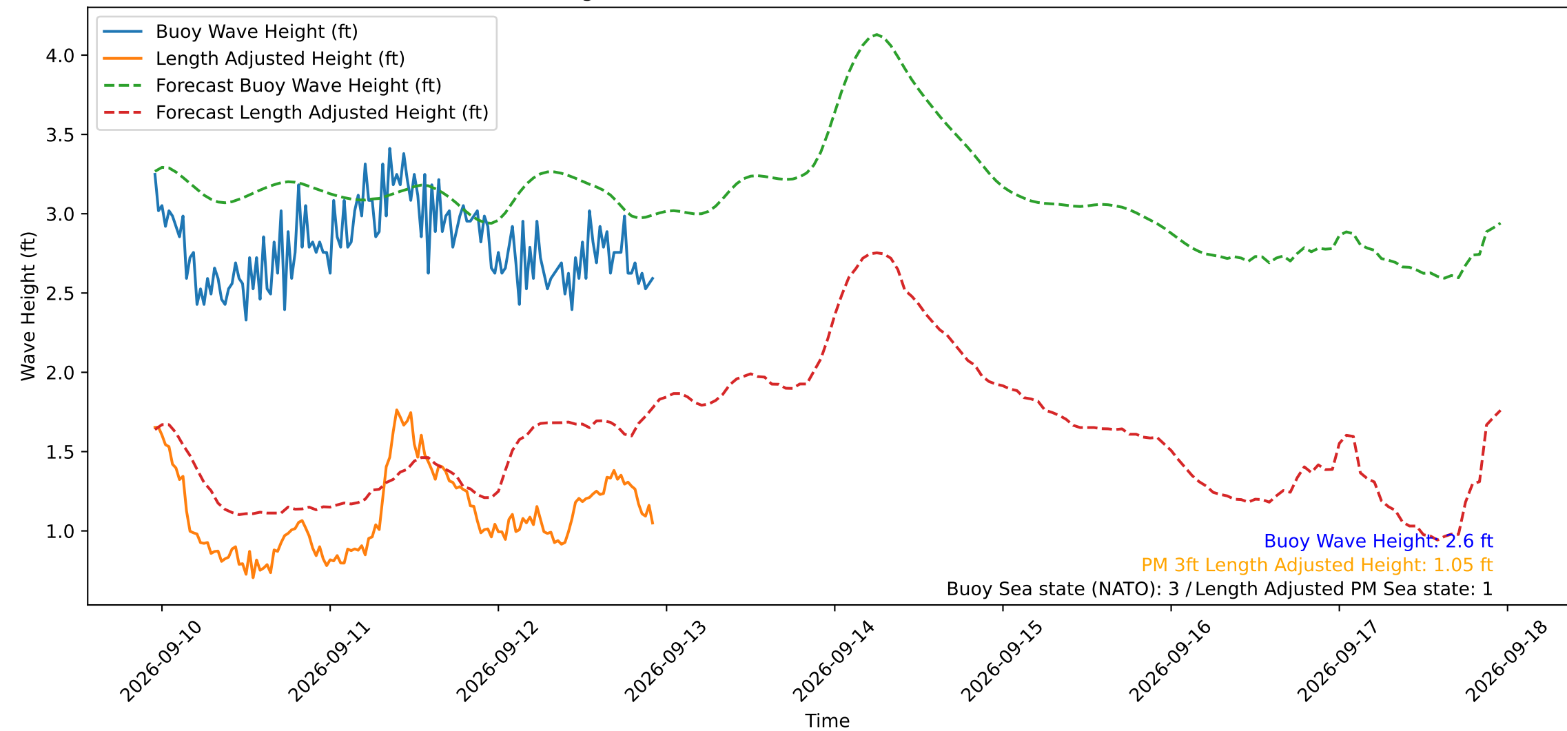
Wave Heights over Time for Red Beach at 2026-09-12 22:40:49
