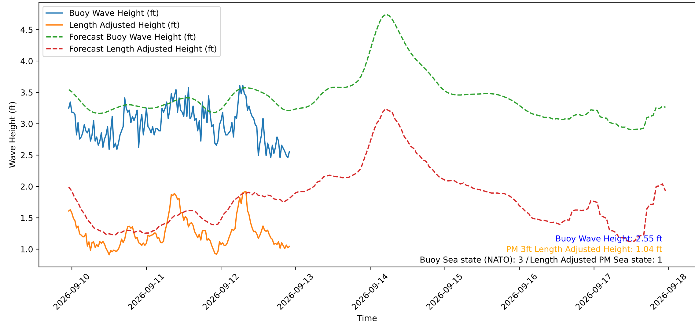
Wave Heights over Time for Green Beach at 2026-09-12 22:41:11
