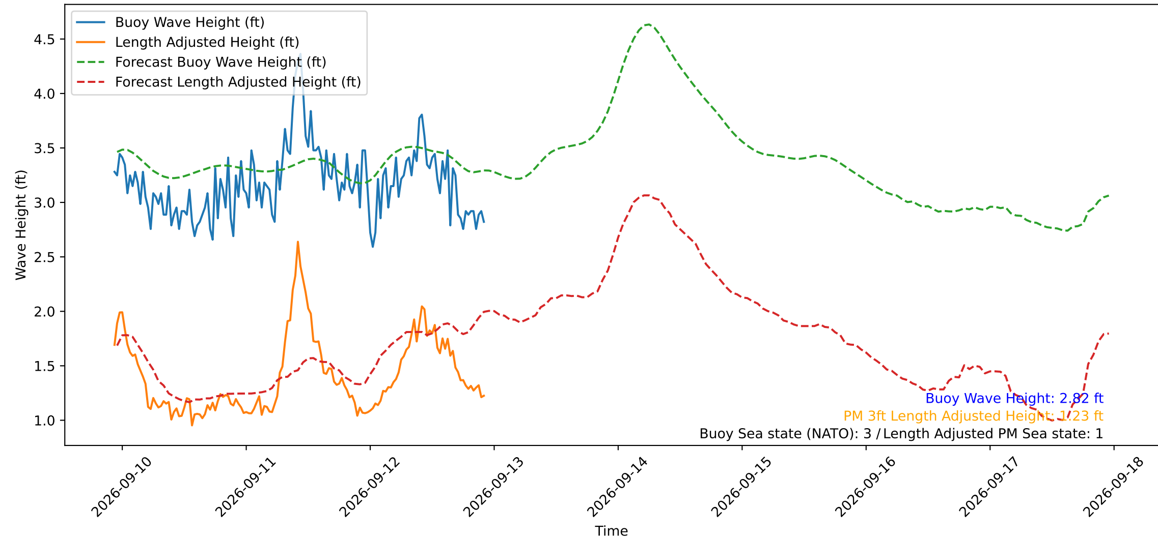
Wave Heights over Time for Oceanside Harbor at 2026-09-12 22:40:29
