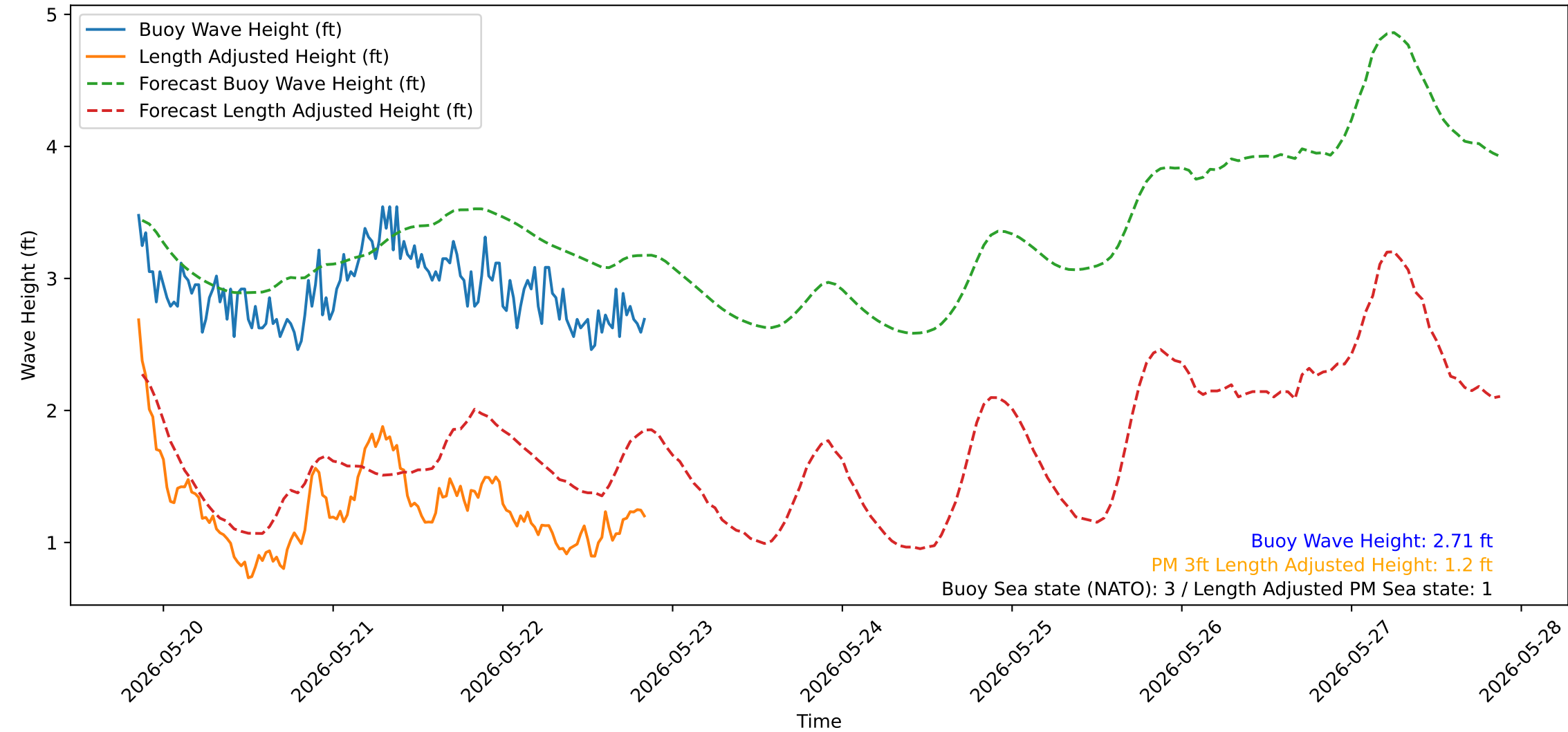
Wave Heights over Time for Green Beach at 2026-05-22 20:41:14
