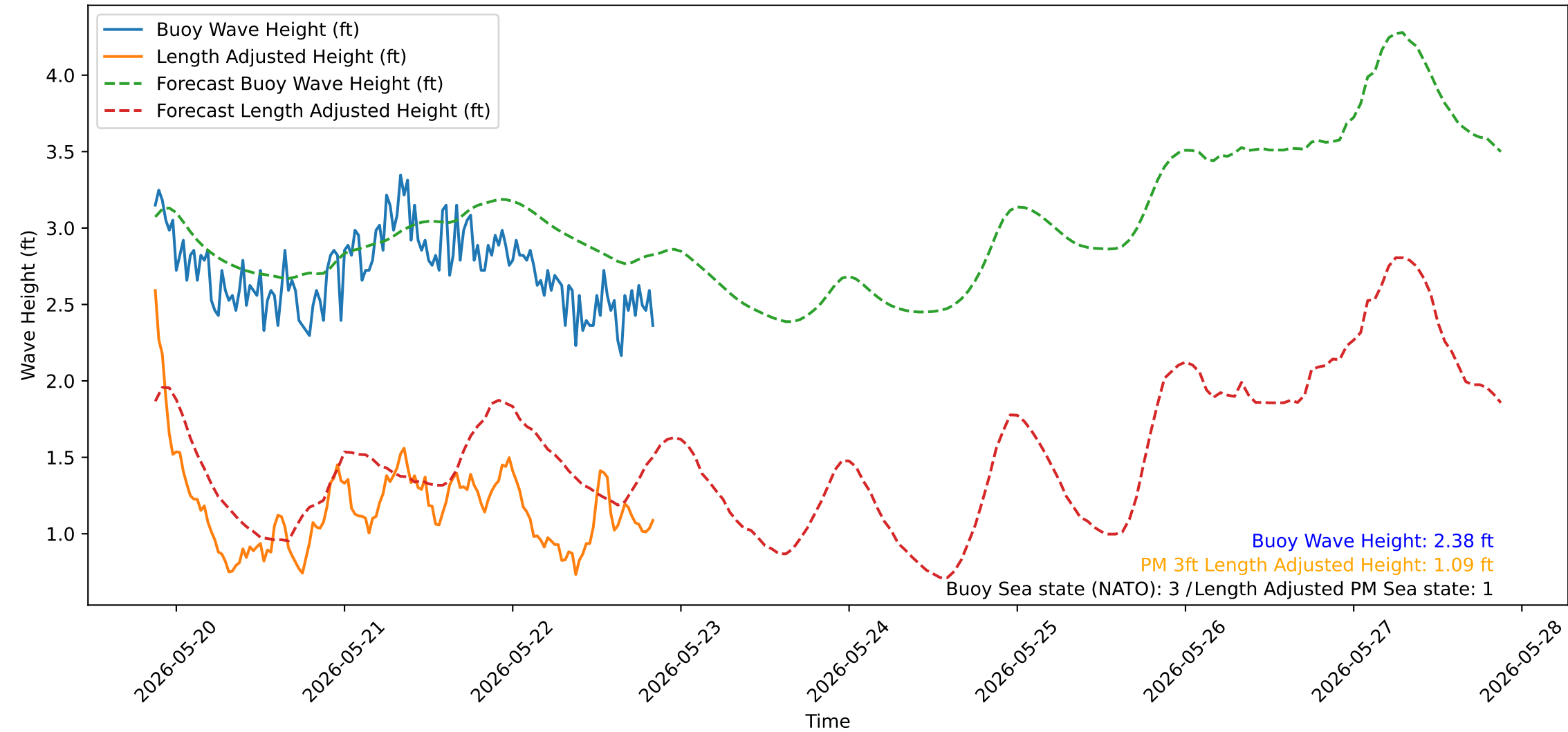
Wave Heights over Time for Red Beach at 2026-05-22 20:40:51
