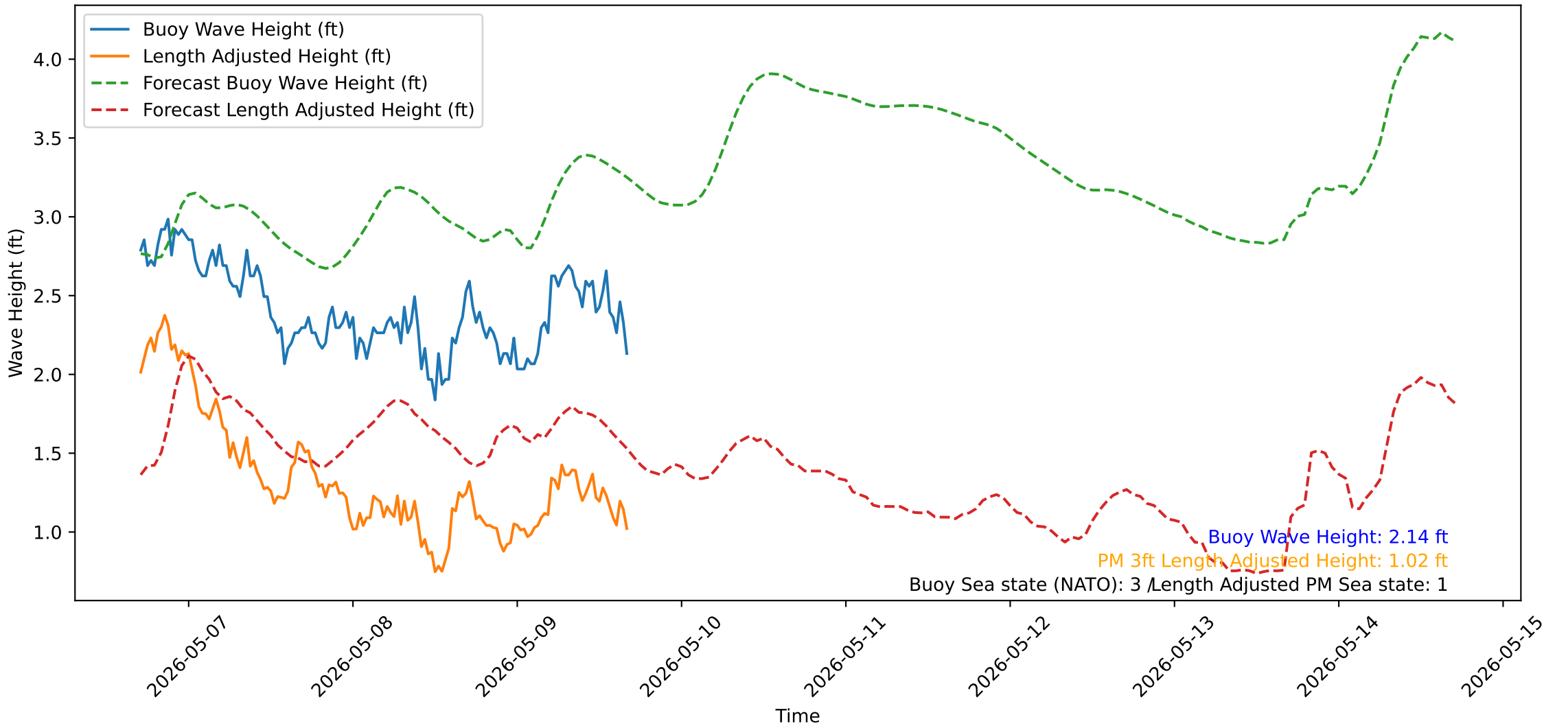
Wave Heights over Time for Green Beach at 2026-05-09 16:51:15
