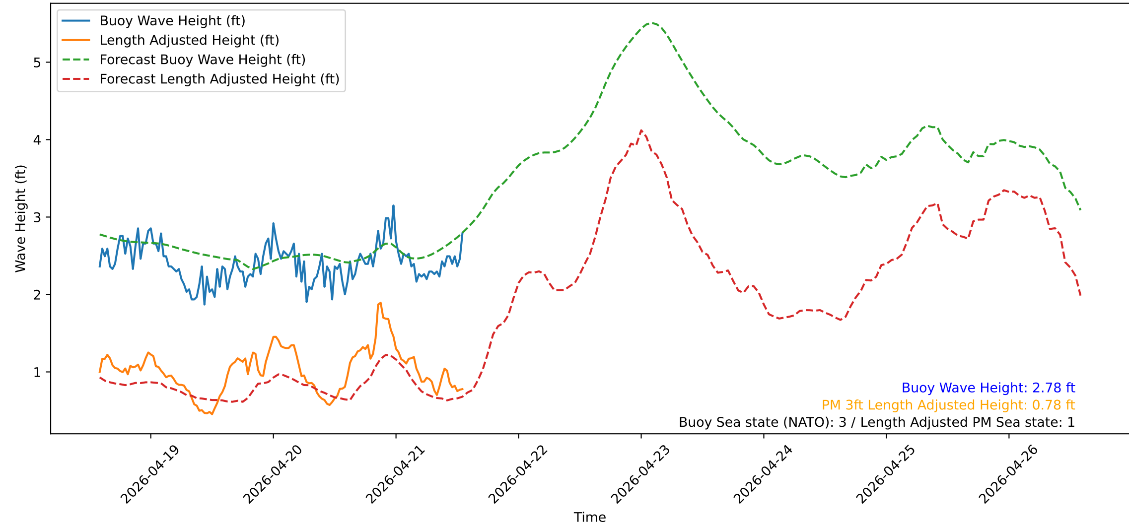
Wave Heights over Time for Green Beach at 2026-04-21 13:51:16
