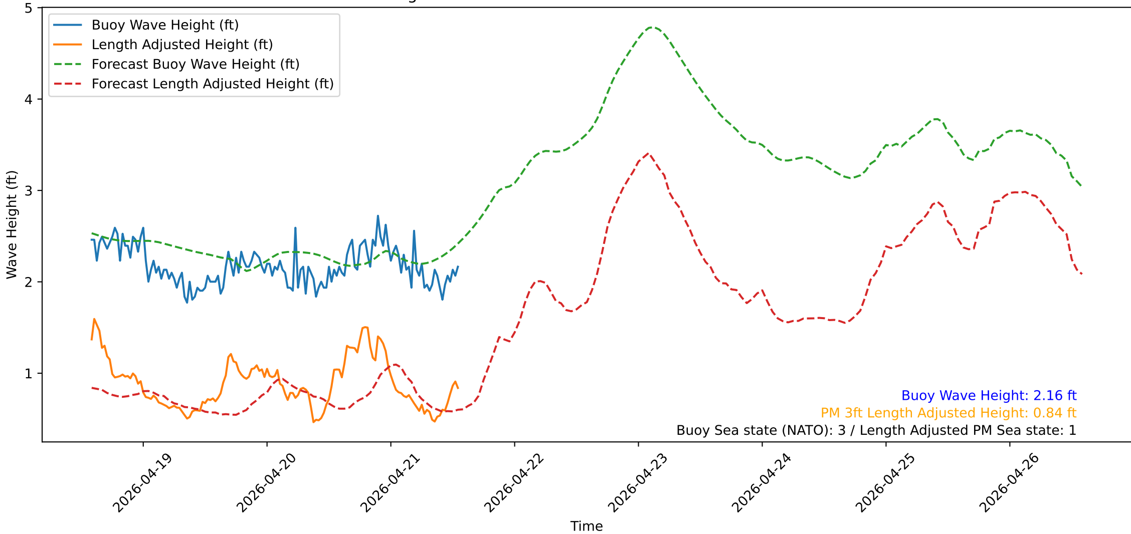
Wave Heights over Time for Red Beach at 2026-04-21 13:50:54
