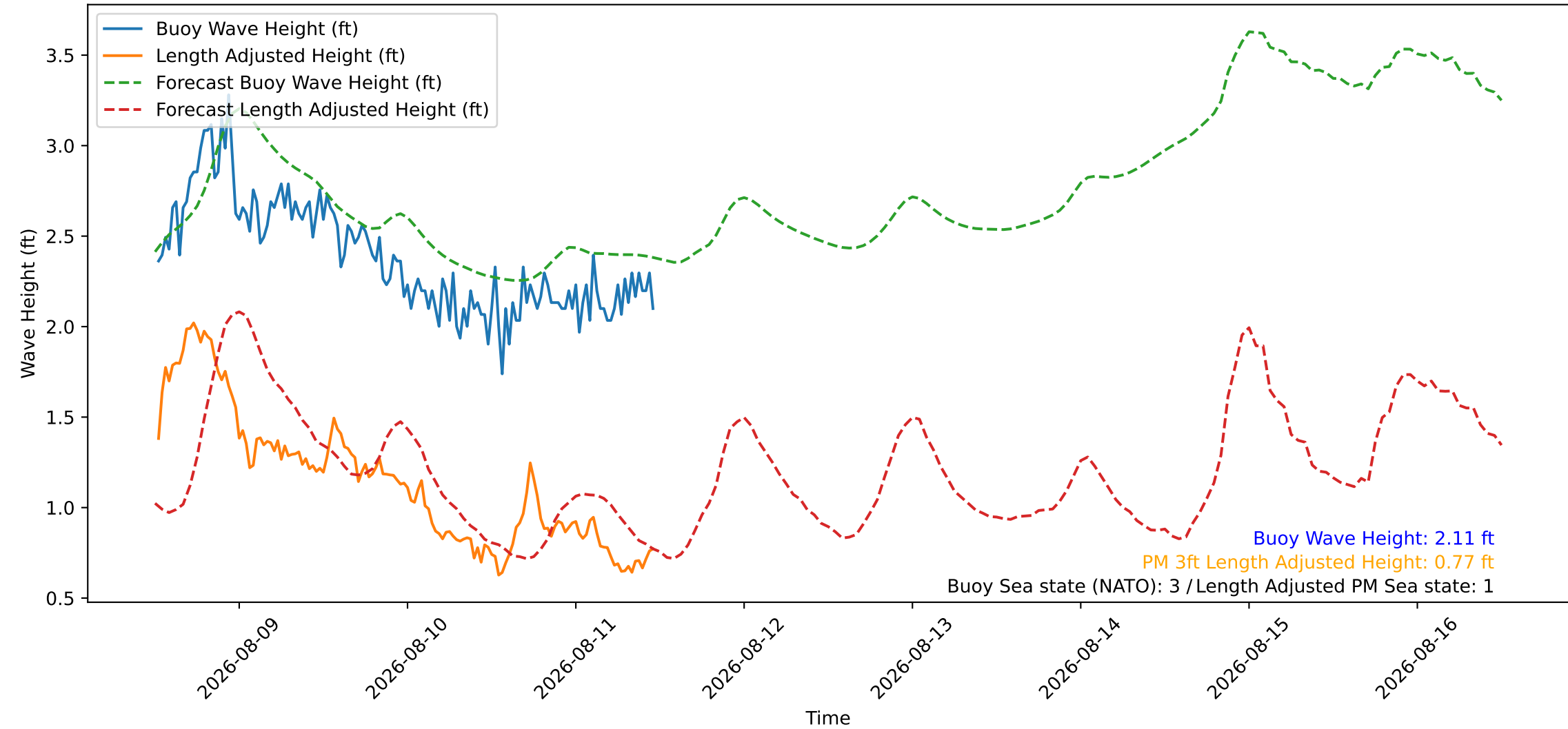
Wave Heights over Time for Red Beach at 2026-08-11 12:10:46
