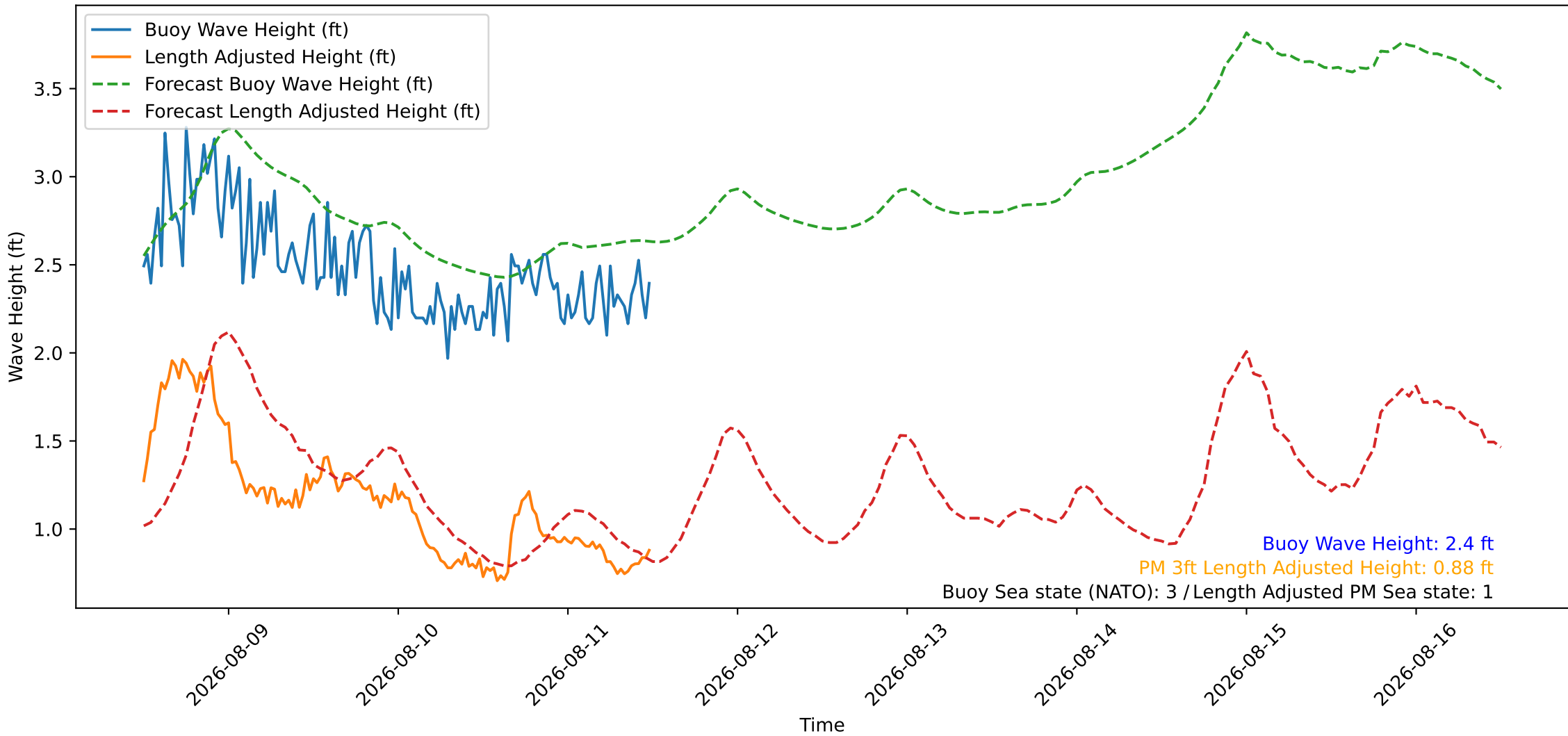
Wave Heights over Time for Oceanside Harbor at 2026-08-11 12:10:26
