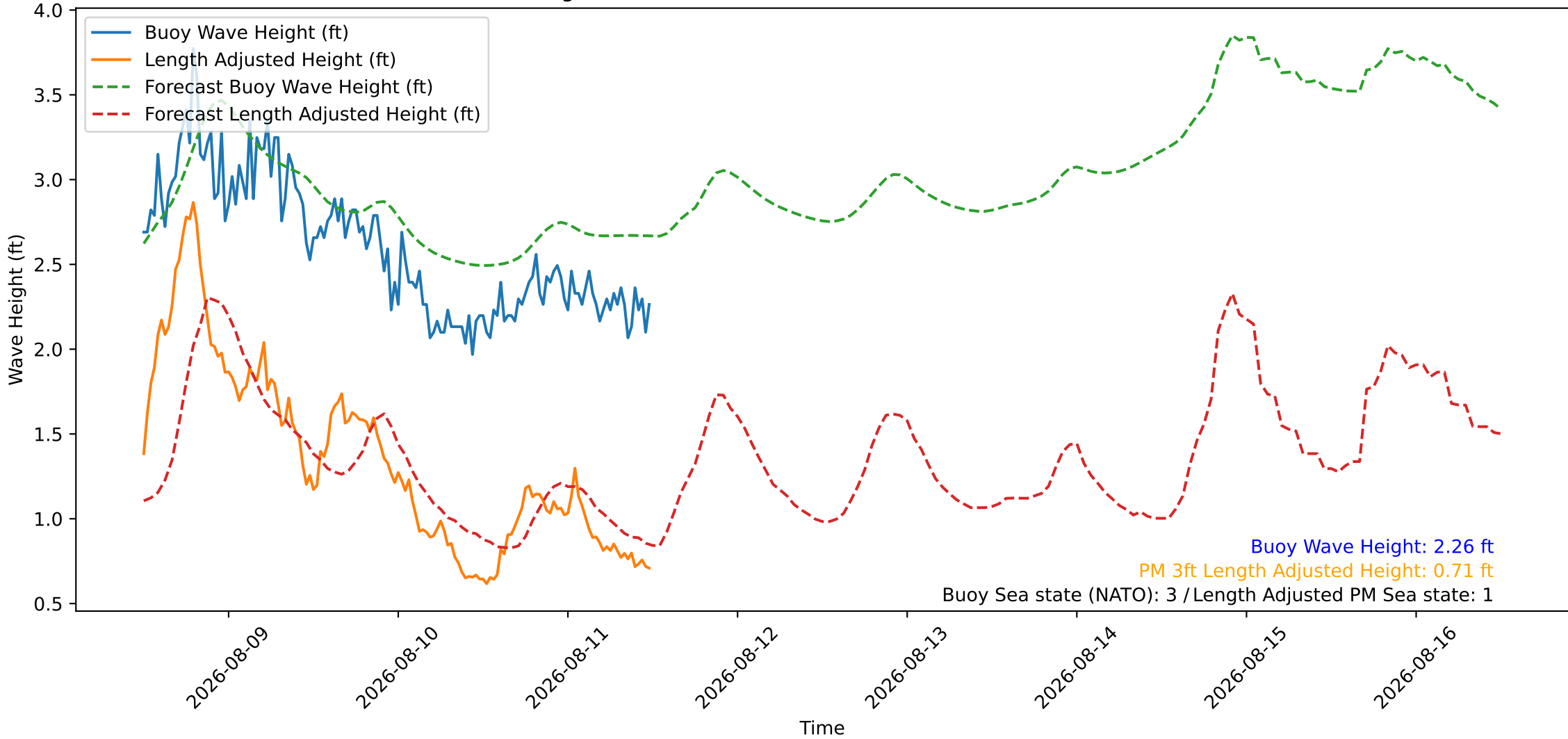
Wave Heights over Time for Green Beach at 2026-08-11 12:11:09
