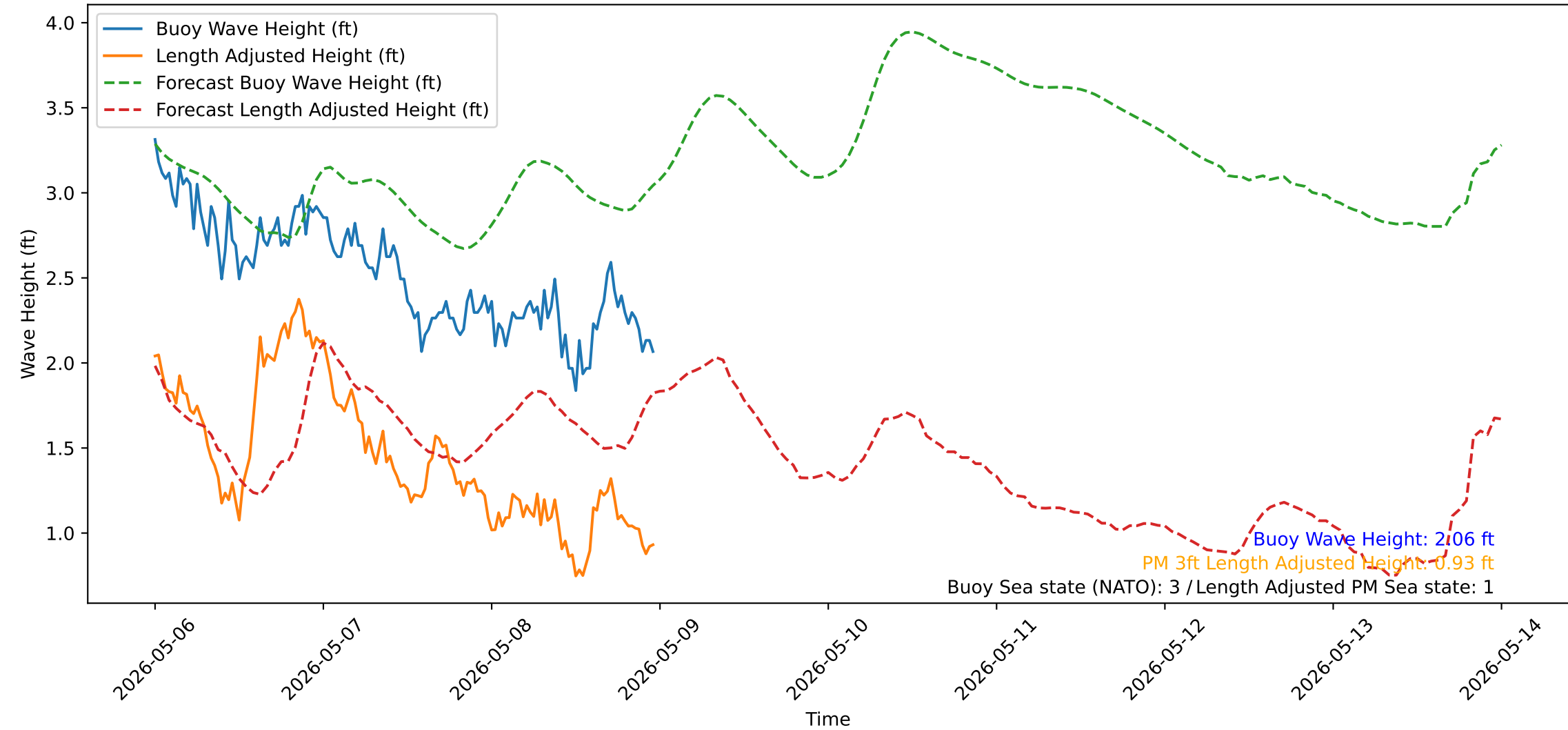
Wave Heights over Time for Green Beach at 2026-05-09 00:01:14
