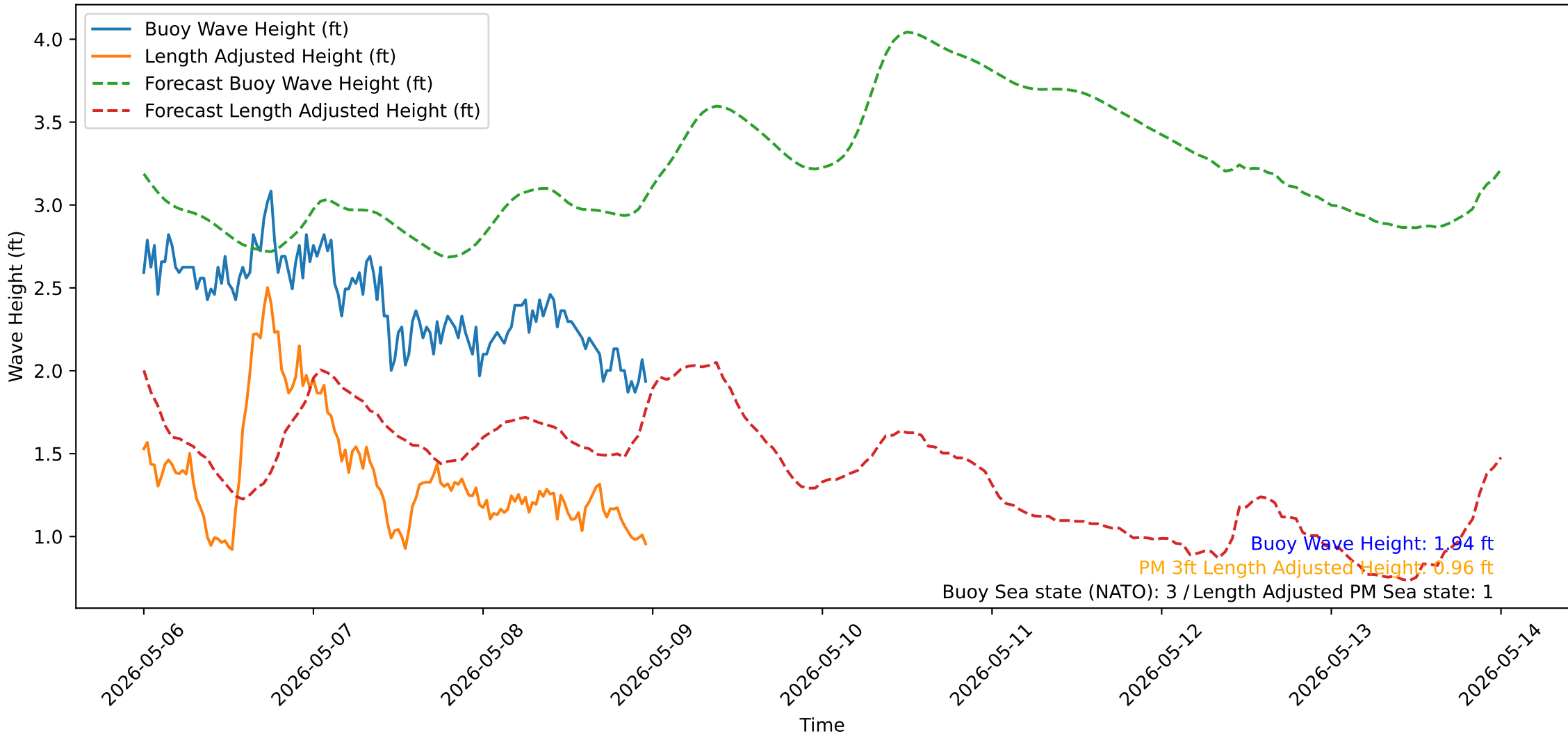
Wave Heights over Time for Oceanside Harbor at 2026-05-09 00:00:32
