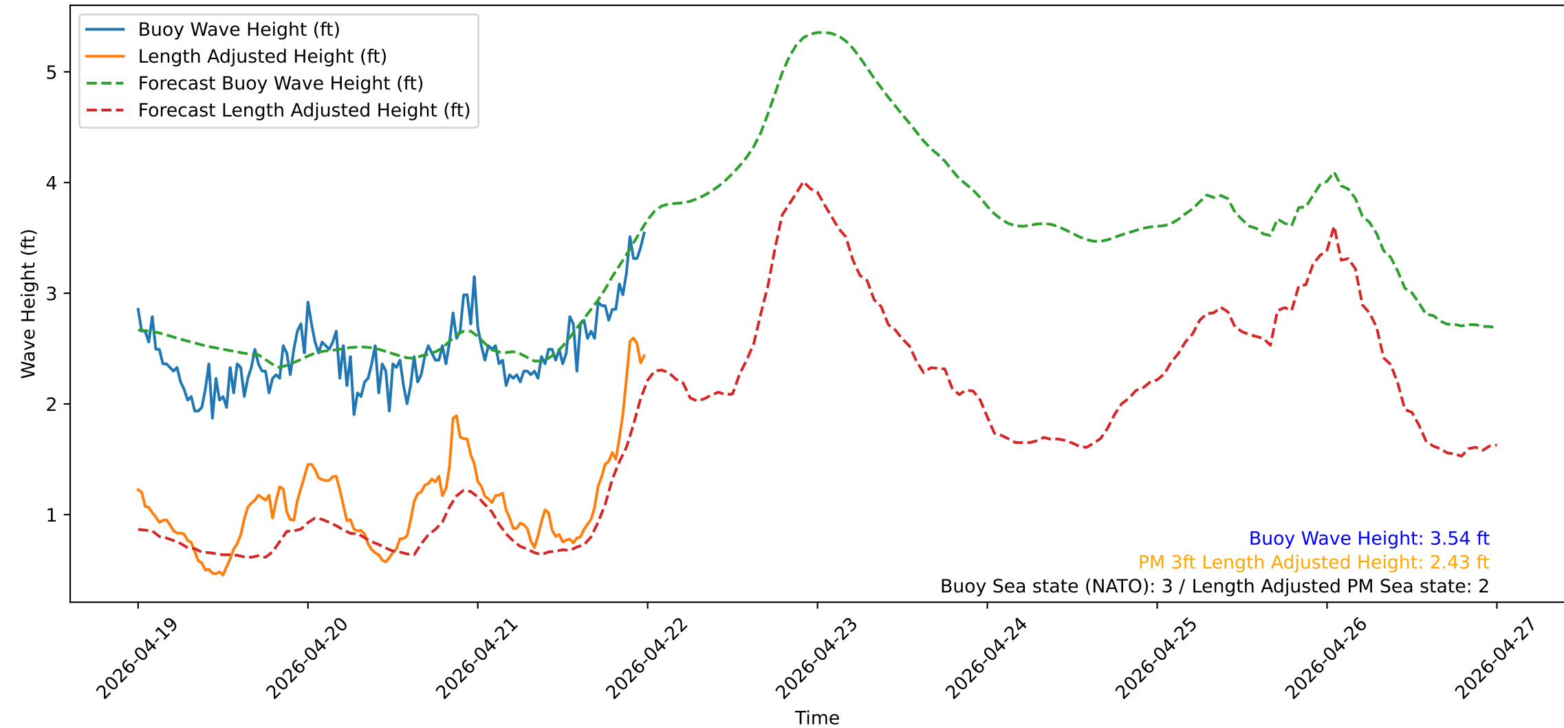
Wave Heights over Time for Green Beach at 2026-04-22 00:11:13
