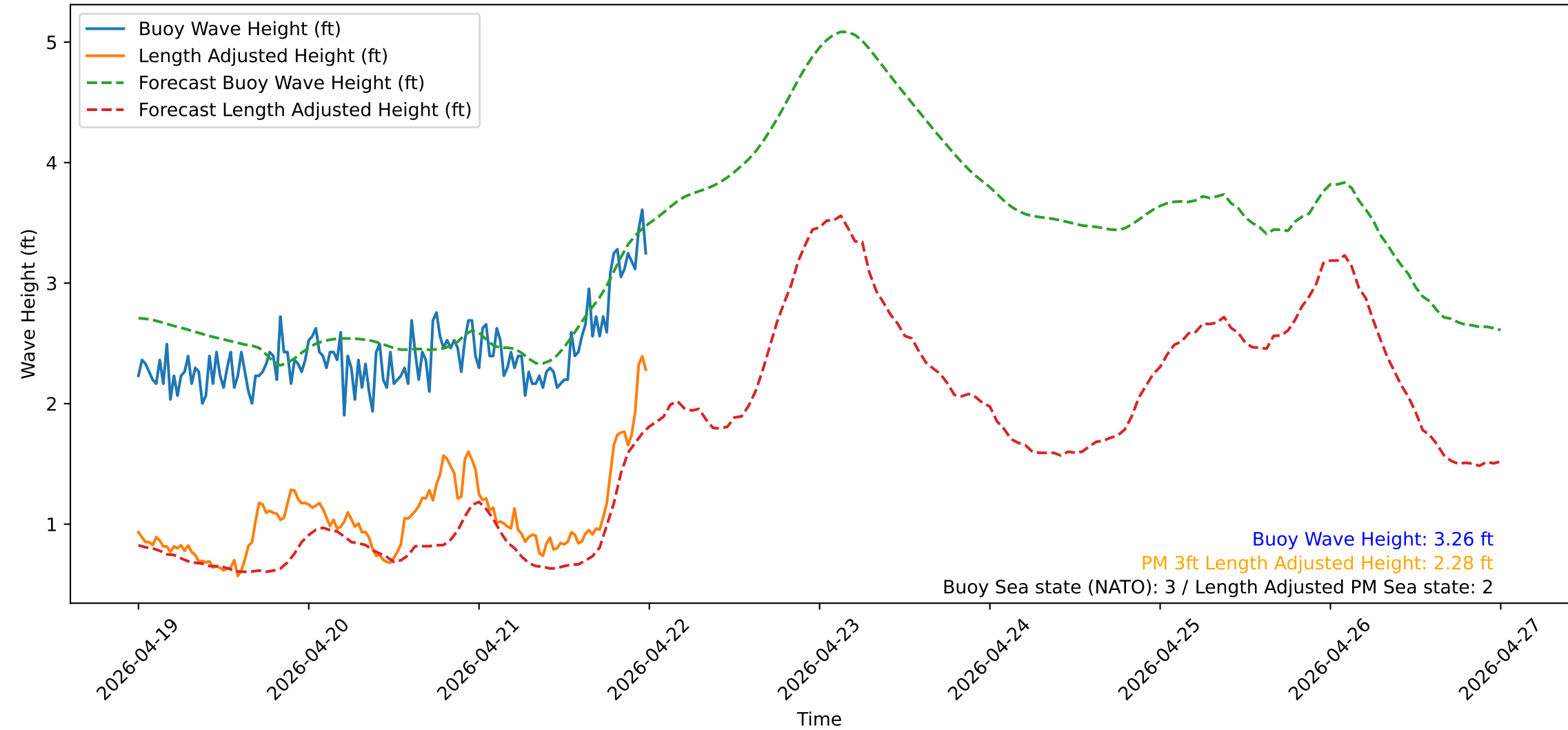
Wave Heights over Time for Oceanside Harbor at 2026-04-22 00:10:31
