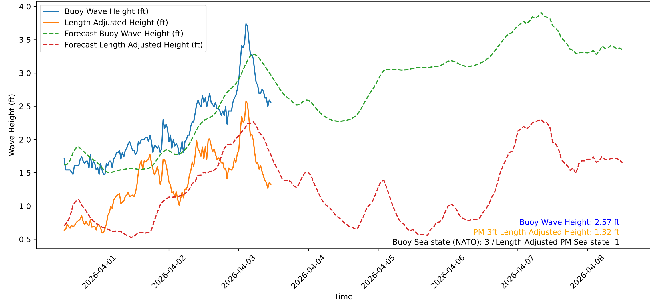
Wave Heights over Time for Red Beach at 2026-04-03 11:50:49
