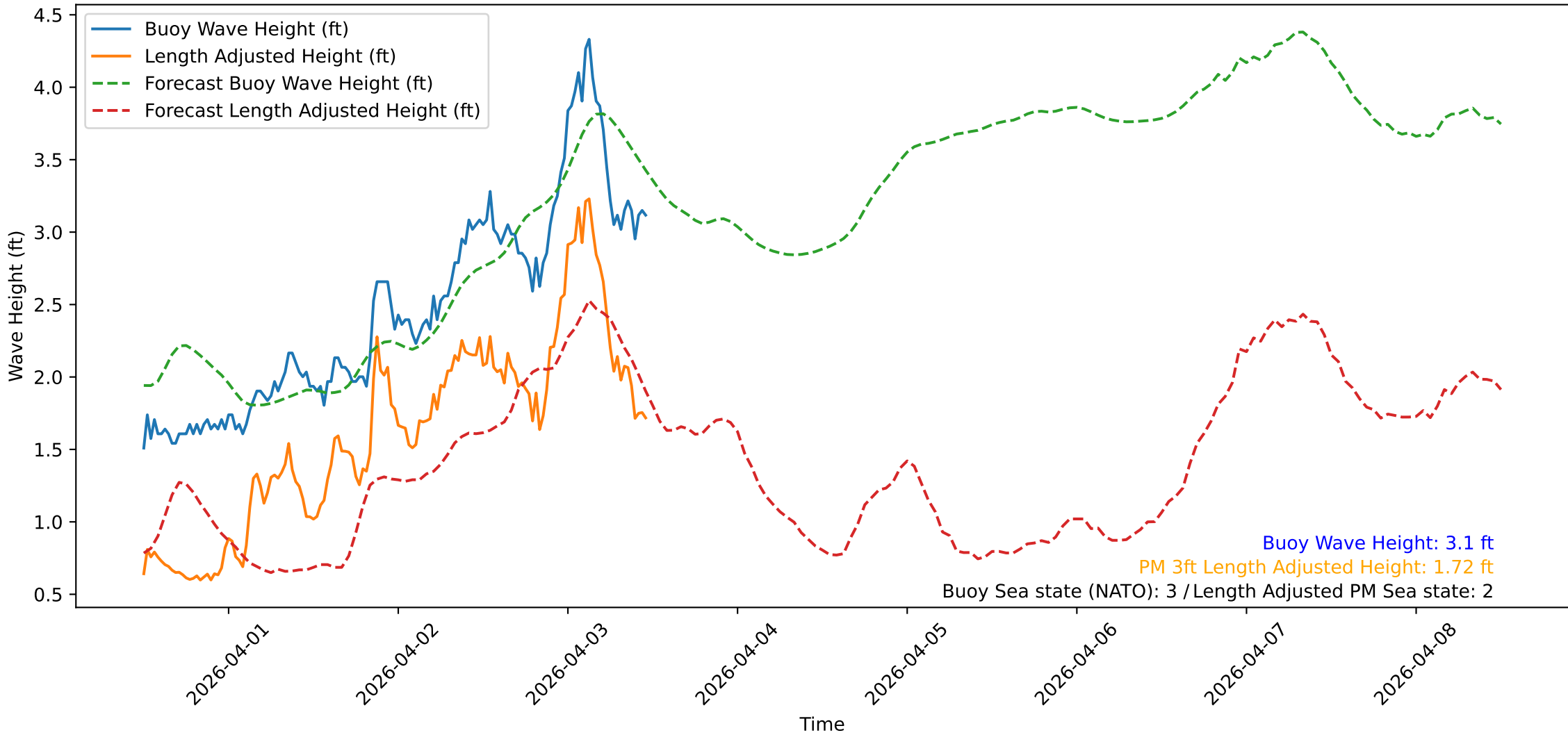
Wave Heights over Time for Green Beach at 2026-04-03 11:51:12
