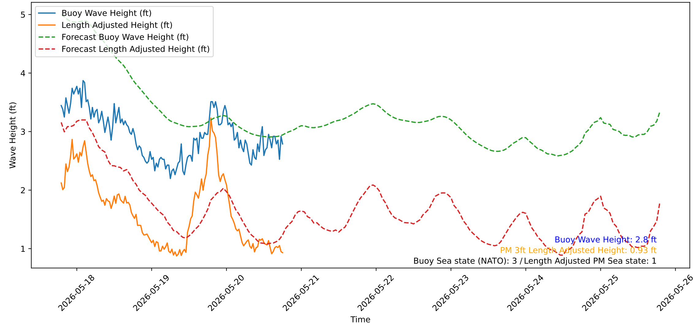
Wave Heights over Time for Oceanside Harbor at 2026-05-20 19:00:32
