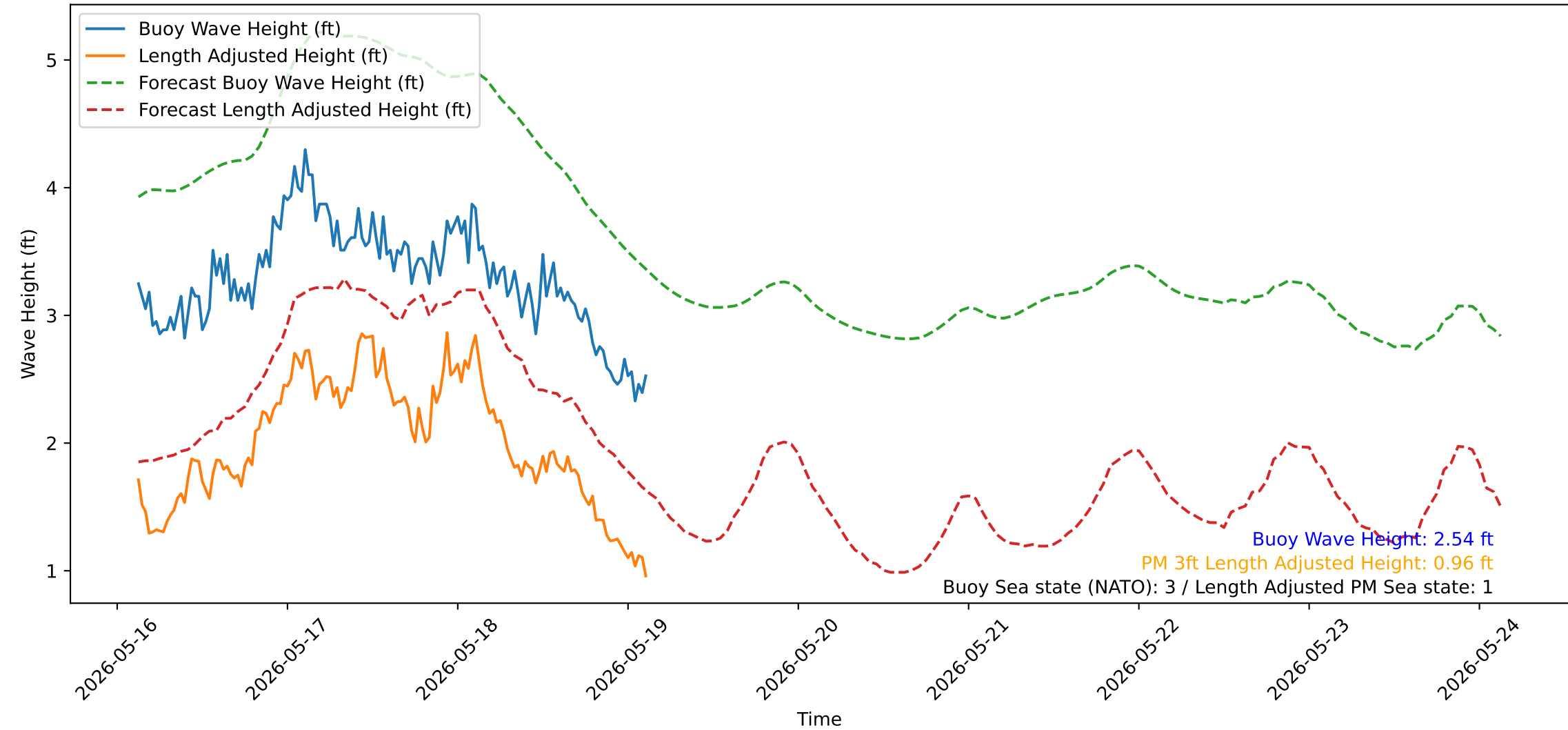
Wave Heights over Time for Oceanside Harbor at 2026-05-19 03:00:32
