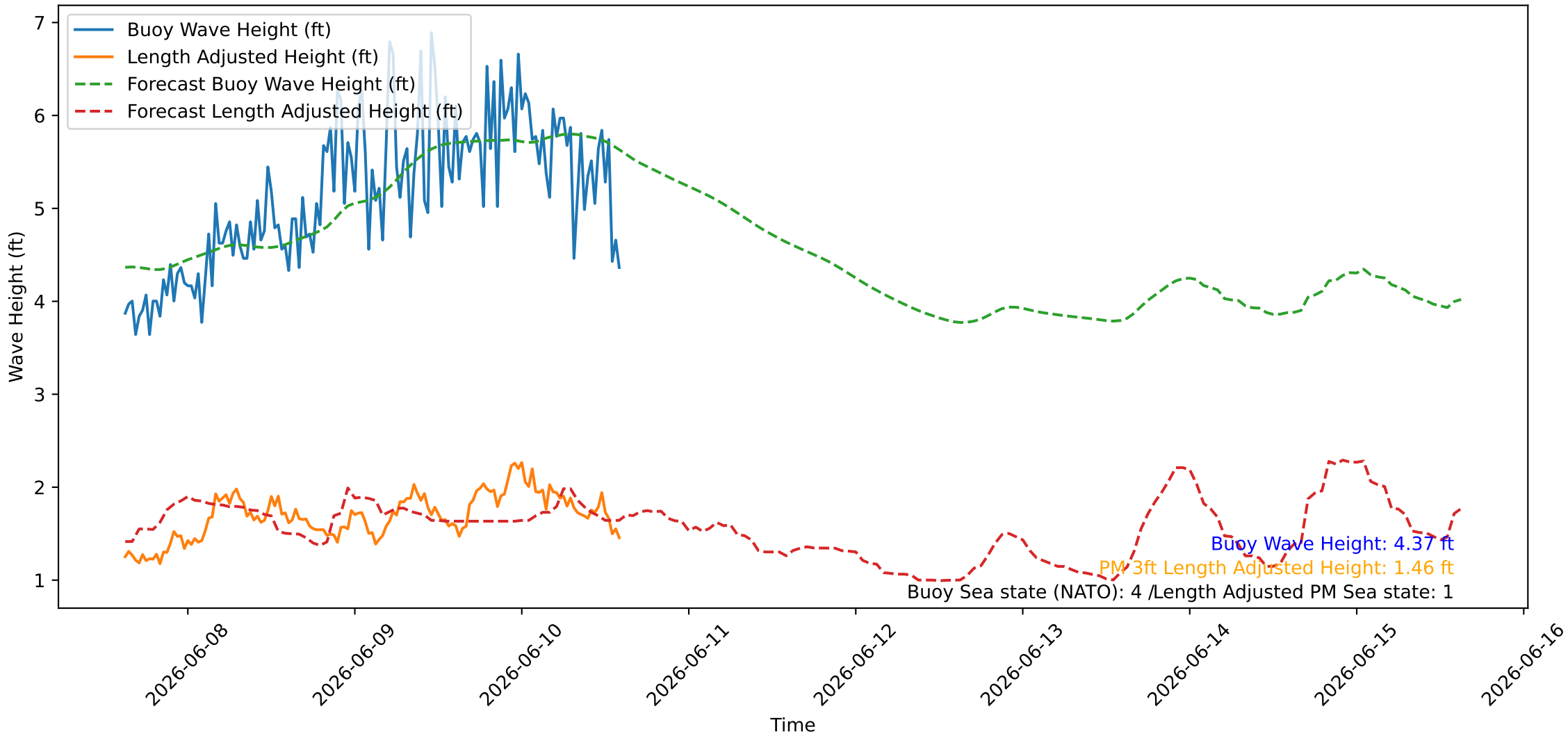
Wave Heights over Time for Green Beach at 2026-06-10 15:01:10
