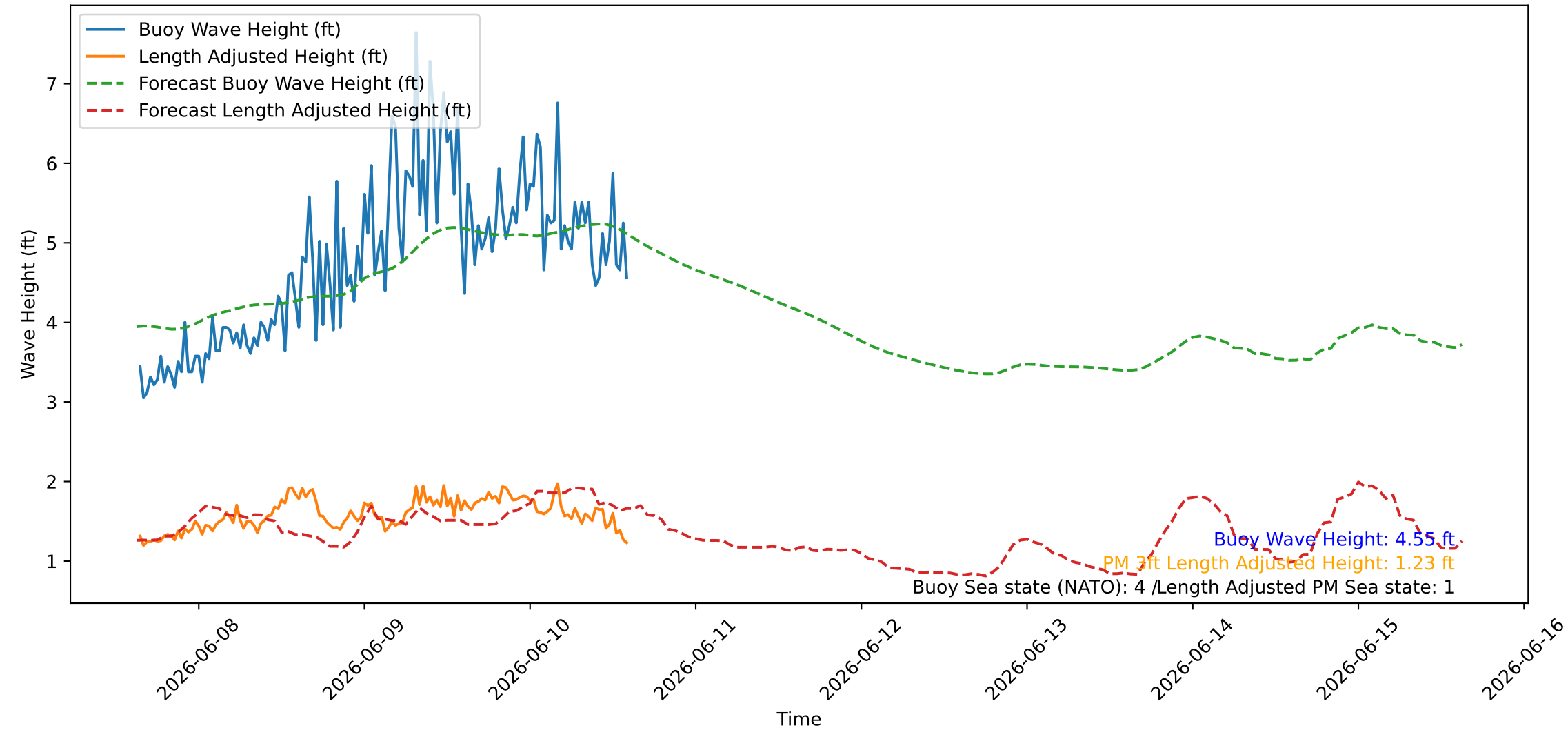
Wave Heights over Time for Red Beach at 2026-06-10 15:00:46
