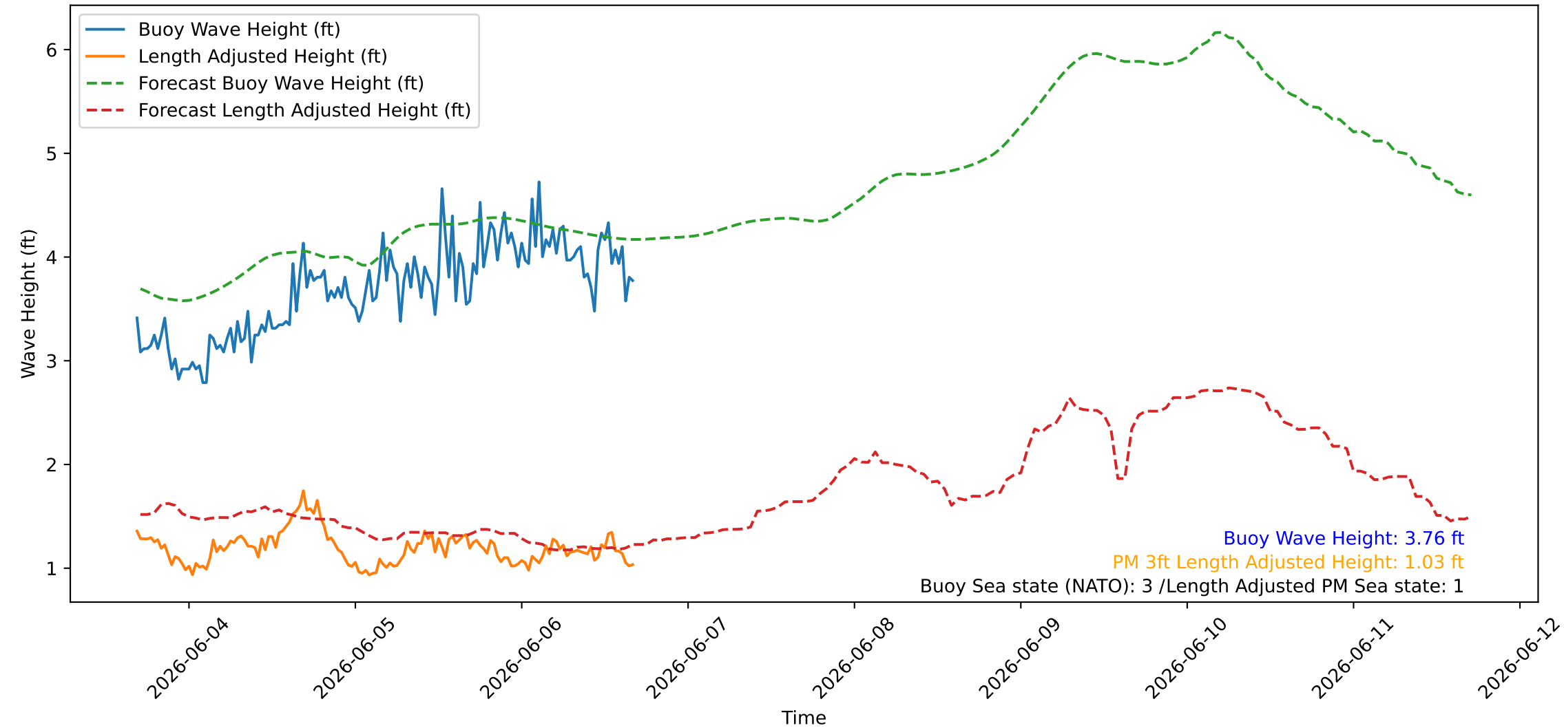
Wave Heights over Time for Green Beach at 2026-06-06 16:41:07
