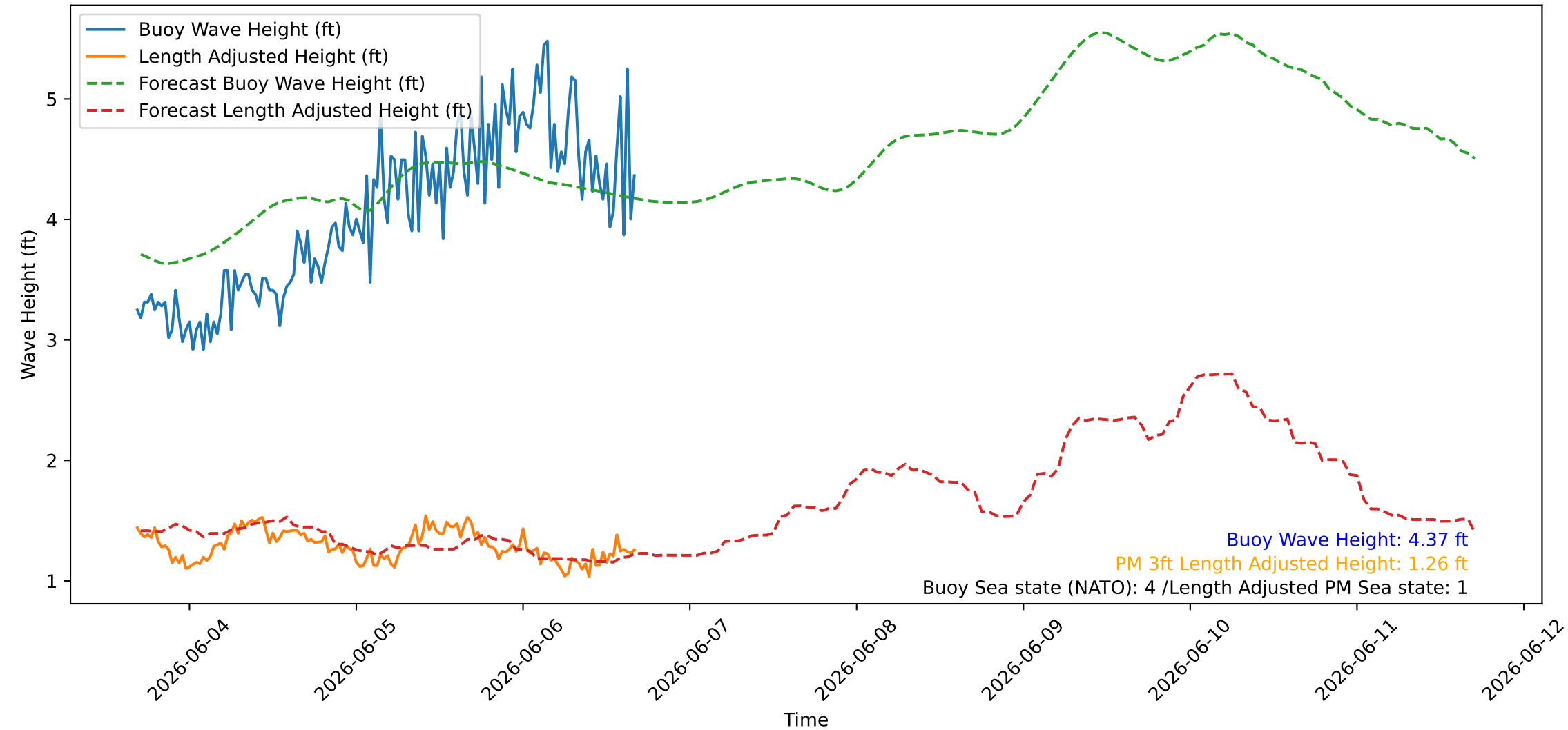
Wave Heights over Time for Oceanside Harbor at 2026-06-06 16:40:25
