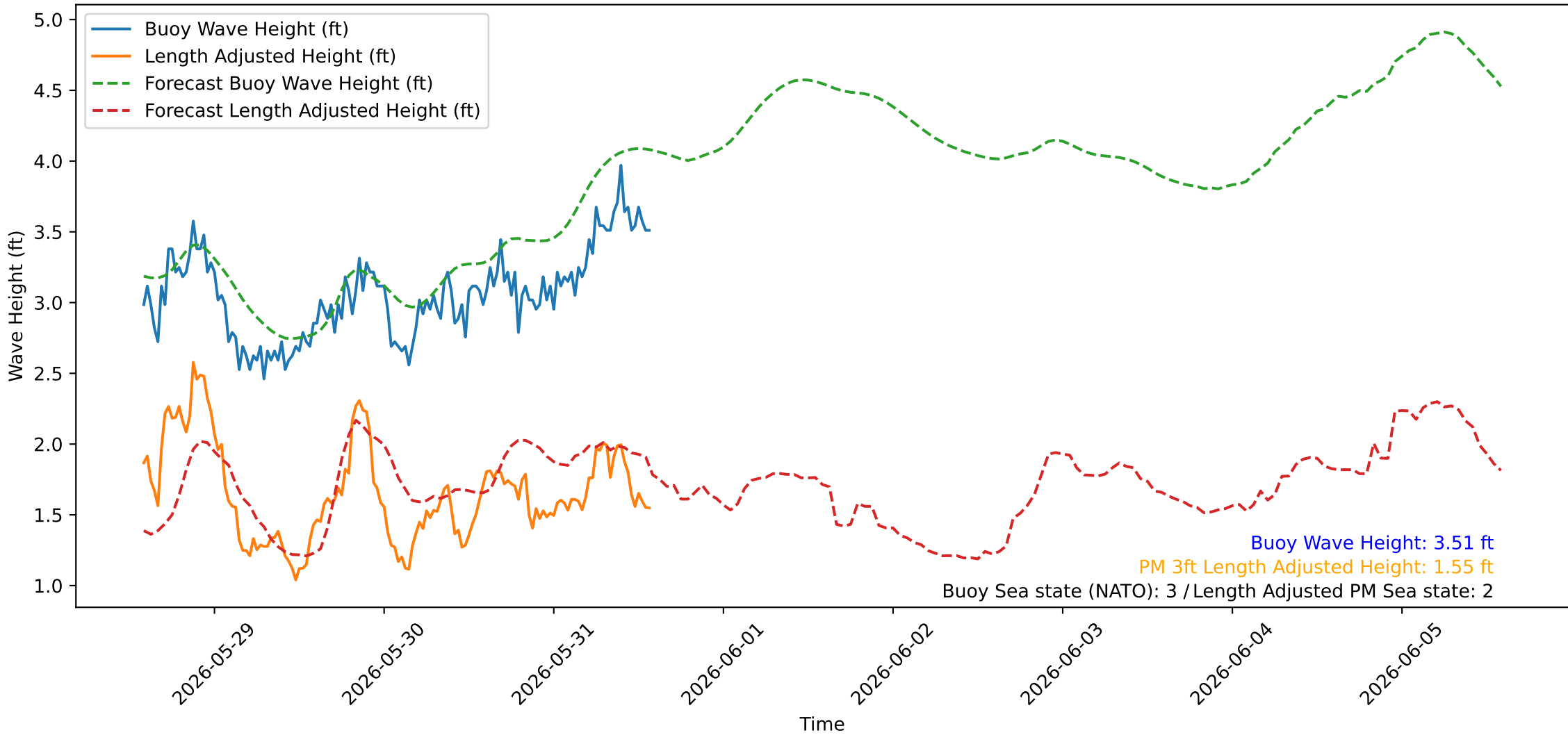
Wave Heights over Time for Green Beach at 2026-05-31 14:11:07
