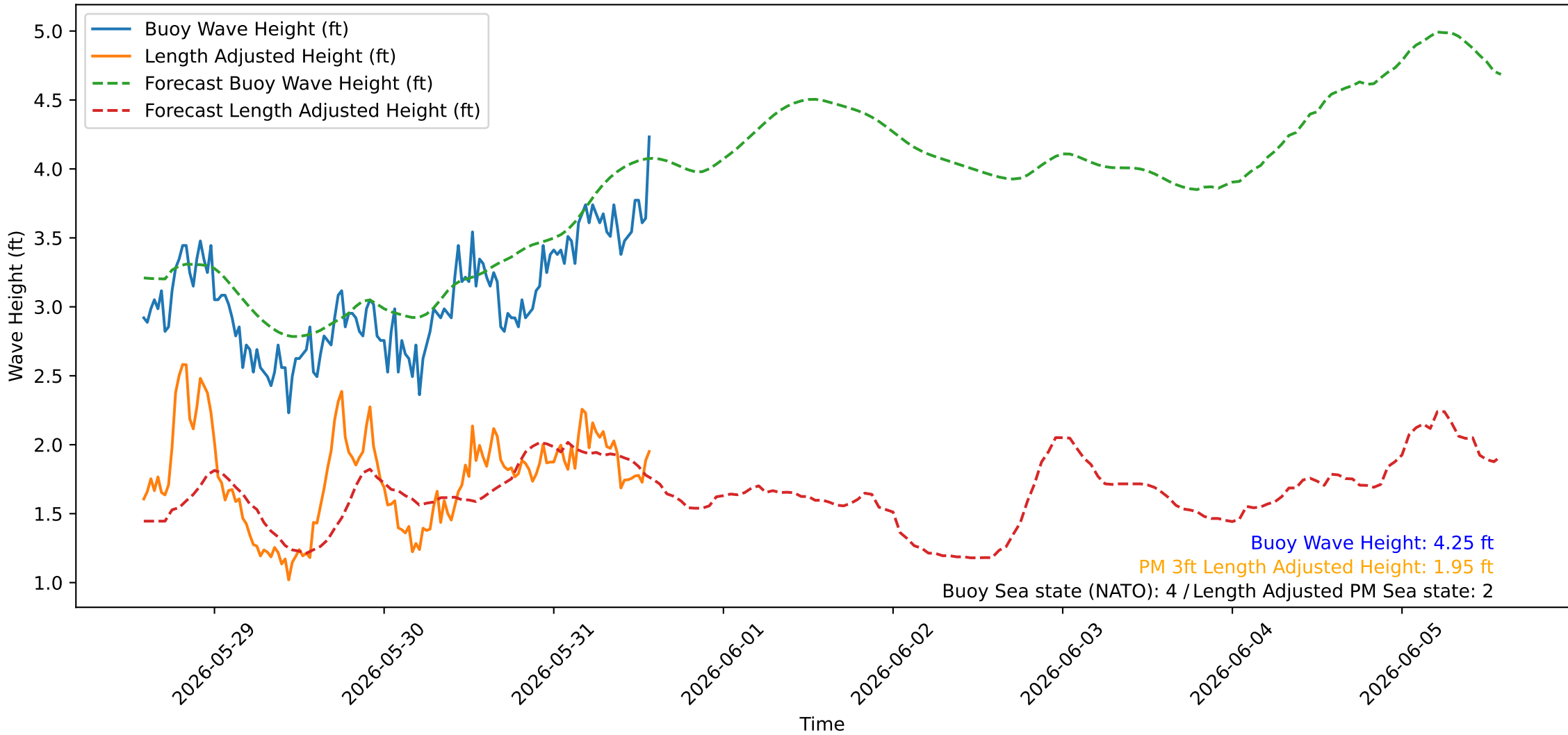
Wave Heights over Time for Oceanside Harbor at 2026-05-31 14:10:26
